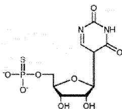
5'-O-(1-Thiophosphate)-Pseudouridine
