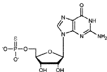
5'-O-(1-Thiophosphate)-Guanosine
