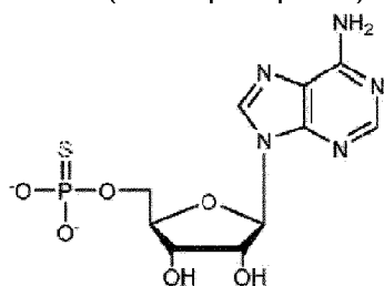
5'-O-(1-Thiophosphate)-Adenosine
