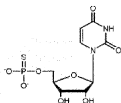
5'-O-(1-Thiophosphate)-Uridine
