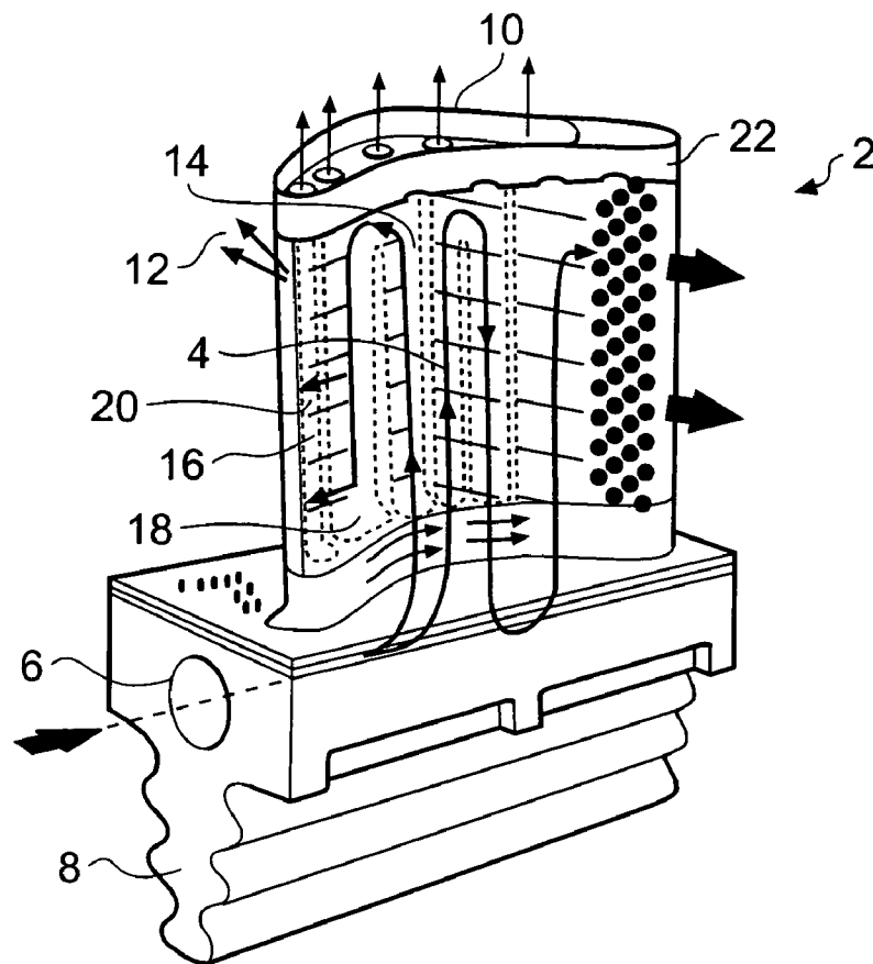
Fig. 1 (Prior Art)
