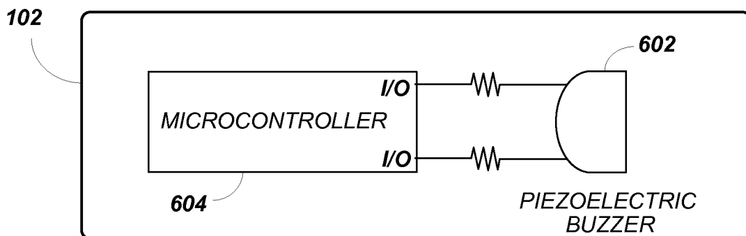
FIG. 6 (PRIOR ART)
