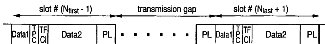
(a) Frame structure type A
