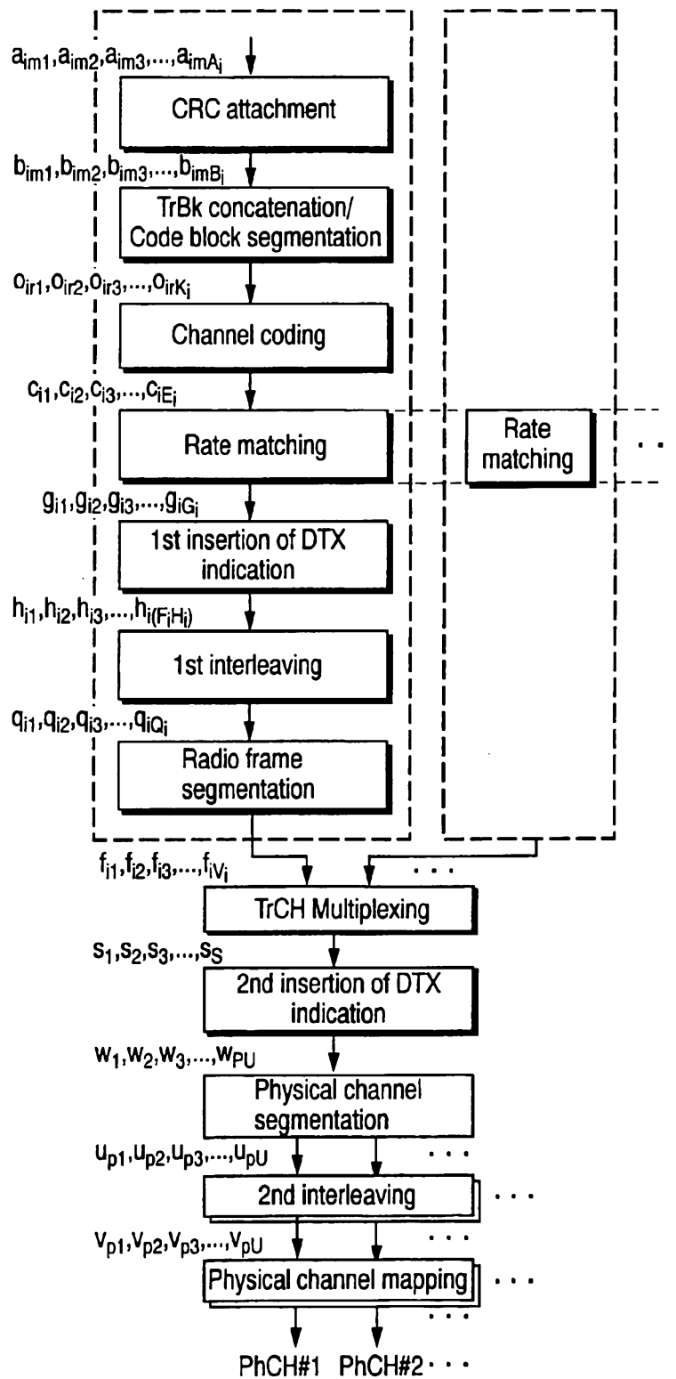
Transport channel multiplexing structure for downlink
