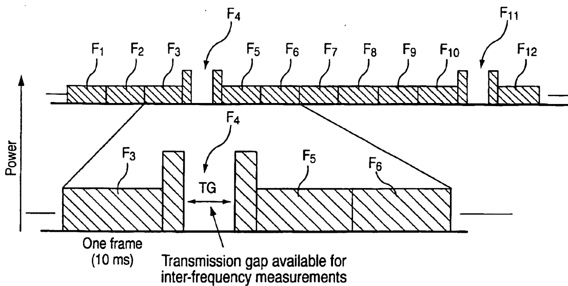
Compressed mode transmission
