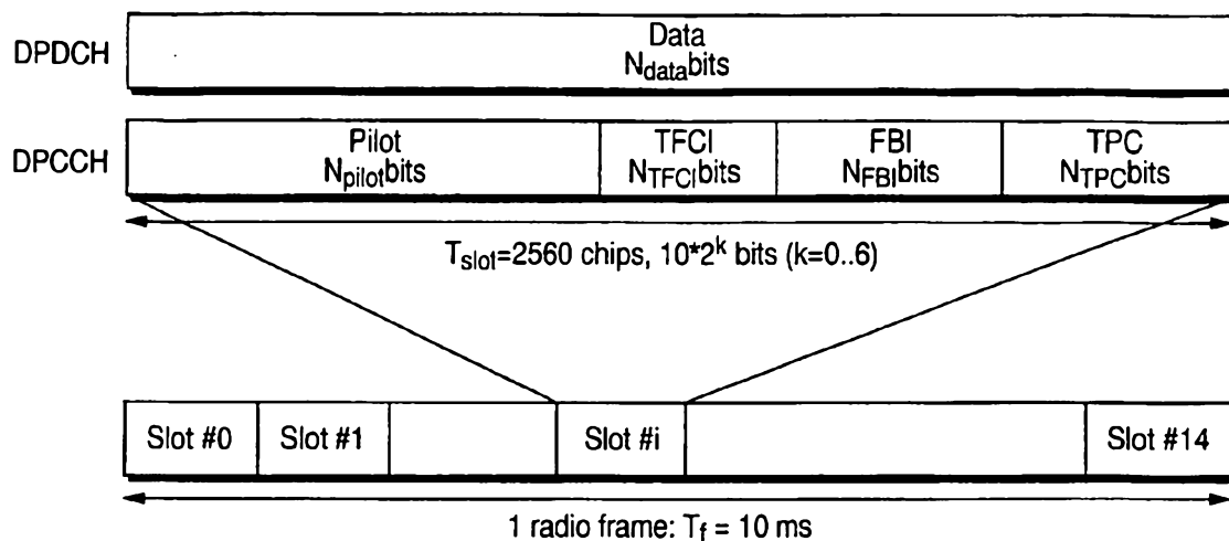
Frame structure for uplink DPDCH/DPCCH
