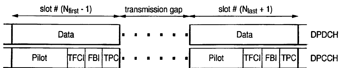
Frame structure in uplink compressed transmission
