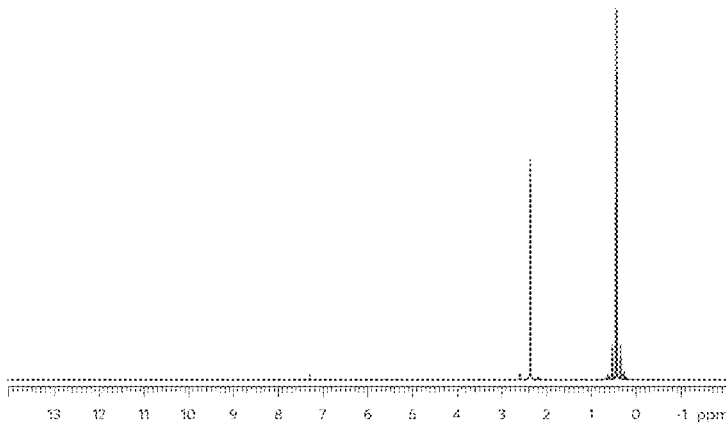
NMR spectrum of Me 3 SnNMe 2
