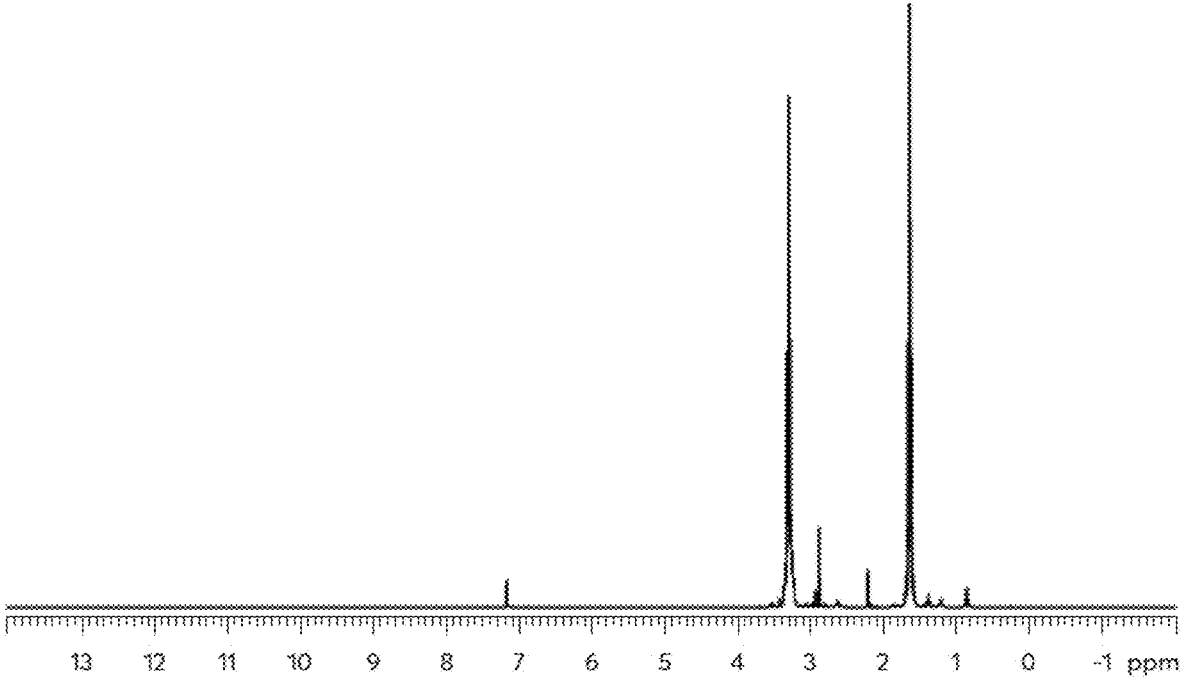
Figure 11: NMR of Sn(Pyrrolodiny)4
