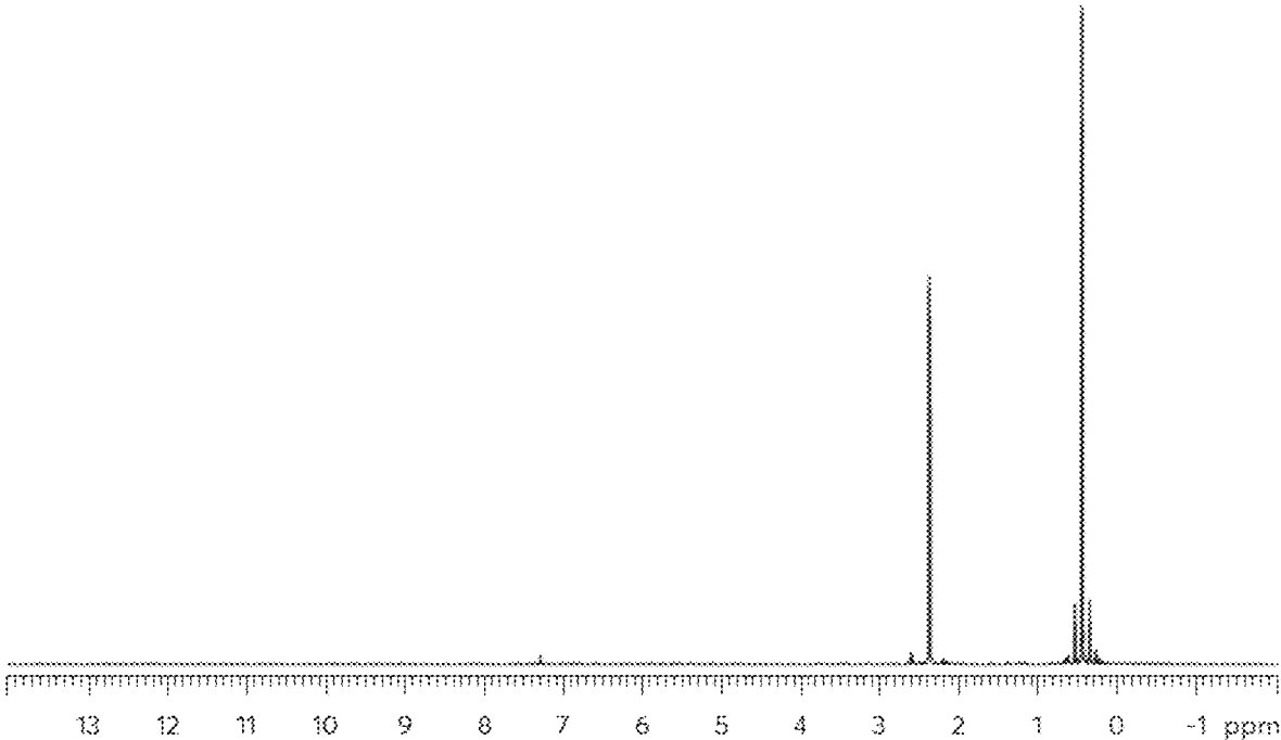
Figure 1: NMR spectrum of Me 3 SnNMe 2
