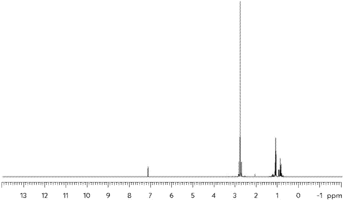
Figure 10: NMR of Me 2 Sn(NEt 2 ) 2
