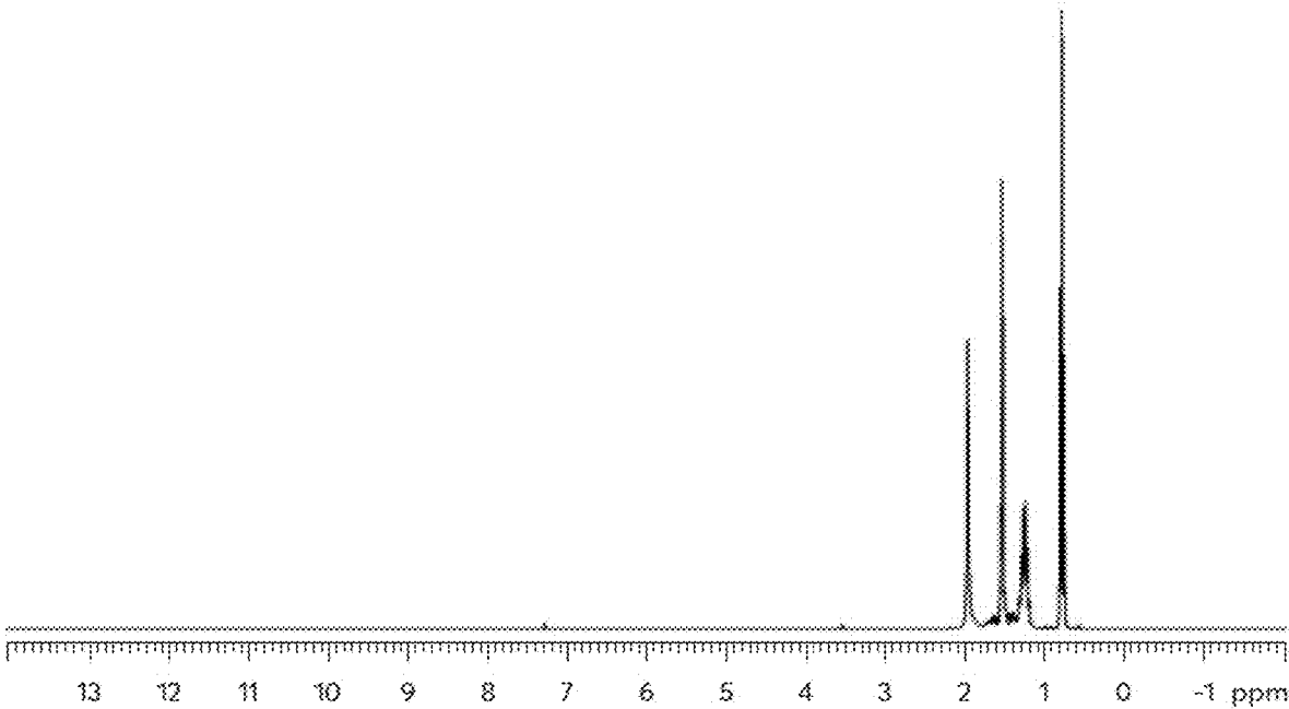
Figure 8: NMR of Bu 2 Sn(OAc) 2
