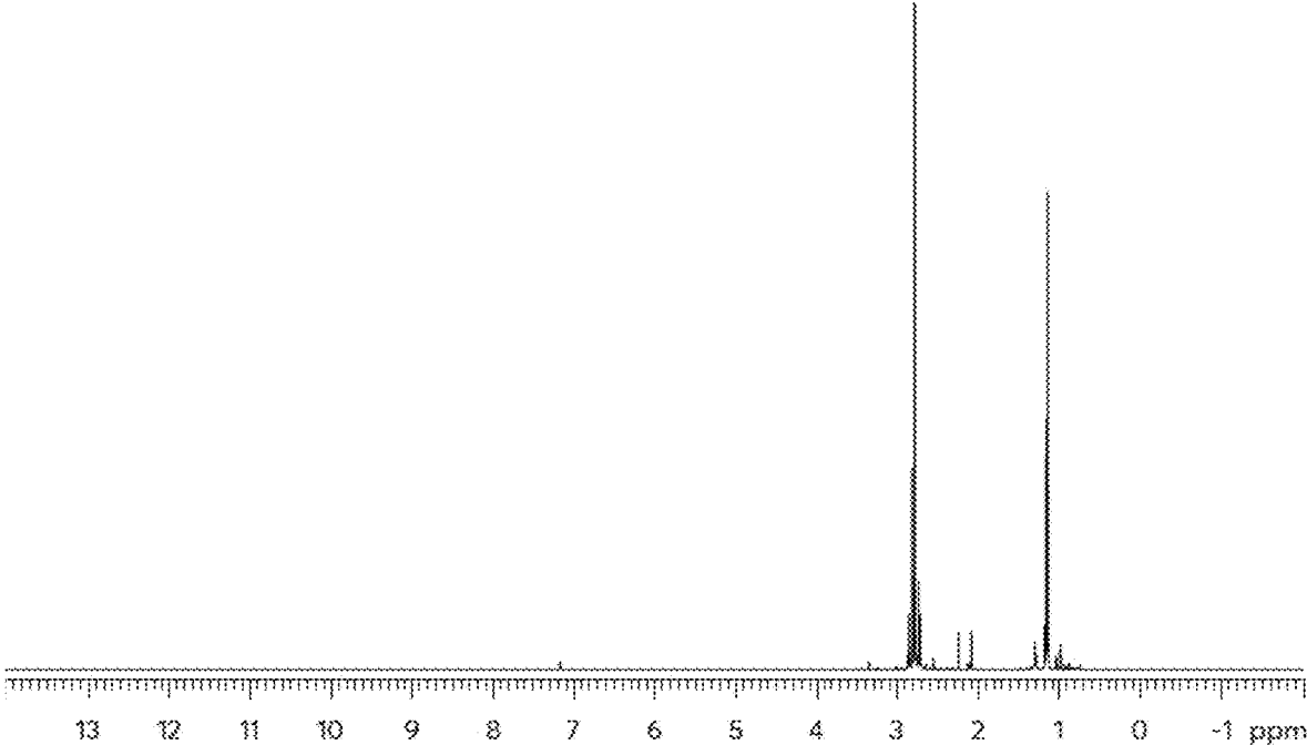
Figure 14: NMR of Me 2 Sn(NMe 2 ) 2
