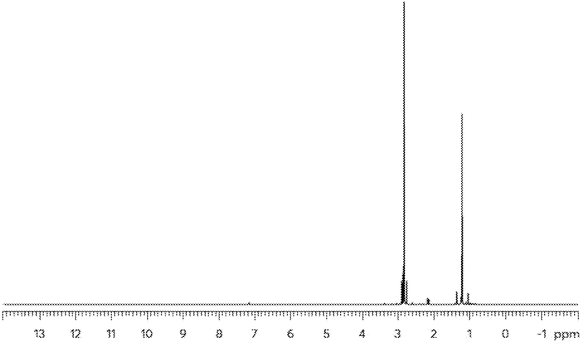
Figure 15: NMR of tBuSn(NMe2)3
