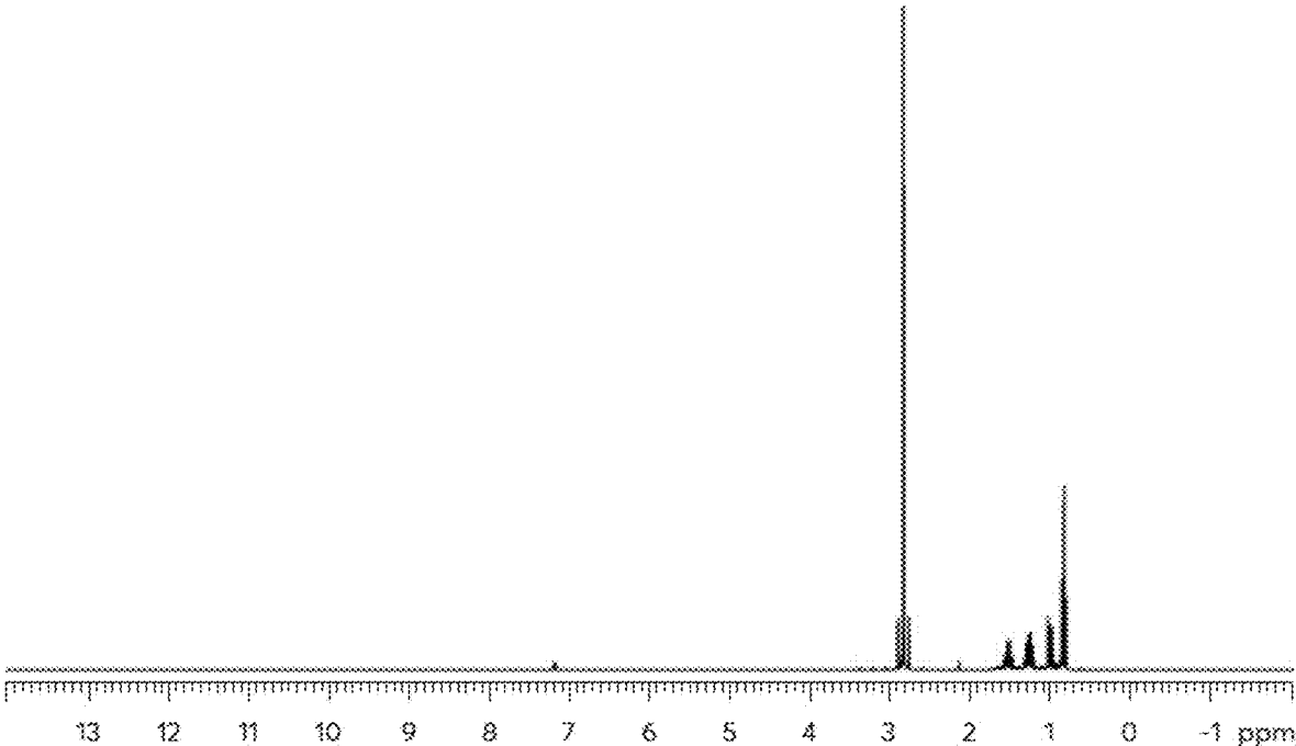
Figure 4: NMR of Bu 2 Sn(NMe 2 ) 2
