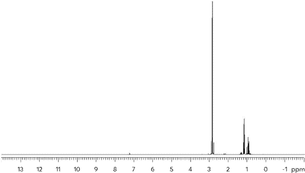
Figure 9: NMR of Et 2 Sn(NMe 2 ) 2
