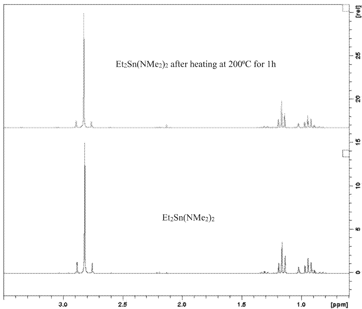
Figure 22. NMR of \text{Et}_2\text{Sn}(\text{NMe}_2)_2 before and after heating at 200^\circ\text{C}
