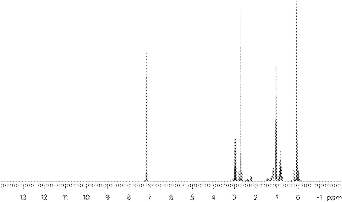
Figure 3: NMR of Me 2 Sn(NEtMe) 2
