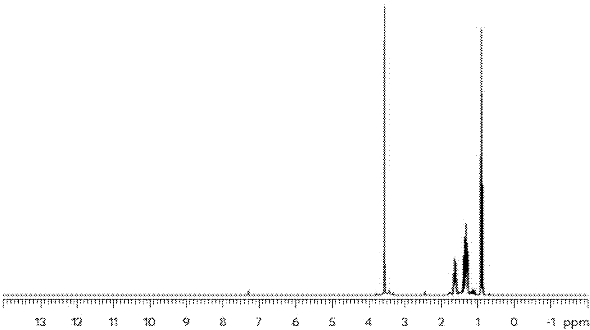
Figure 7: NMR of Bu2Sn(OMe)2
