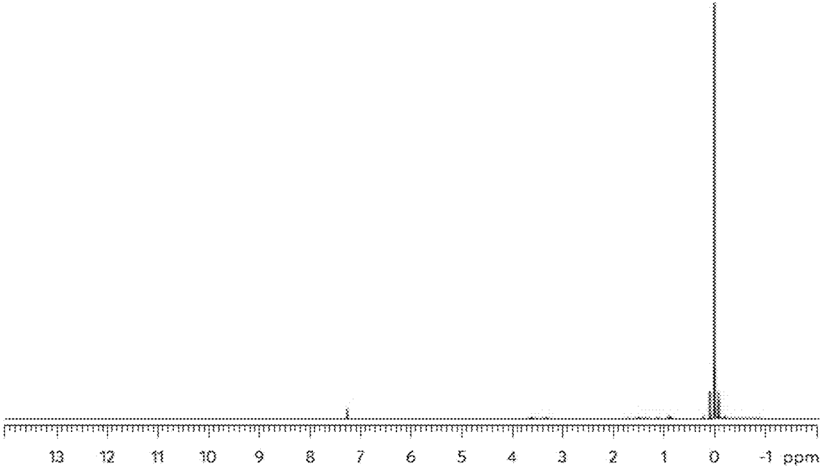
Figure 6: NMR of Me4Sn
