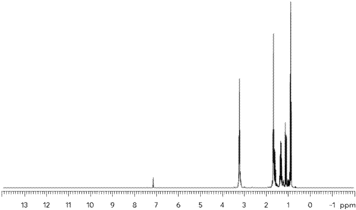
Figure 12: NMR of Bu 2 Sn(Pyrrolodiny) 2
