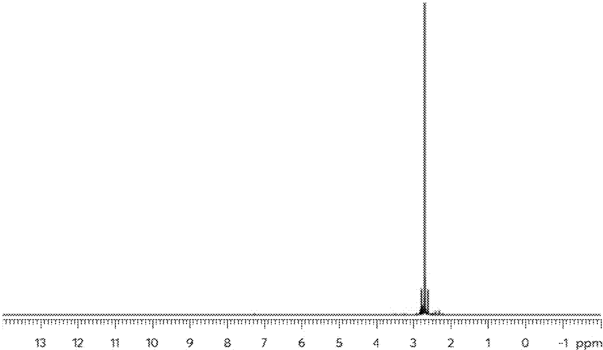
Figure 2: NMR spectrum of \text{Sn}(\text{NMe}_2)_4
