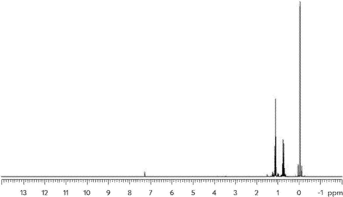
Figure 5: NMR of Me 2 SnEt 2
