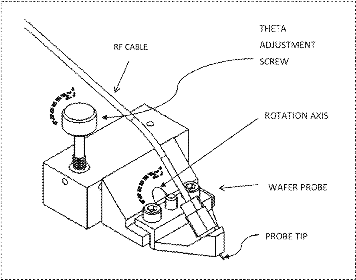
FIG. 13: Prior art
