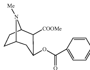
(-)- Cocaine
