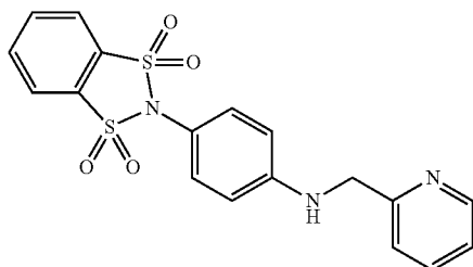
2-4-((pyridine-2-ylmethyl)amino)phenylbenzo[d] [1,3,2]dithiazole-1,1,3,3-tetraoxide
