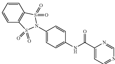
N-(4-(1,1,3,3-tetraoxidobenzo[d][1,3,2]dithiazol-2-yl)phenyl)pyrimidine-4-carboxamide
