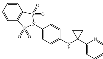
2-4-((1-pyridine-2-yl)cyclopropyl)amino)phenyl benzo[d][1,3,2]dithiazole-1,1,3,3-tetraoxide
