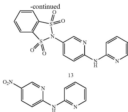
5-nitro-N-(pyridin-2-yl)pyridin-2-amine
