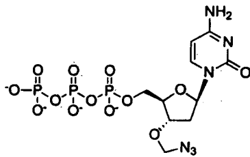
3'-O-Azido-dCTP
