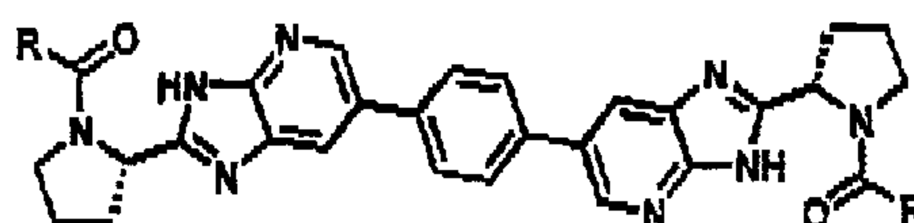
Compounds 2-1 to 2-219
