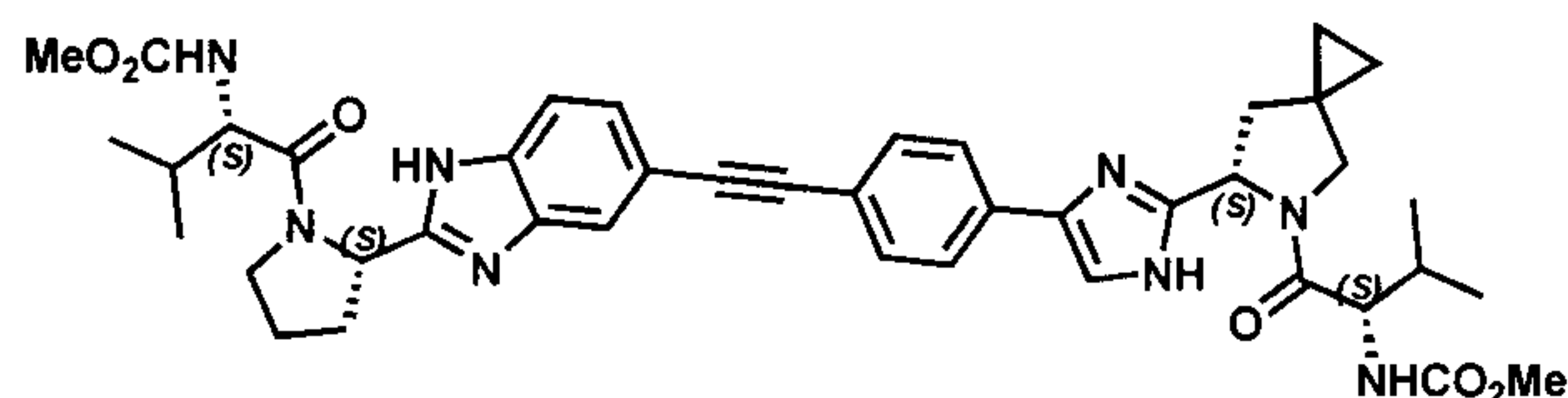
Compound-523
