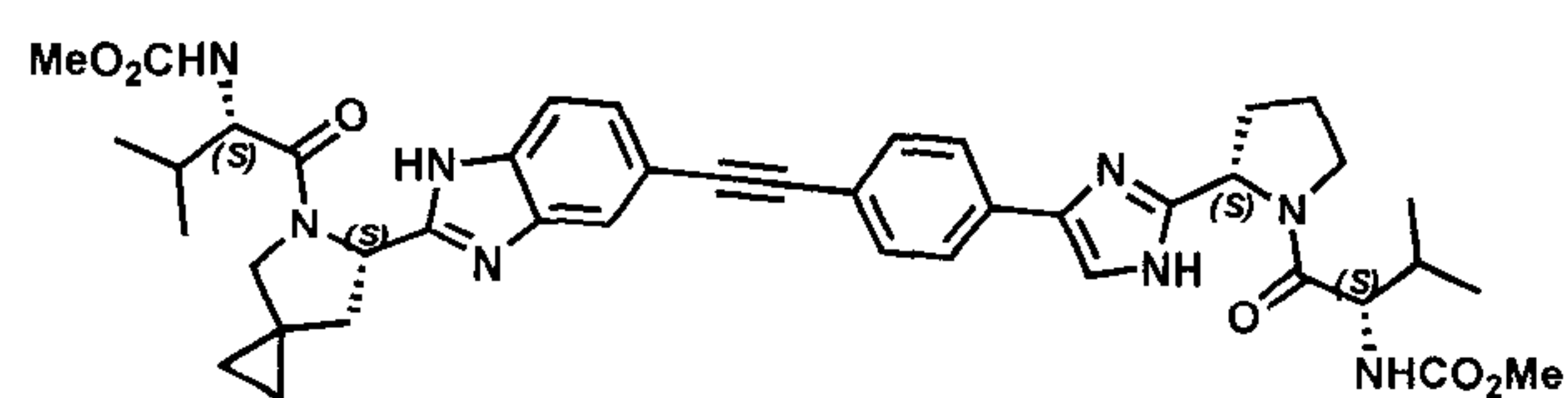
Compound-521
