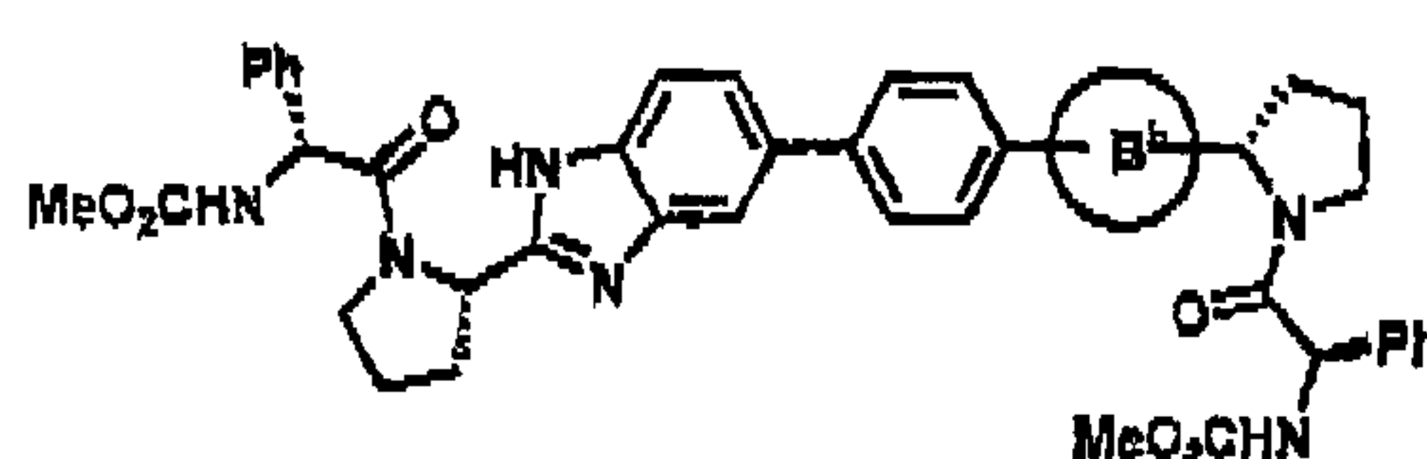
Compounds 1-435 to 1-440
