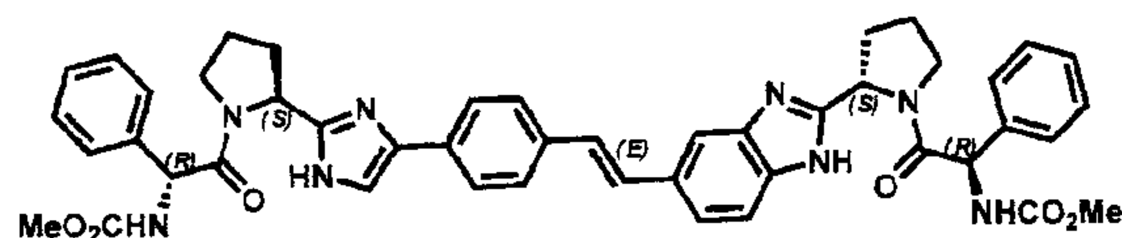
Example 1-357.
