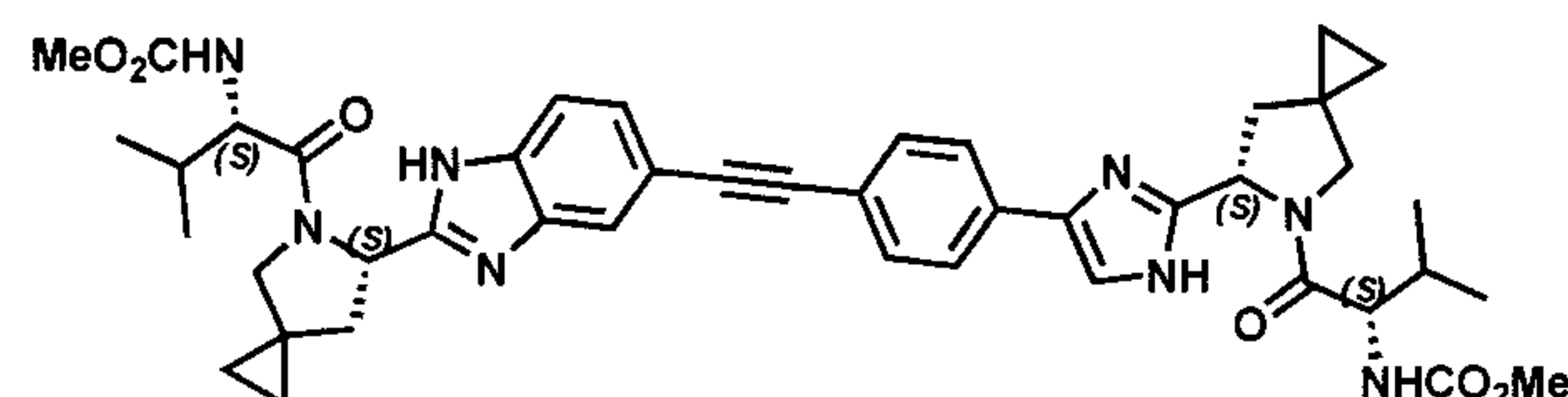
Compound-525
