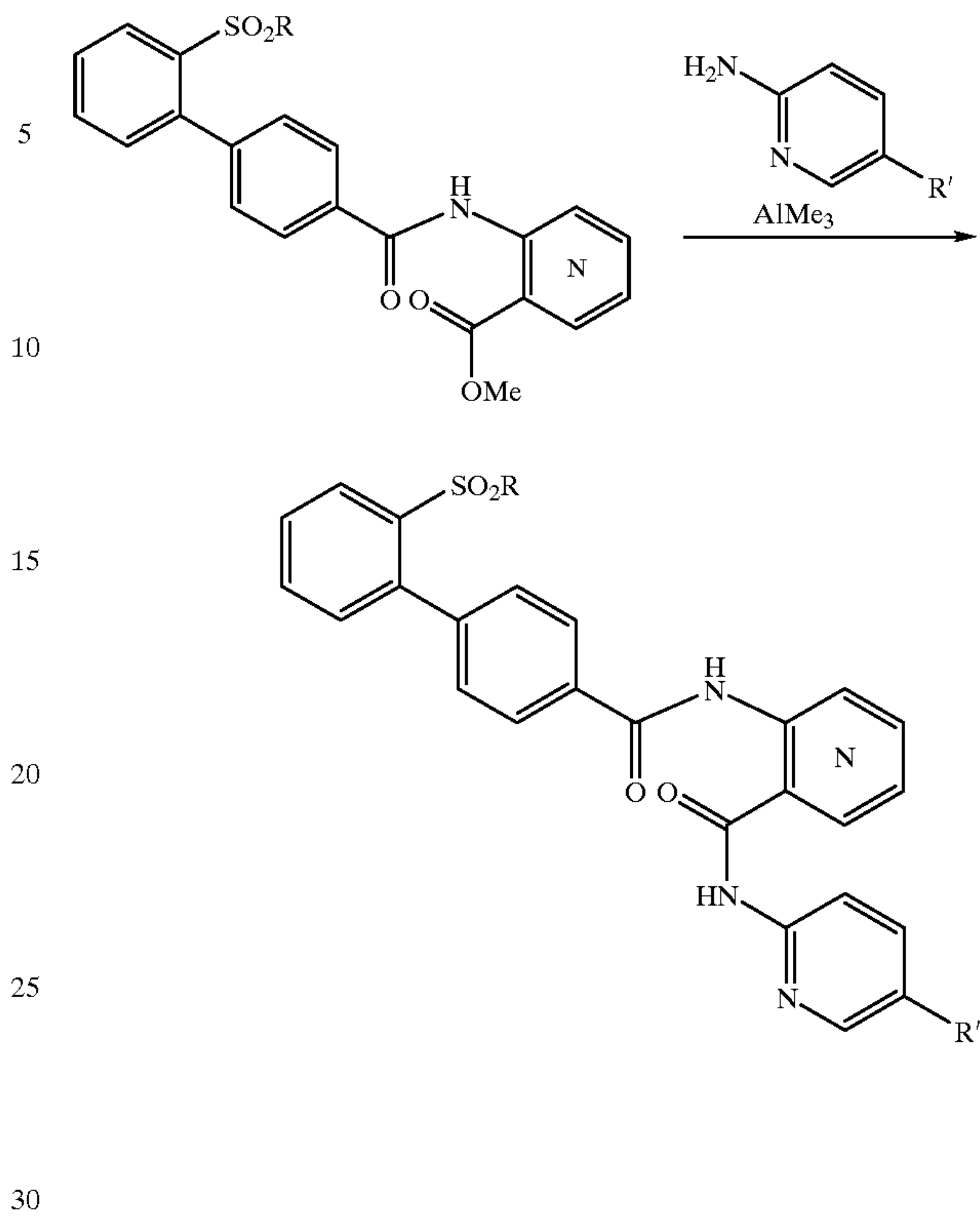
Scheme 7
