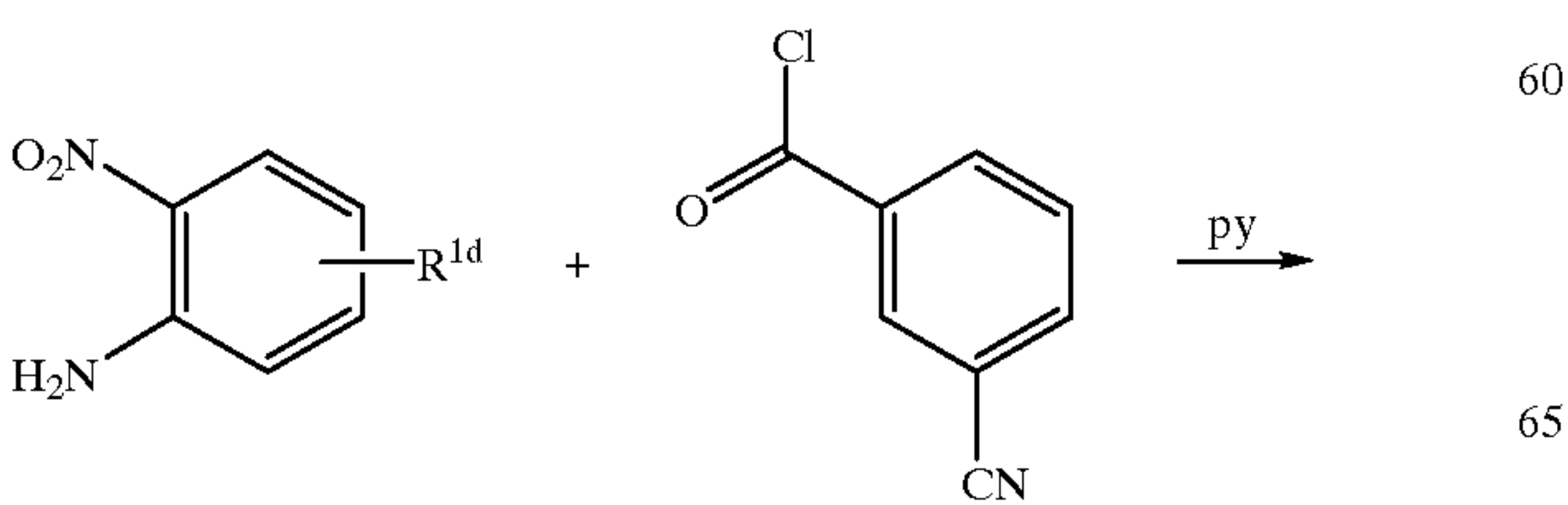
Scheme 15
