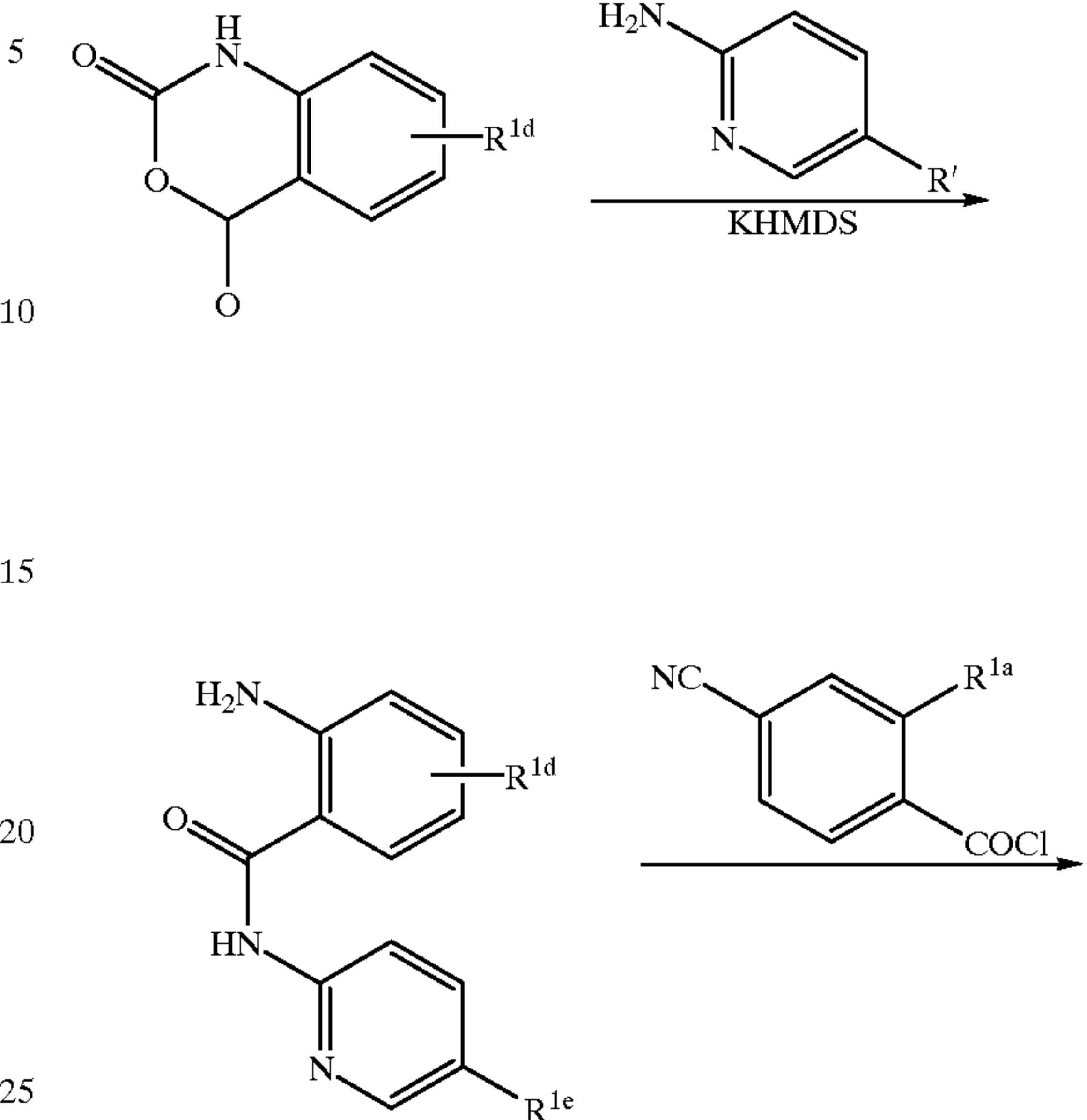
Scheme 10
