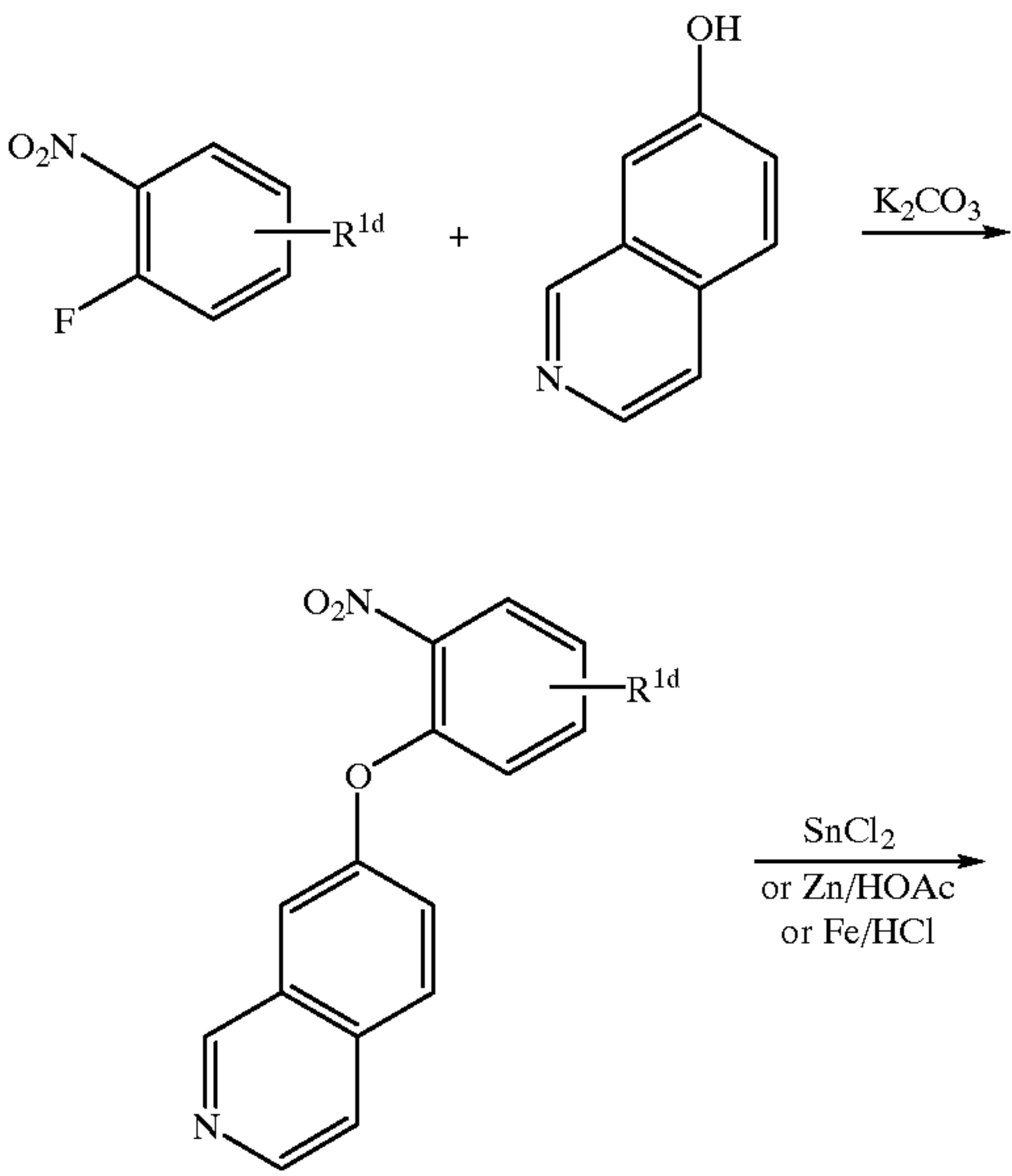
Scheme 2
