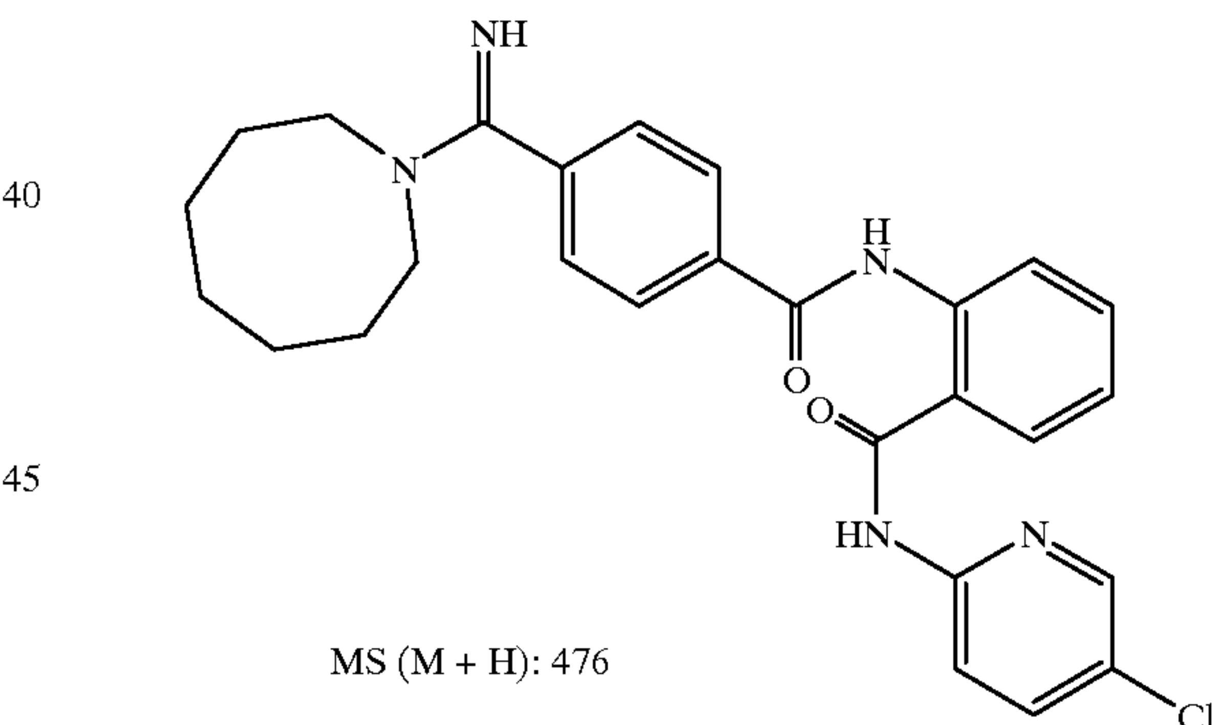
Example 49
