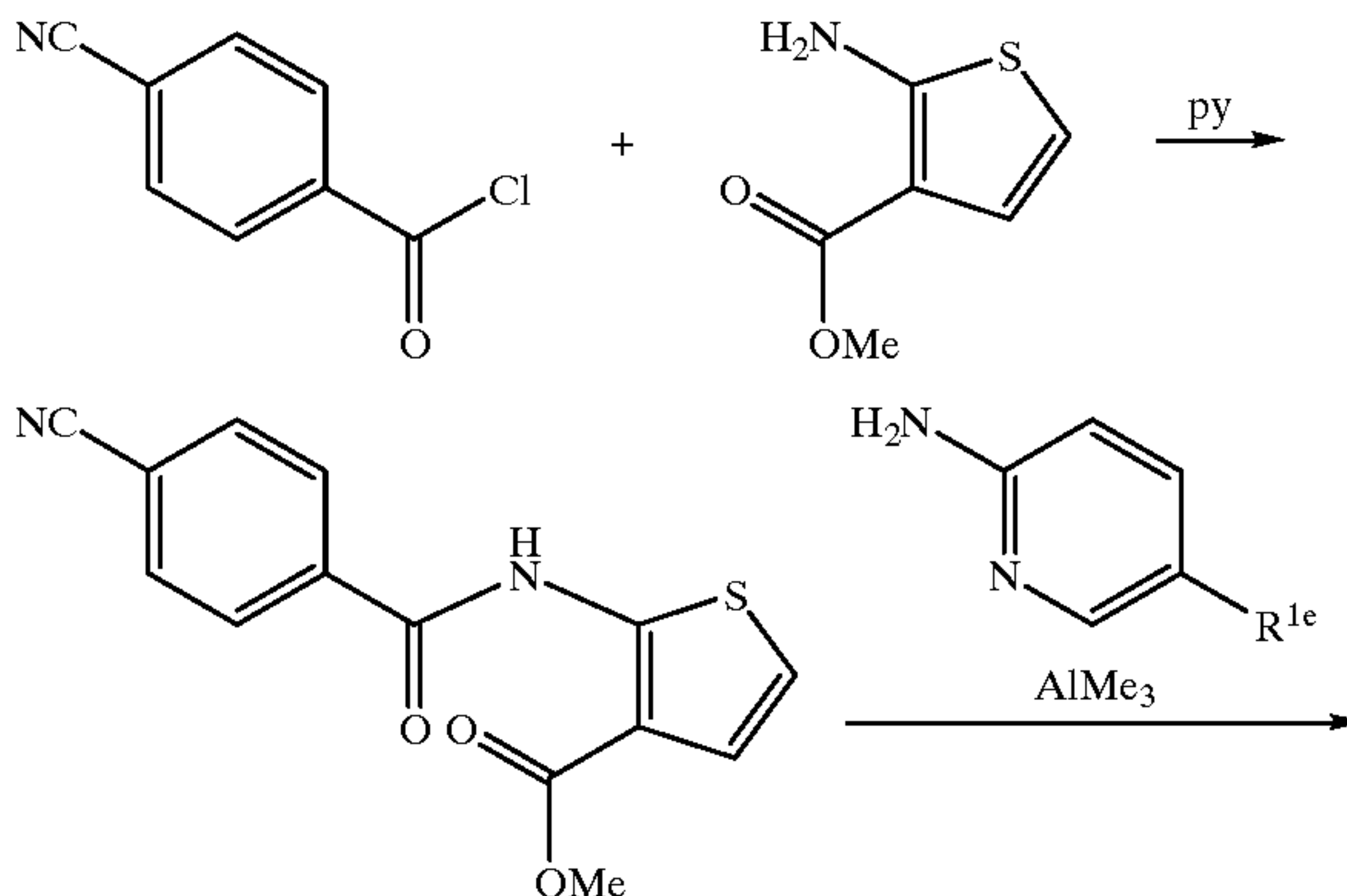
Scheme 12
