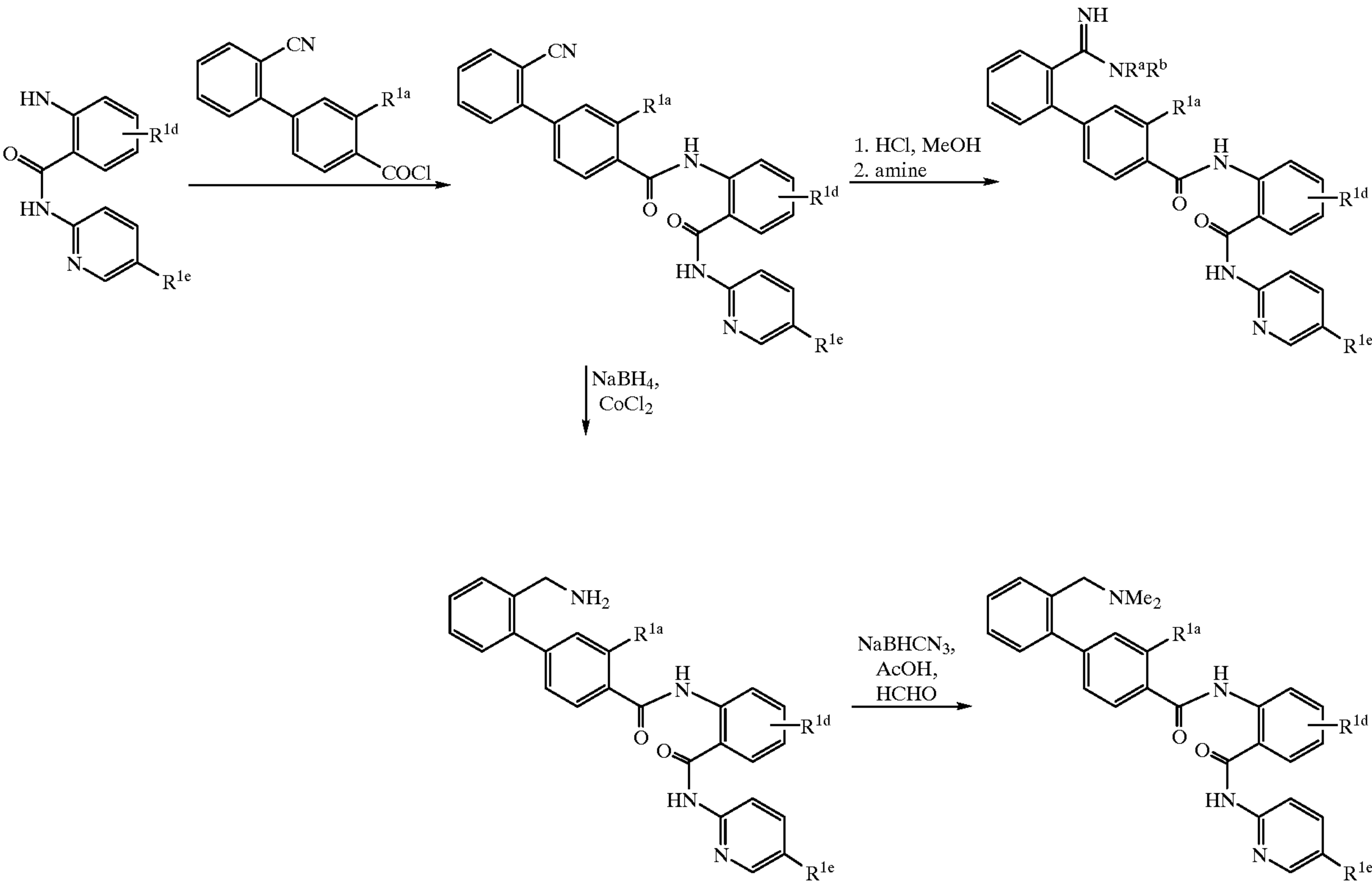
Scheme 9
