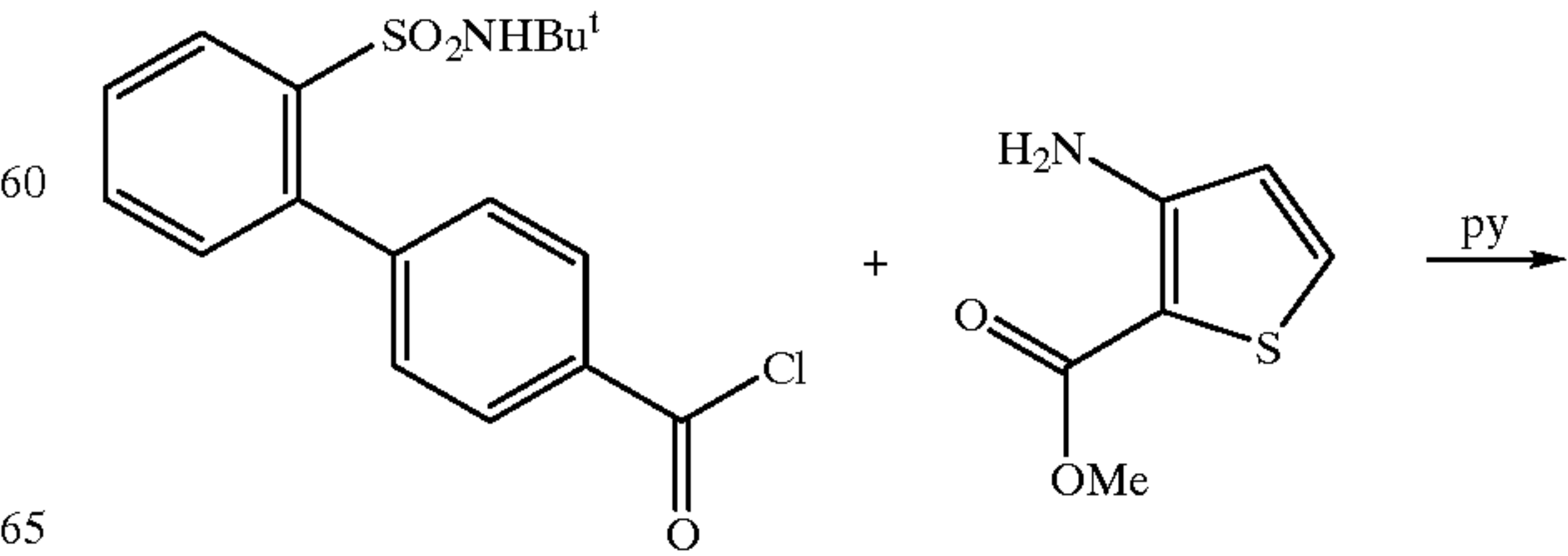
Scheme 14
