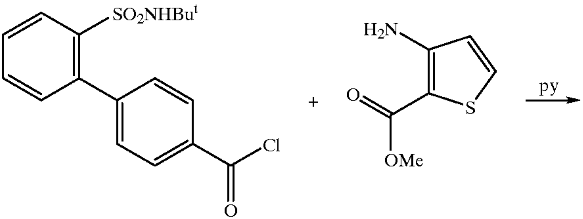
Scheme 13
