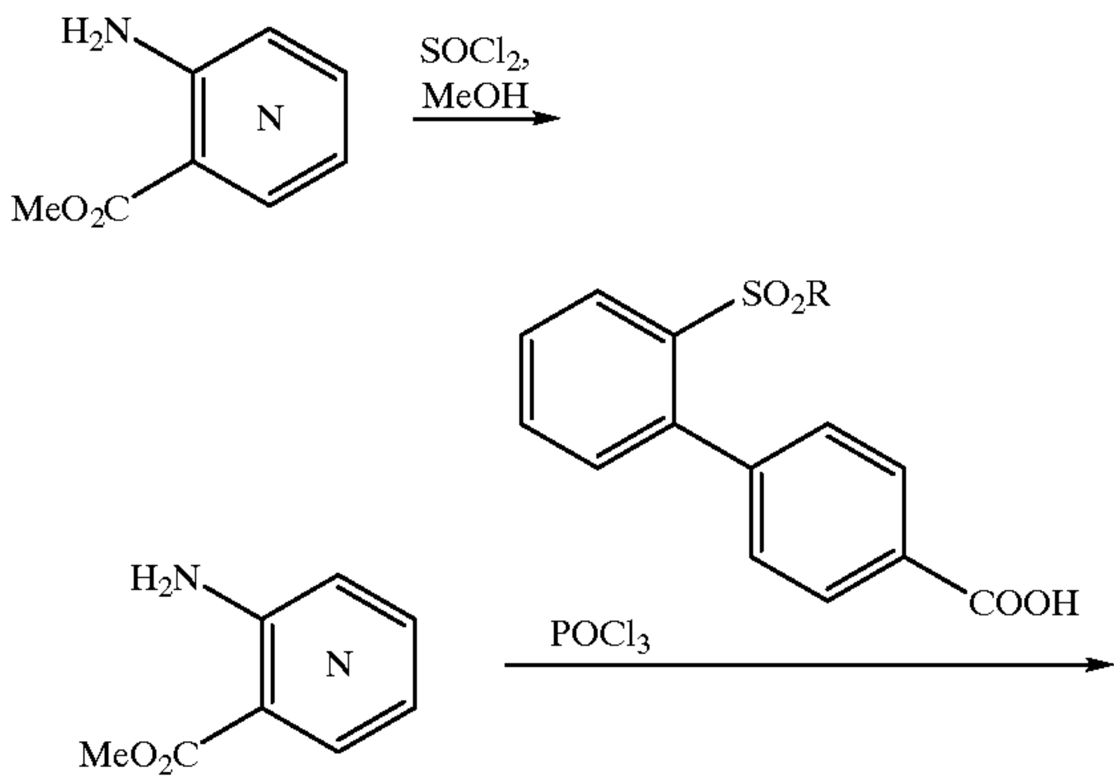
Scheme 6
