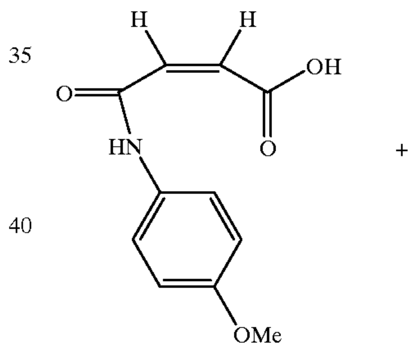
Scheme 7
