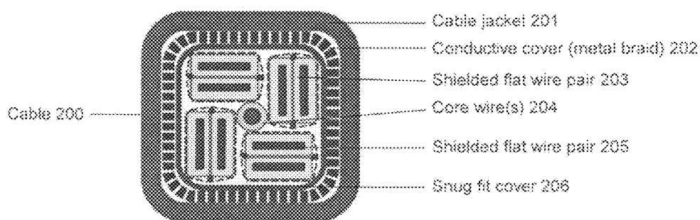
Fig. 2: Compact multichannel flat wire pair cable cross-section
