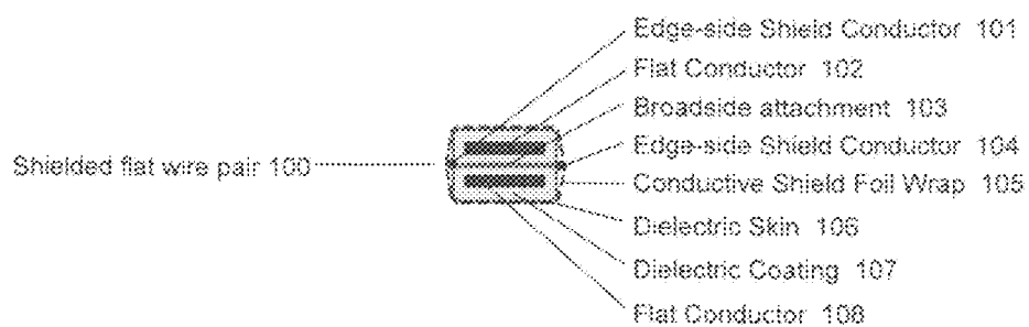
Fig. 1: Flat conductor shielded pair
