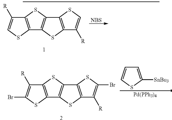
Scheme 2(a) Synthesis of \alpha -, \alpha' -thiophene substituted, \beta -, \beta' -alkyl substituted FT4 using Stille coupling.
