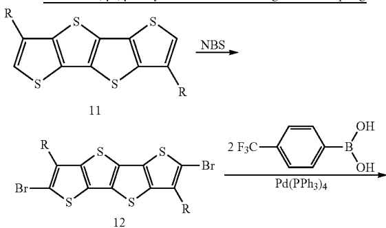
Scheme 2(c) Synthesis of \alpha -, \alpha' -p-trifluoromethylphenyl substituted, \beta -, \beta' -alkyl substituted FT5 using Suzuki coupling.
