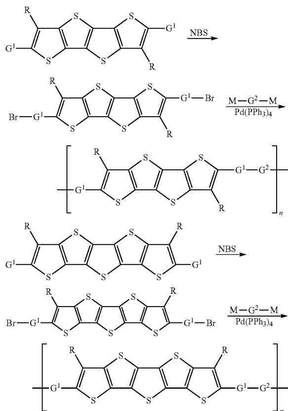
Scheme 1(c) Exemplary synthesis of three-unit polymers from \alpha -, \alpha' -aromatic ring substituted, \beta -, \beta' -alkyl substituted fused thiophenes FT4 and FT5.
