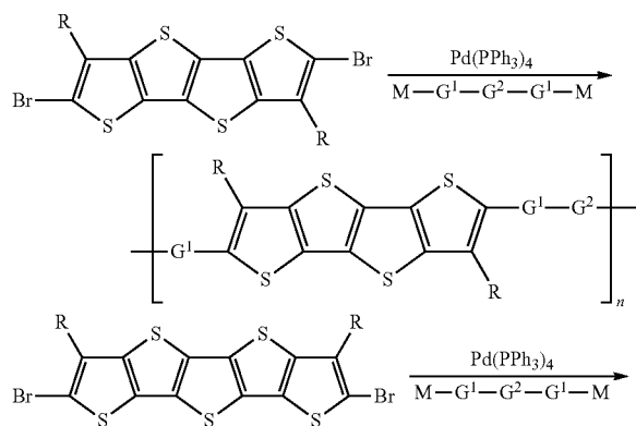
Scheme 1(d) Alternative exemplary syntheses of a three-unit polymer.
