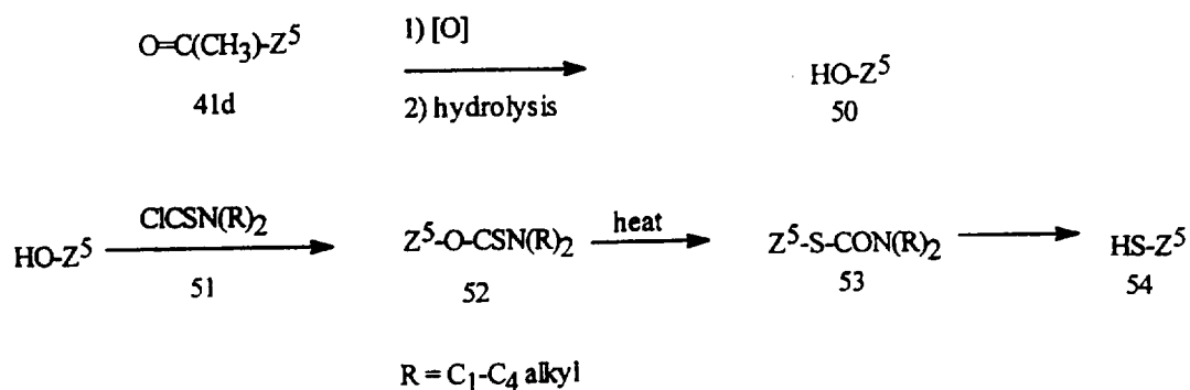
Scheme 30
