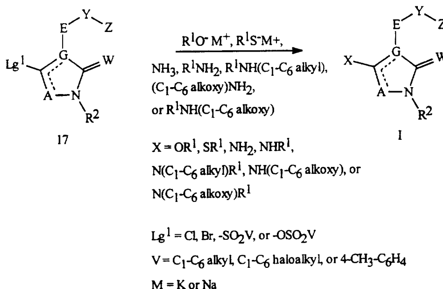
Scheme 9
