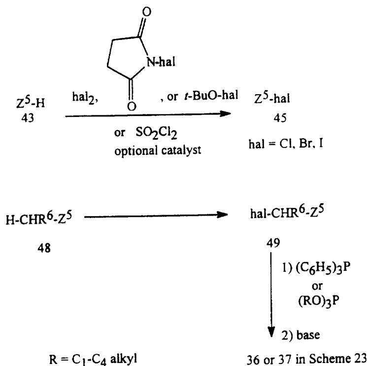
43 Scheme 29
