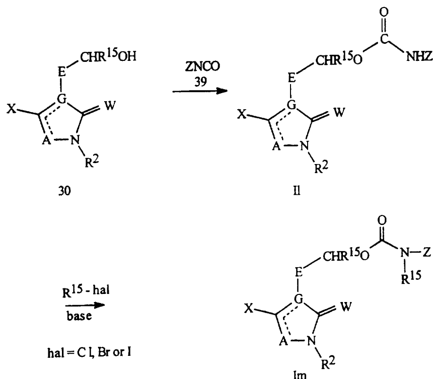
Scheme 25
