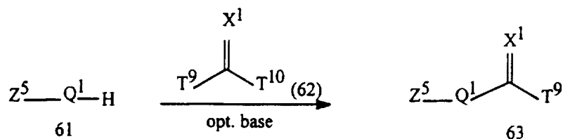
Scheme 34
