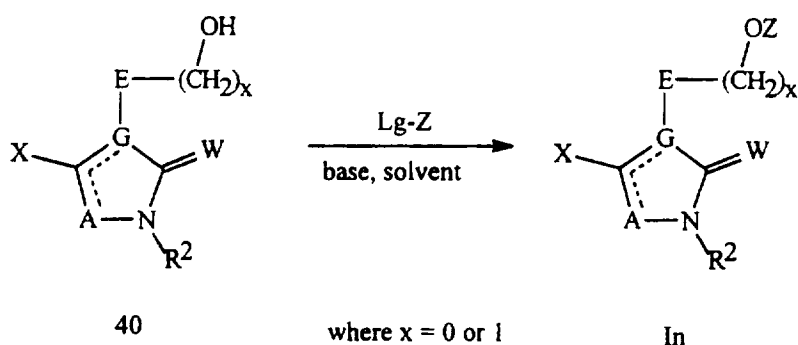
Scheme 26
