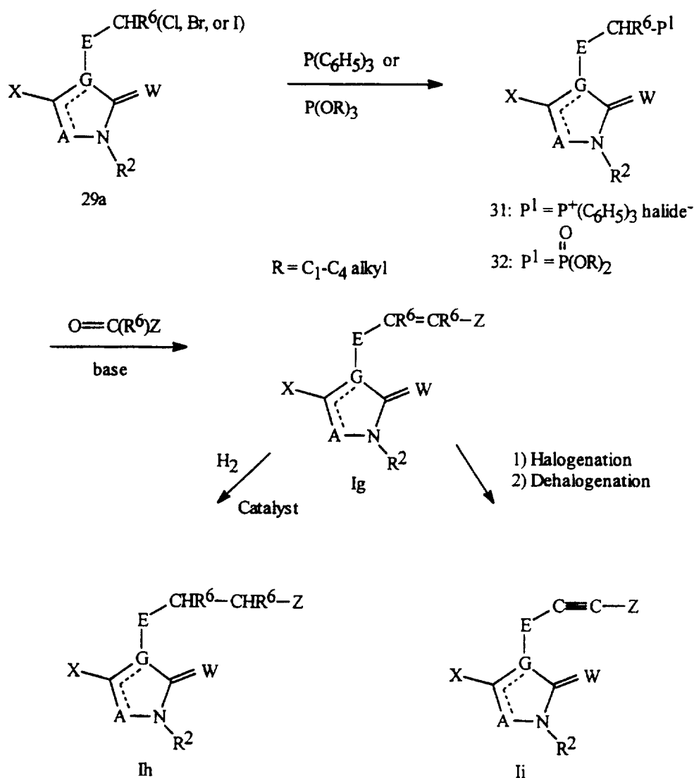
Scheme 22
