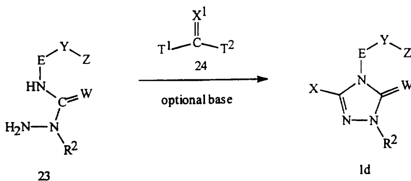
Scheme 16
