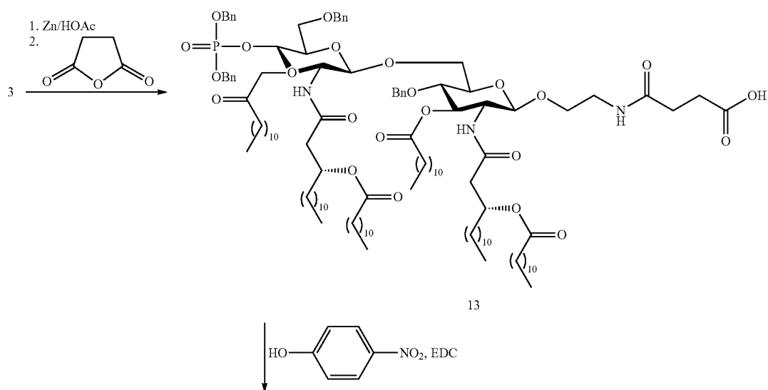
Scheme 2 Synthesis of 1
