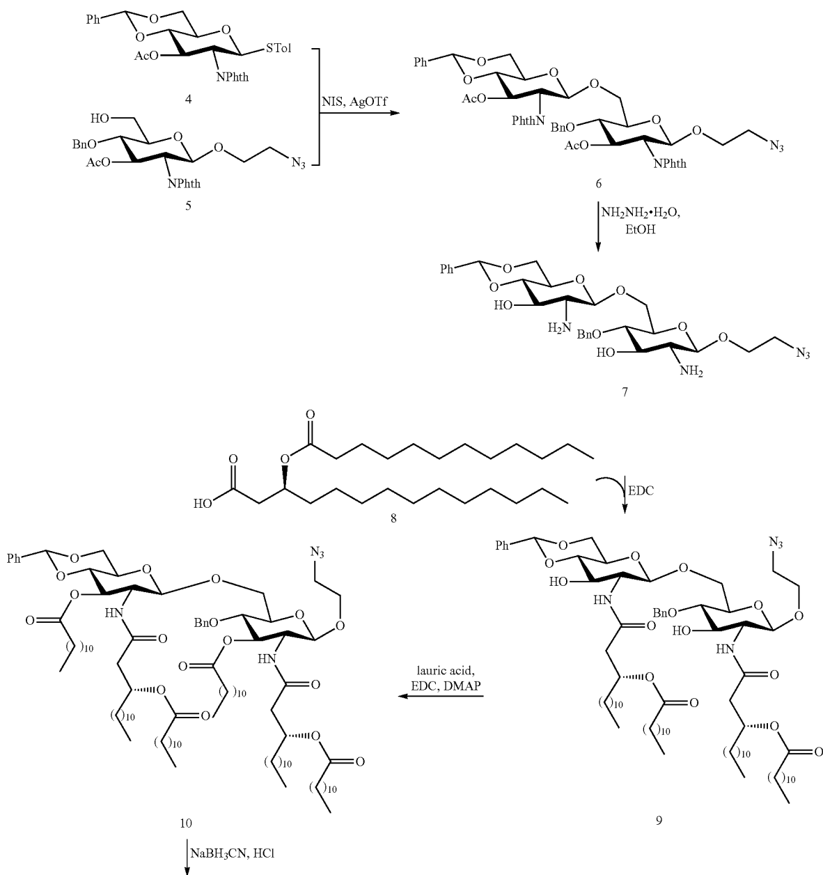
Scheme 1 Synthesis of 3
