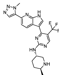
Compound 150:
