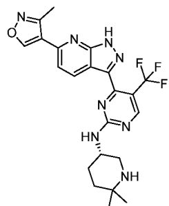
Compound 160:
