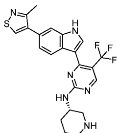
Compound 131:
