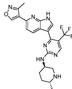
Compound 159:
