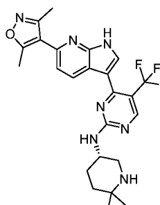
Compound 119:
