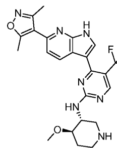
Compound 120:
