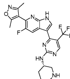
Compound 138:
