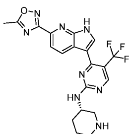
Compound 142:
