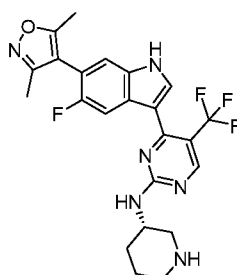
Compound 134:
