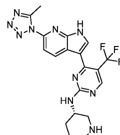
Compound 144:
