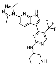
Compound 143:
