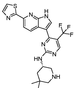
Compound 137:
