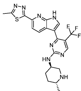
Compound 157:
