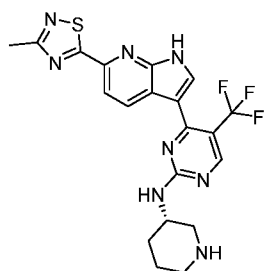
Compound 145:
