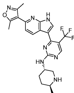
Compound 127:
