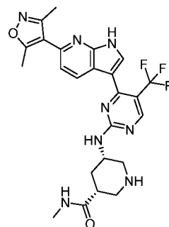
Compound 123:
