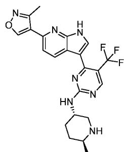
Compound 157:
