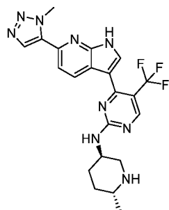
Compound 151:
