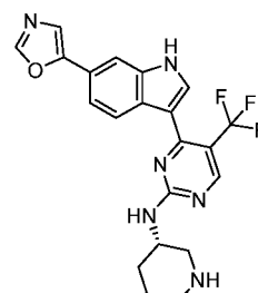
Compound 111:
