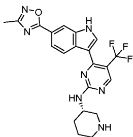
Compound 124:
