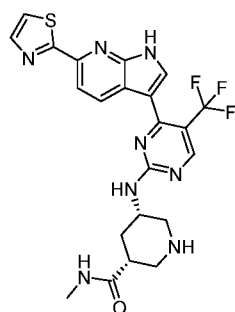
Compound 148:
