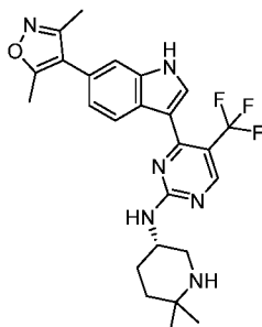
Compound 107:
