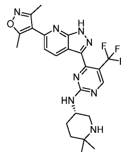
Compound 147:
