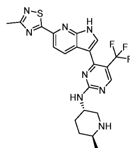
Compound 159:
