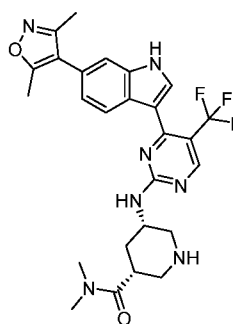
Compound 115:
