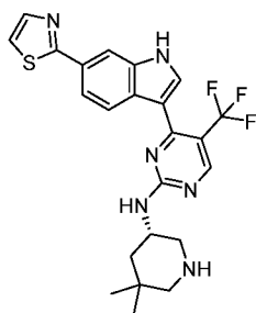
Compound 112:
