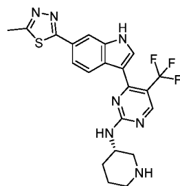
Compound 126:
