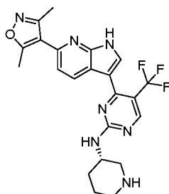
Compound 104:
