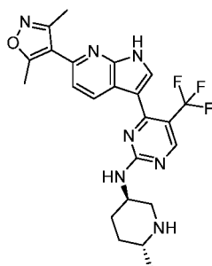
Compound 128:
