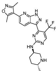
Compound 152:
