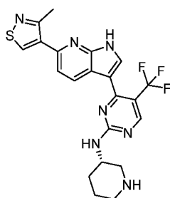
Compound 149:
