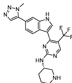
Compound 126:
