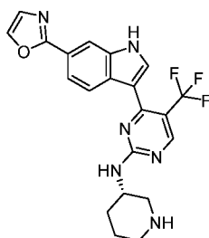
Compound 110:
