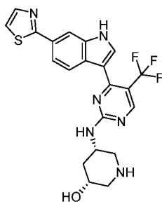
Compound 110:
