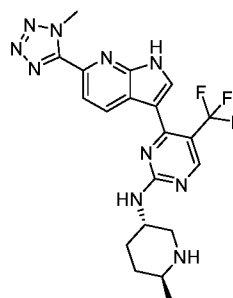
Compound 167:
