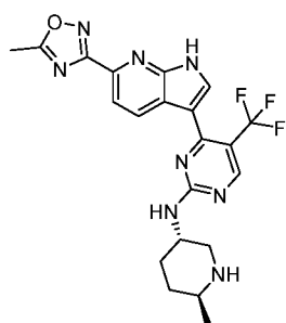
Compound 166:
