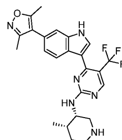
Compound 135:
