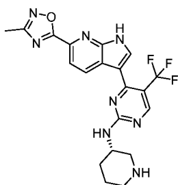
Compound 136:
