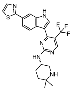
Compound 109:
