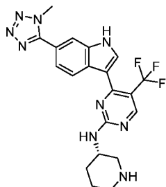
Compound 125:
