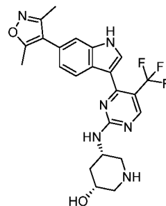
Compound 108:
