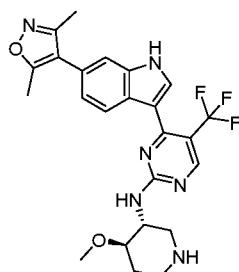
Compound 130:
