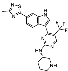
Compound 130:
