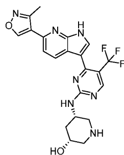
Compound 148:
