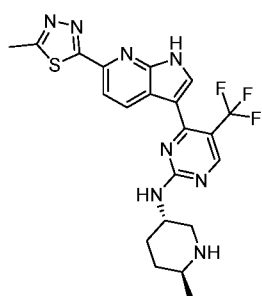
Compound 158:
