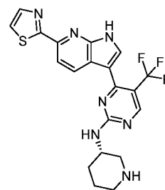
Compound 111:
