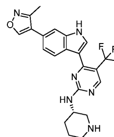
Compound 114:
