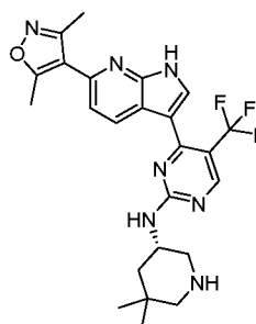
Compound 118:
