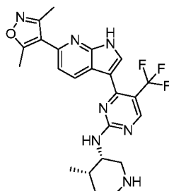
Compound 146:
