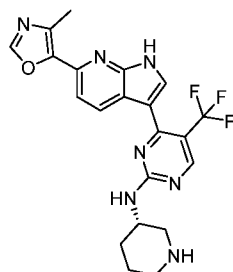
Compound 161:
