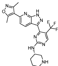
Compound 121:
