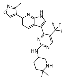
Compound 150:
