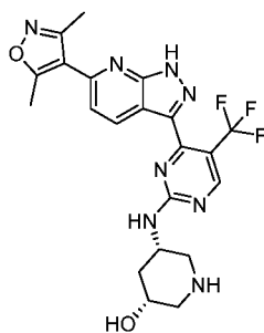
Compound 149:
