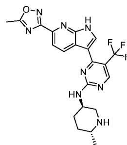
Compound 162:
