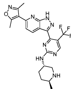
Compound 153:
