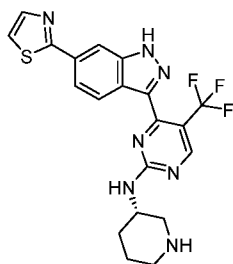
Compound 103:
