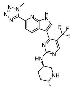
Compound 168:
