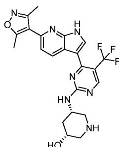
Compound 136:
