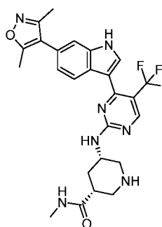
Compound 116:
