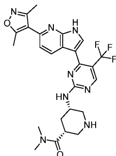
Compound 122:
