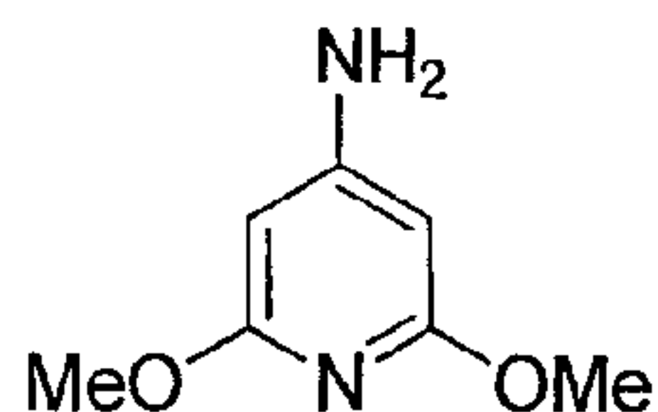
2,6-Dimethoxypyridin-4-amine
