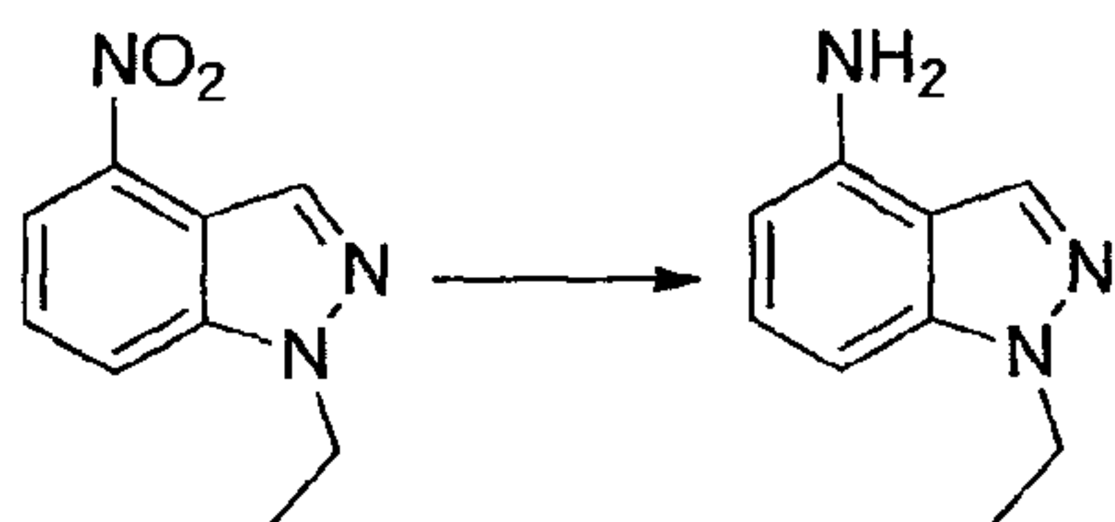
1-Ethyl-1H-indazol-4-amine
