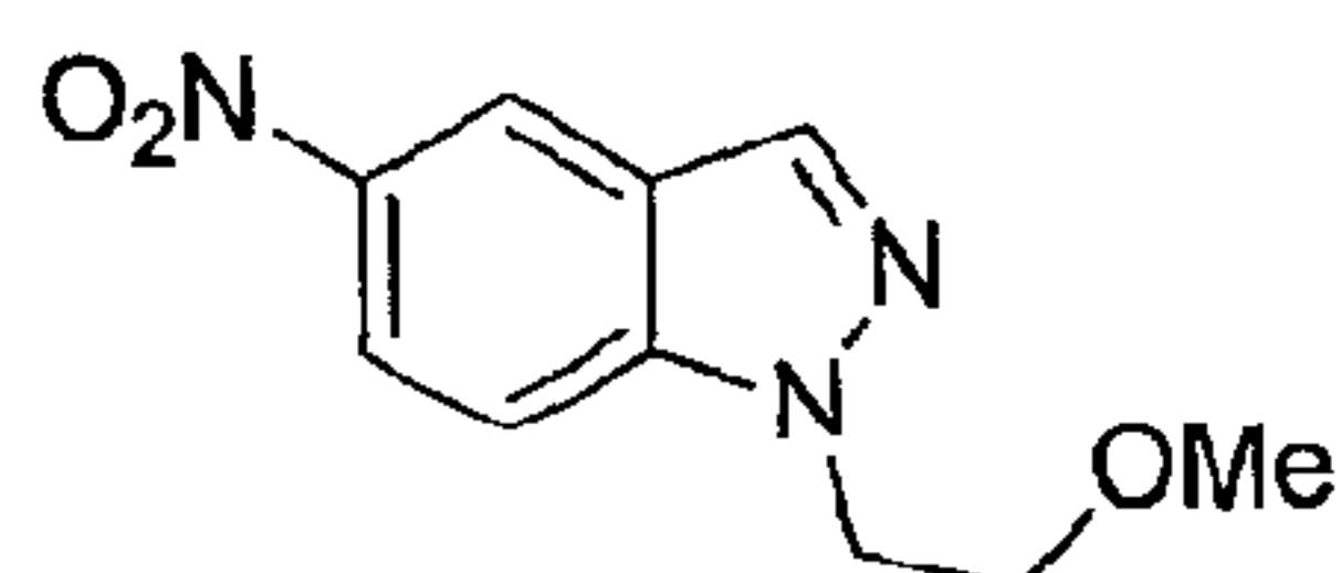
1-(2-Methoxyethyl)-5-nitro-1H-indazole
