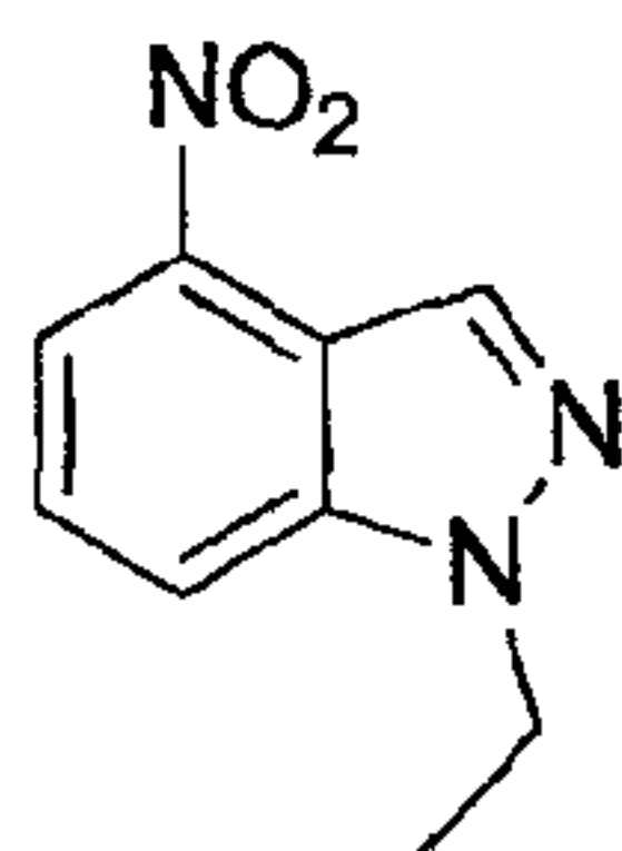
1-Ethyl-4-nitro-1H-indazole
