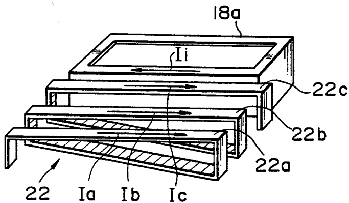
FIG. 2 PRIOR ART
