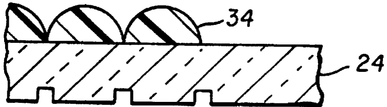
FIG. 3C (PRIOR ART)
