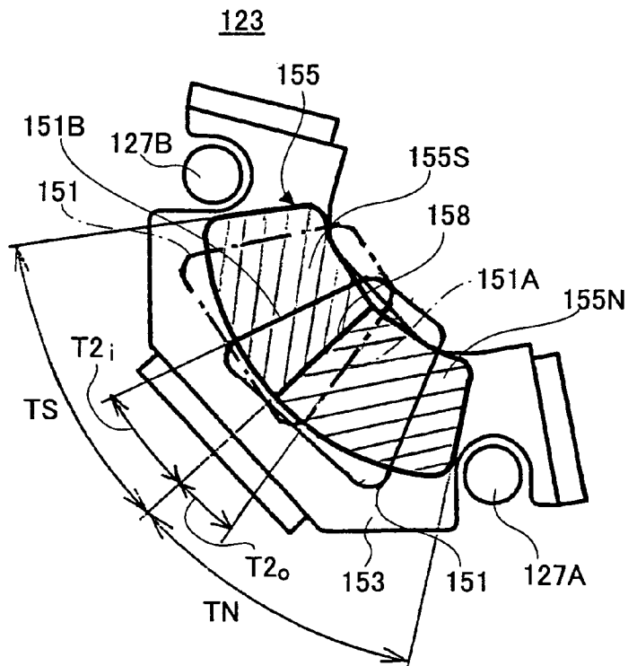
FIG.7 PRIOR ART
