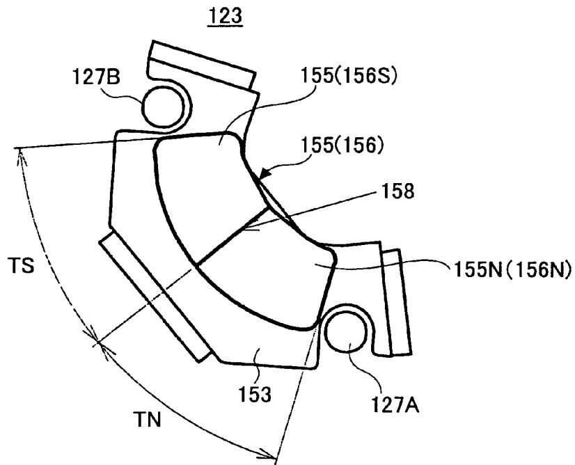
FIG.6 PRIOR ART
