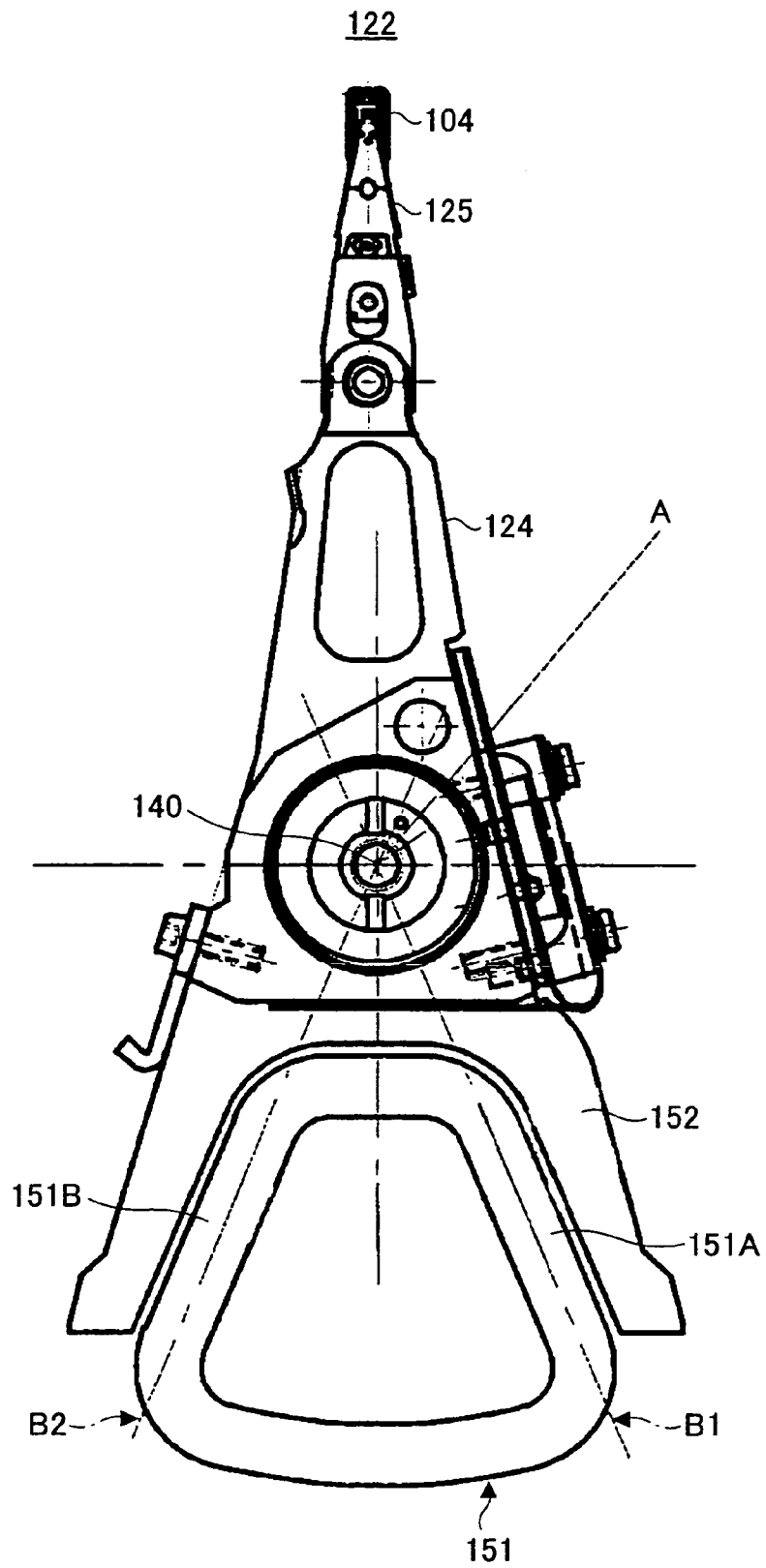
FIG.3 PRIOR ART
