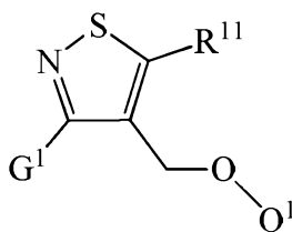
Formula (II)
