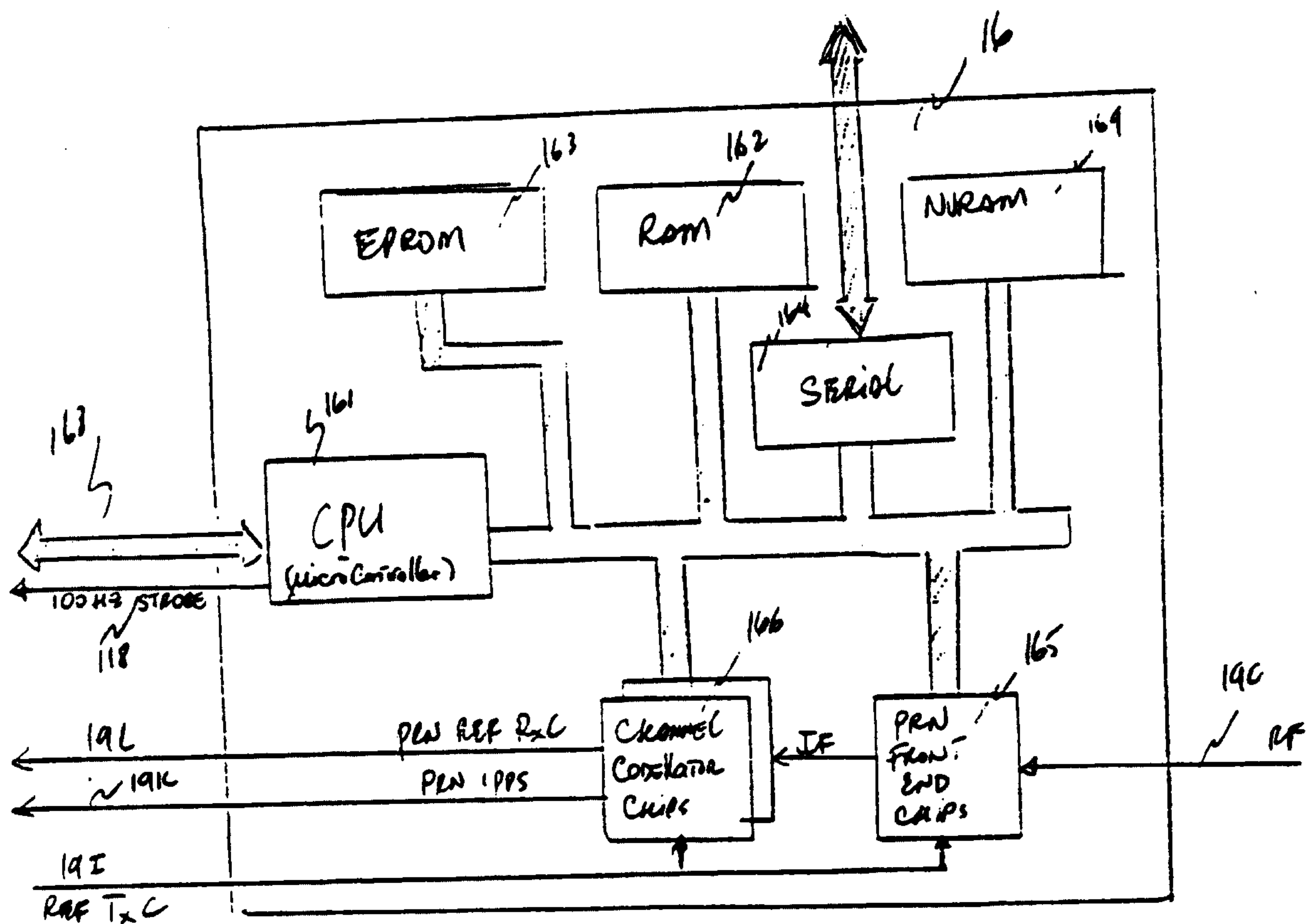
THE PRN RECEIVER (FIGURE 16)
