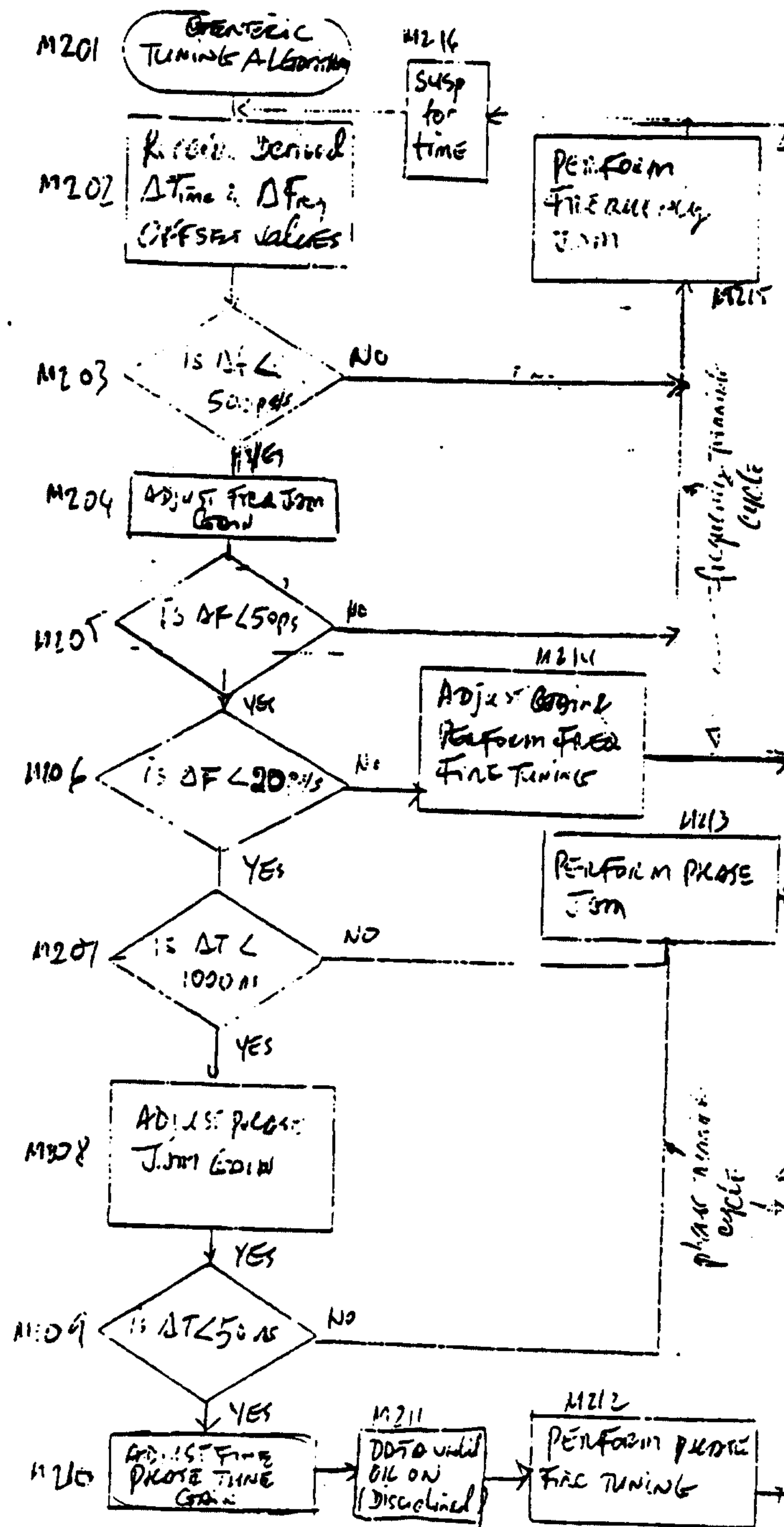
MODE 2 GENERIC TUNING ALGORITHM (FIGURE 9a)
