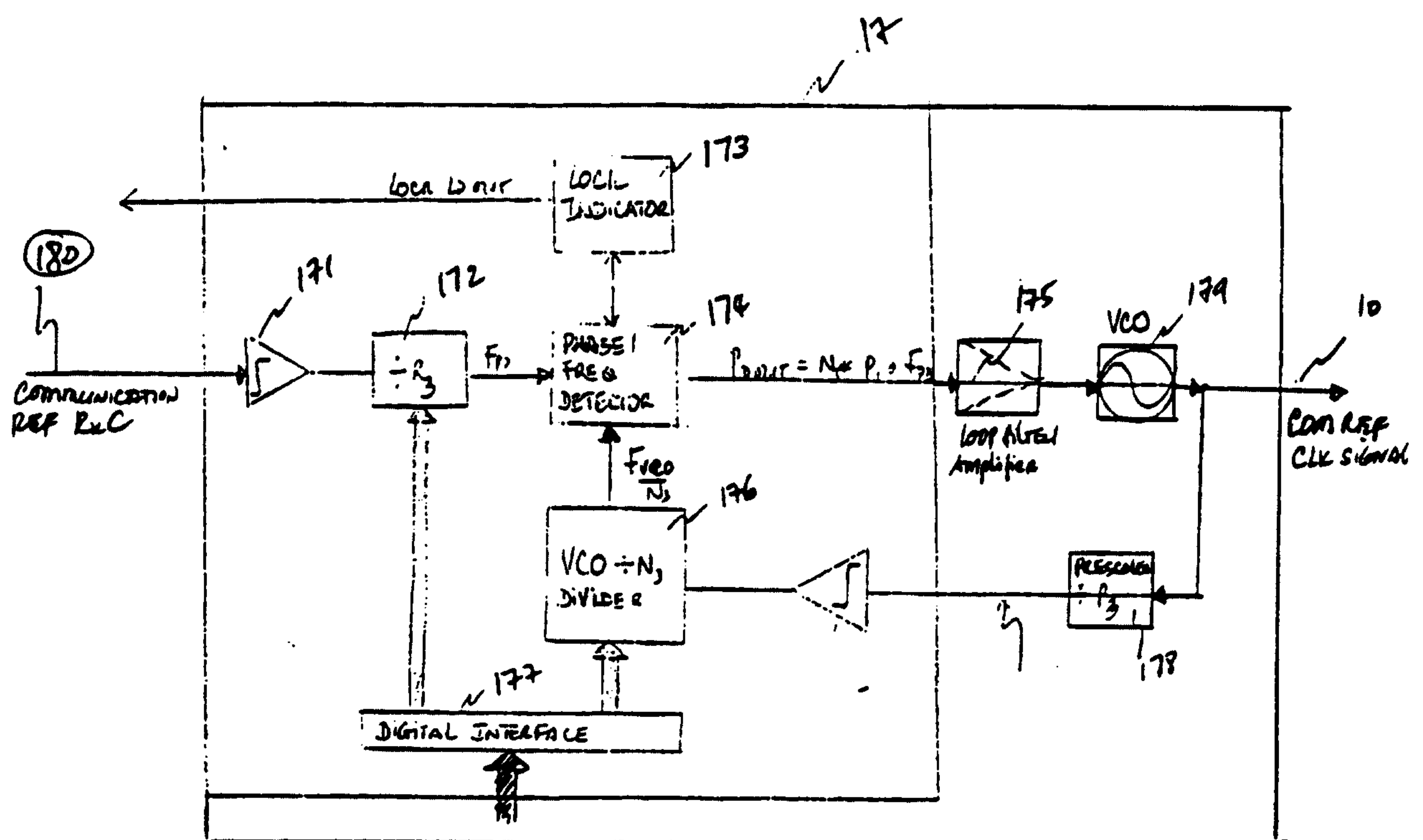
Com Ref CLK Generator
