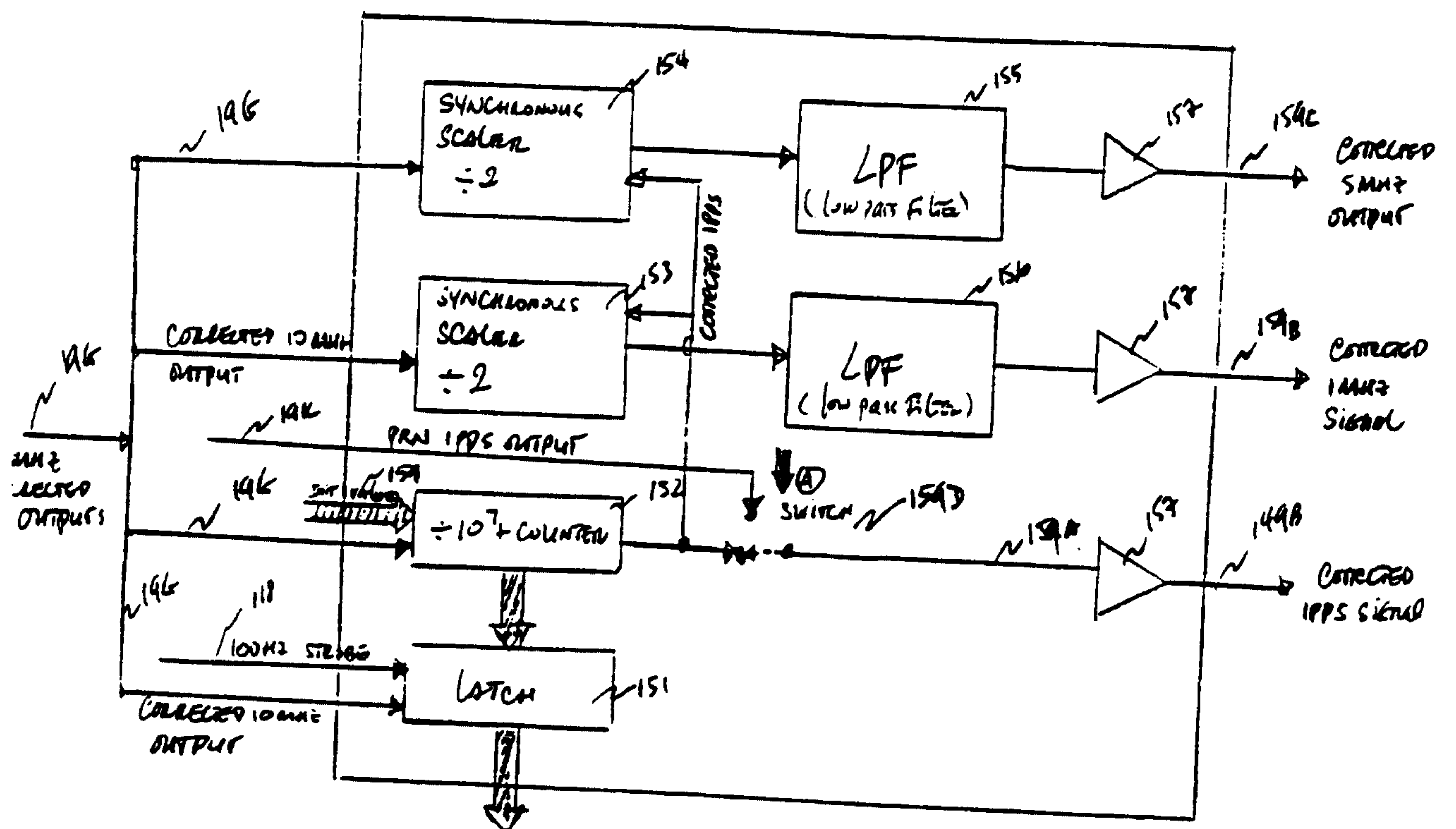
CORRECTED OUTPUT GENERATOR (FIGURE 15)
