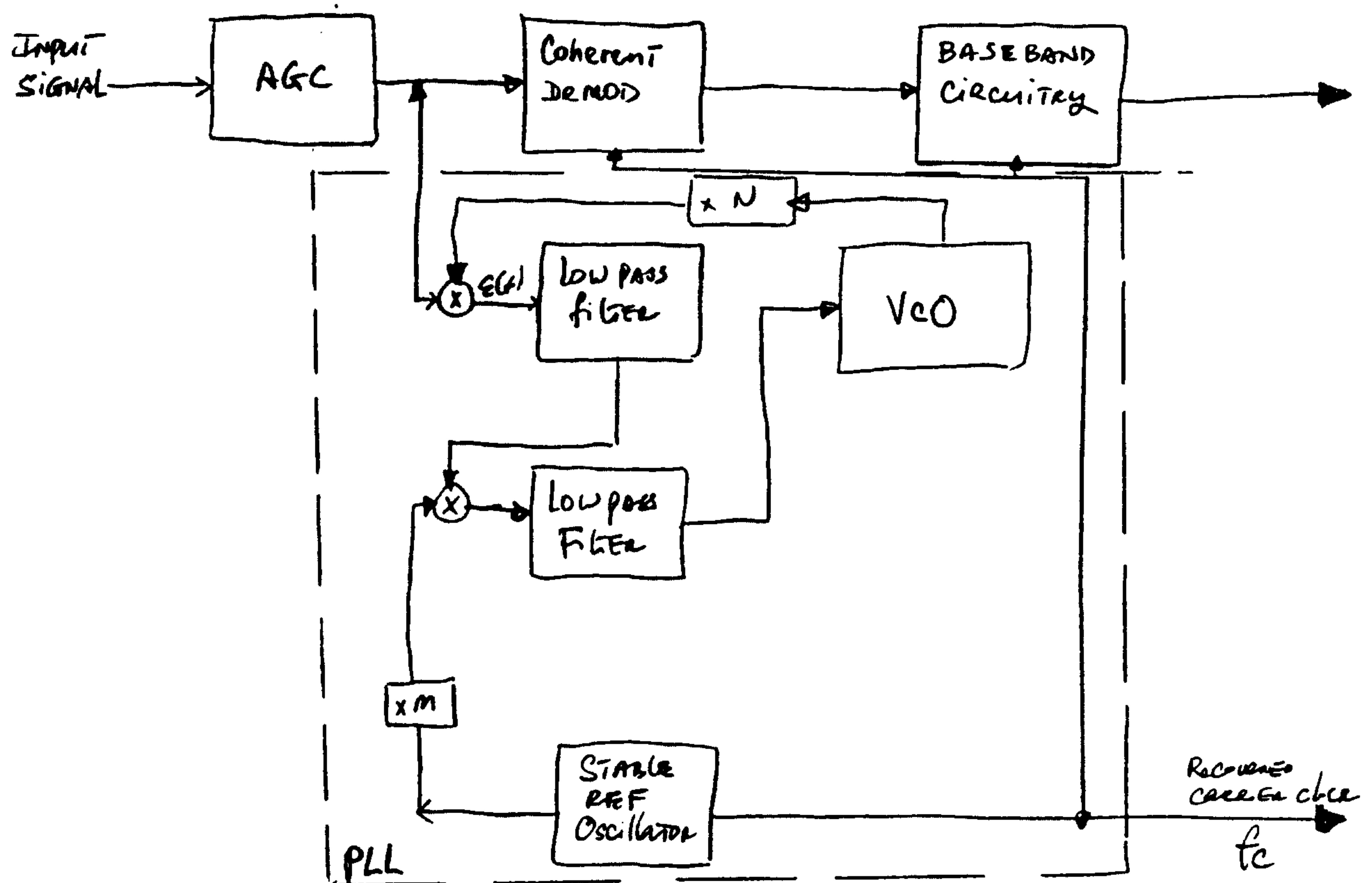
COM2000™ Coherent Carrier Recovery
