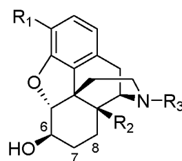
6\beta -isomer
