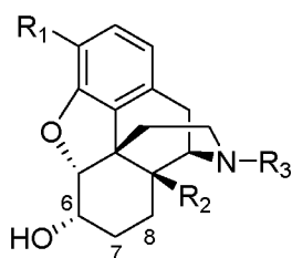
6\alpha -isomer
