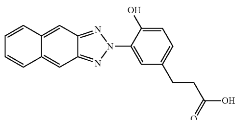
3-(4-Hydroxy-3-(2H-naphtho[2,3-d][1,2,3]triazol-2-yl)phenyl)propanoic acid (Compound D)
