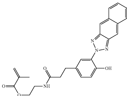
2-(3-(4-hydroxy-3-(2H-naphtho[2,3-d][1,2,3]triazol-2-yl)phenyl)propanamido)ethyl methacrylate
