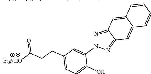
triethylamine 3-(4-hydroxy-3-(2H-naphtho[2,3-d][1,2,3]triazol-2-yl)phenyl)propanoate (Compound E)
