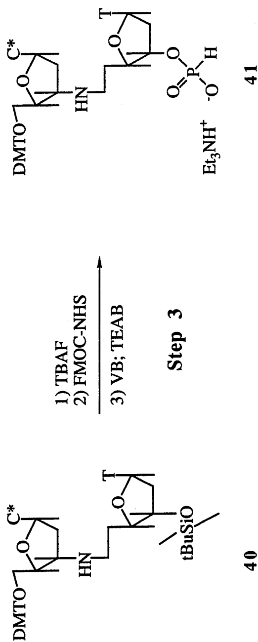
Reaction Scheme 7
