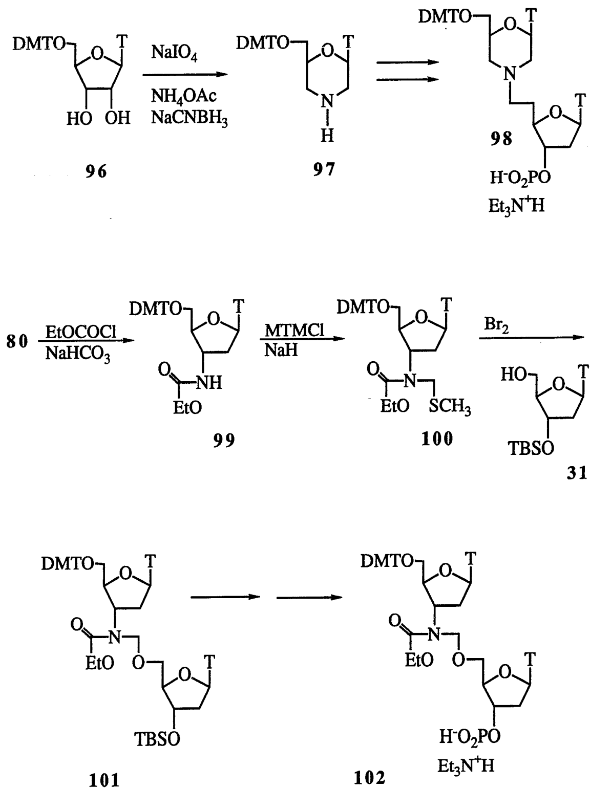
Reaction Scheme 14
