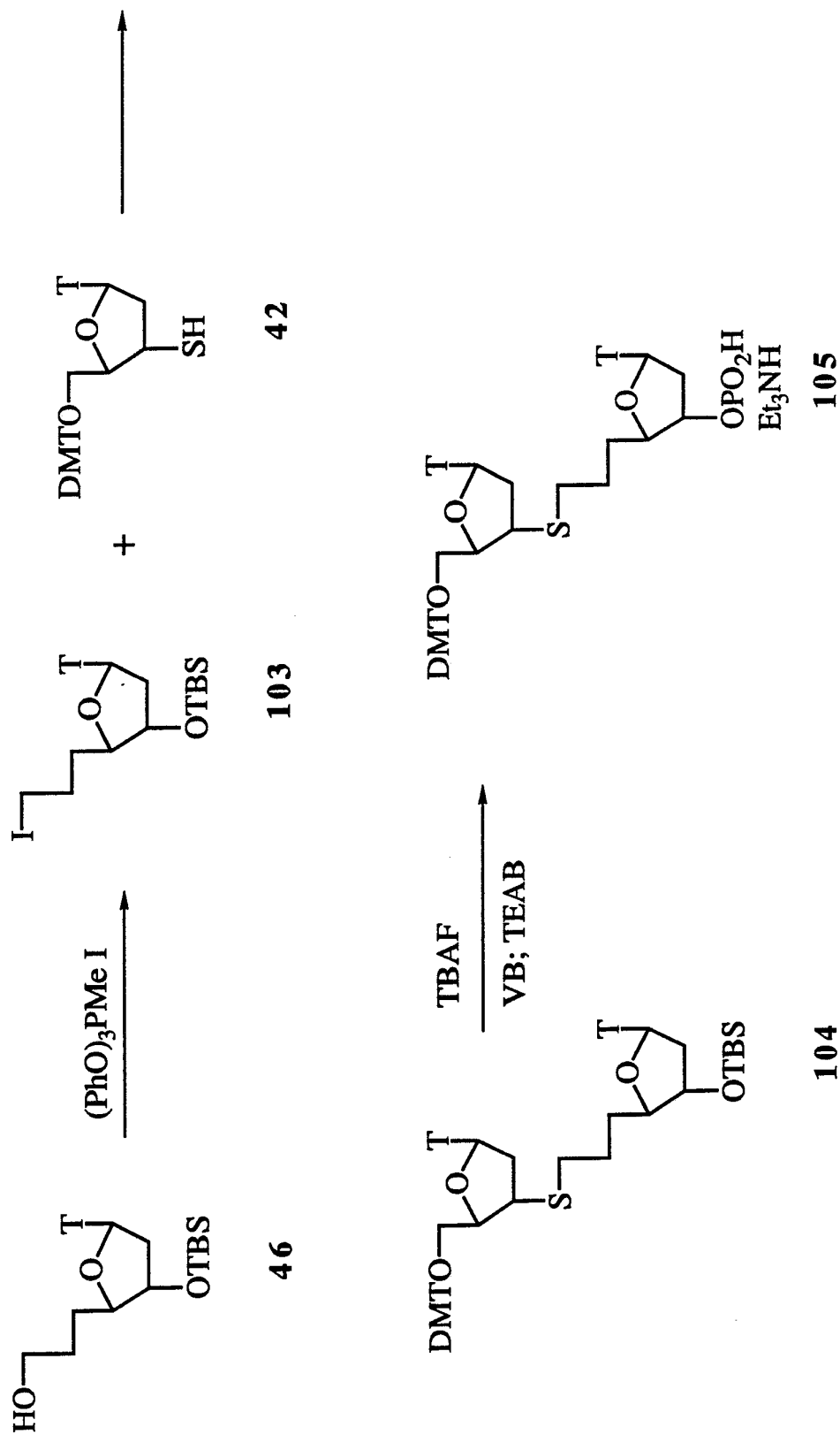
Reaction Scheme 15
