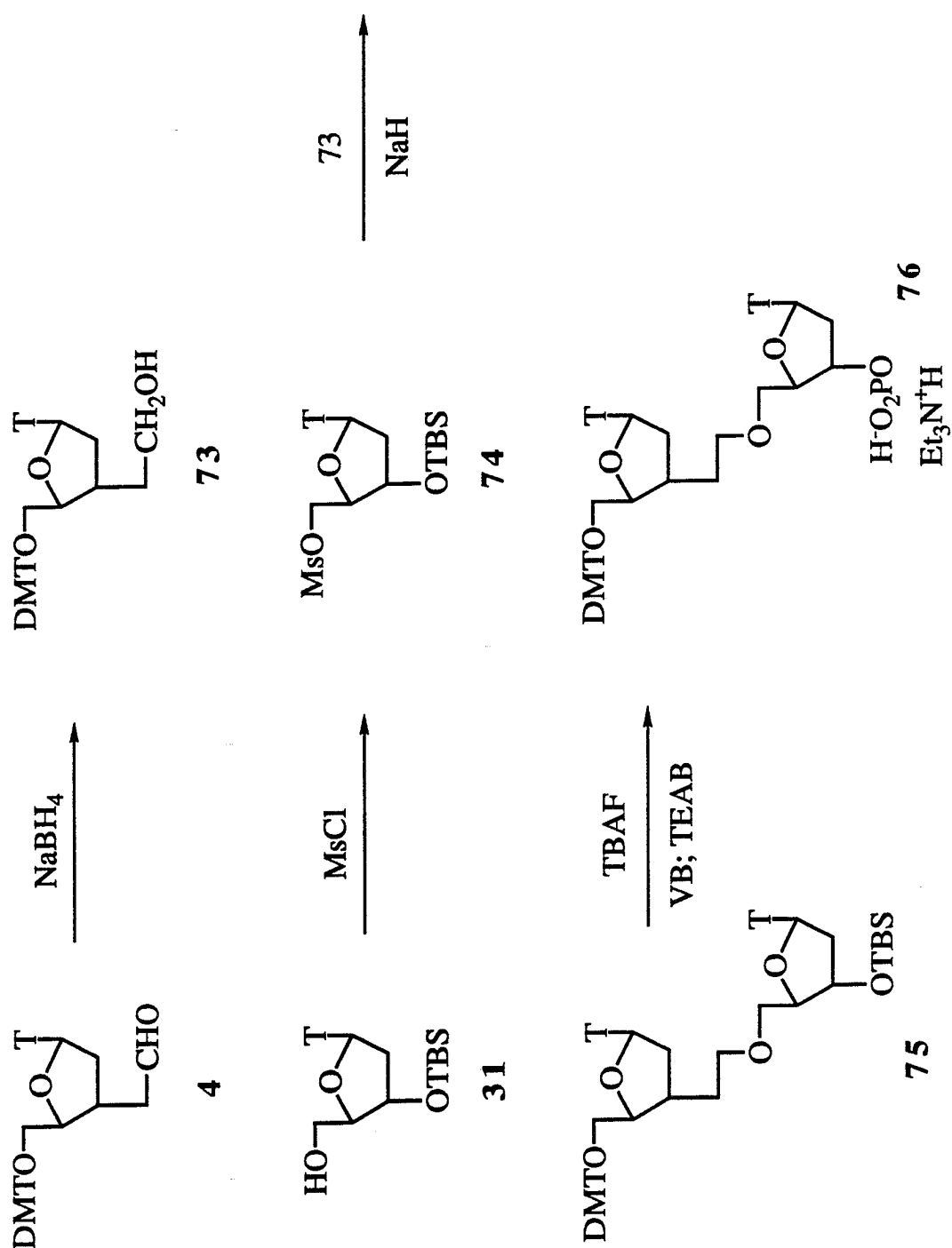
Reaction Scheme 12
