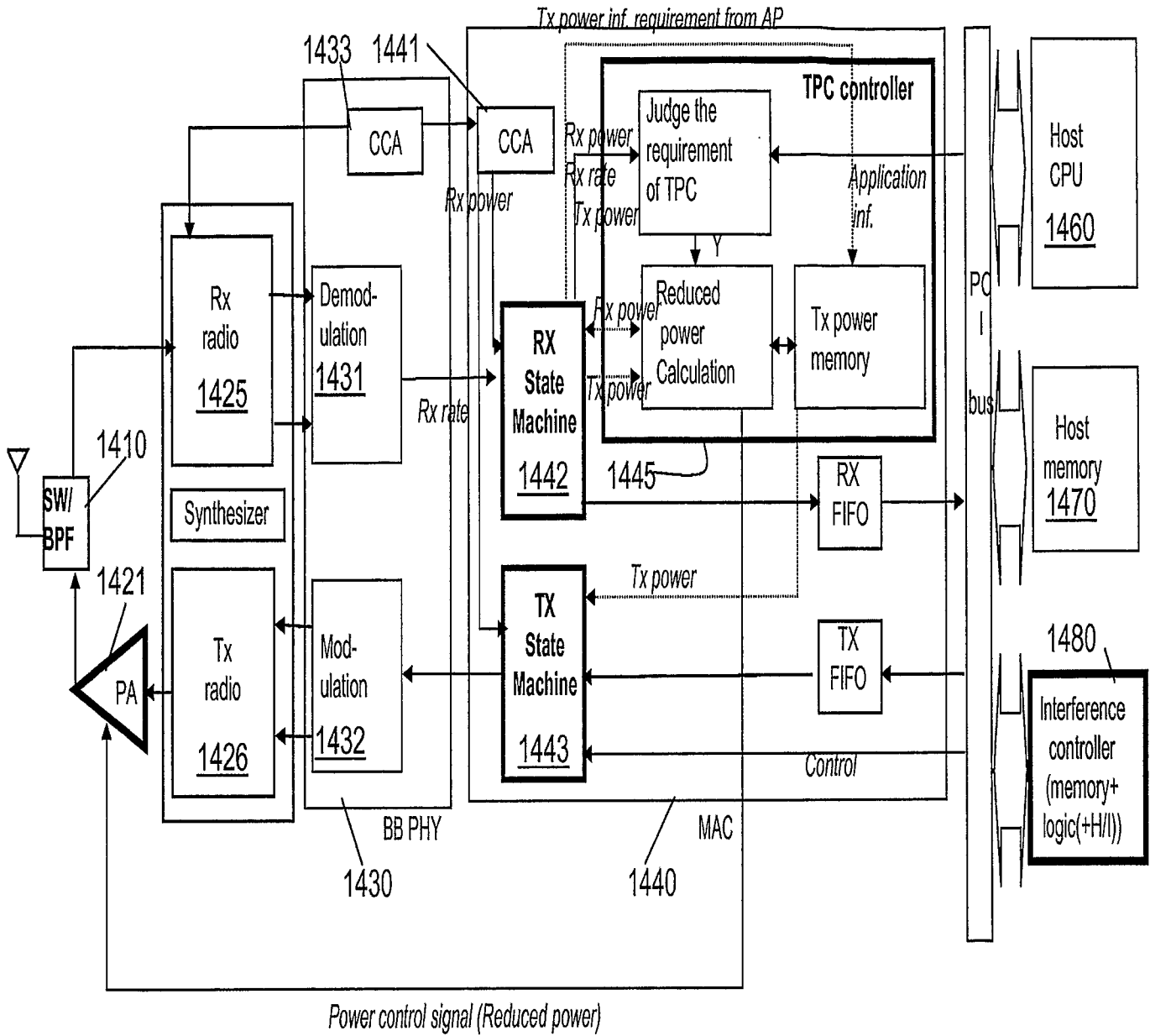
Figure 14: Block Diagram of STA for TPC
