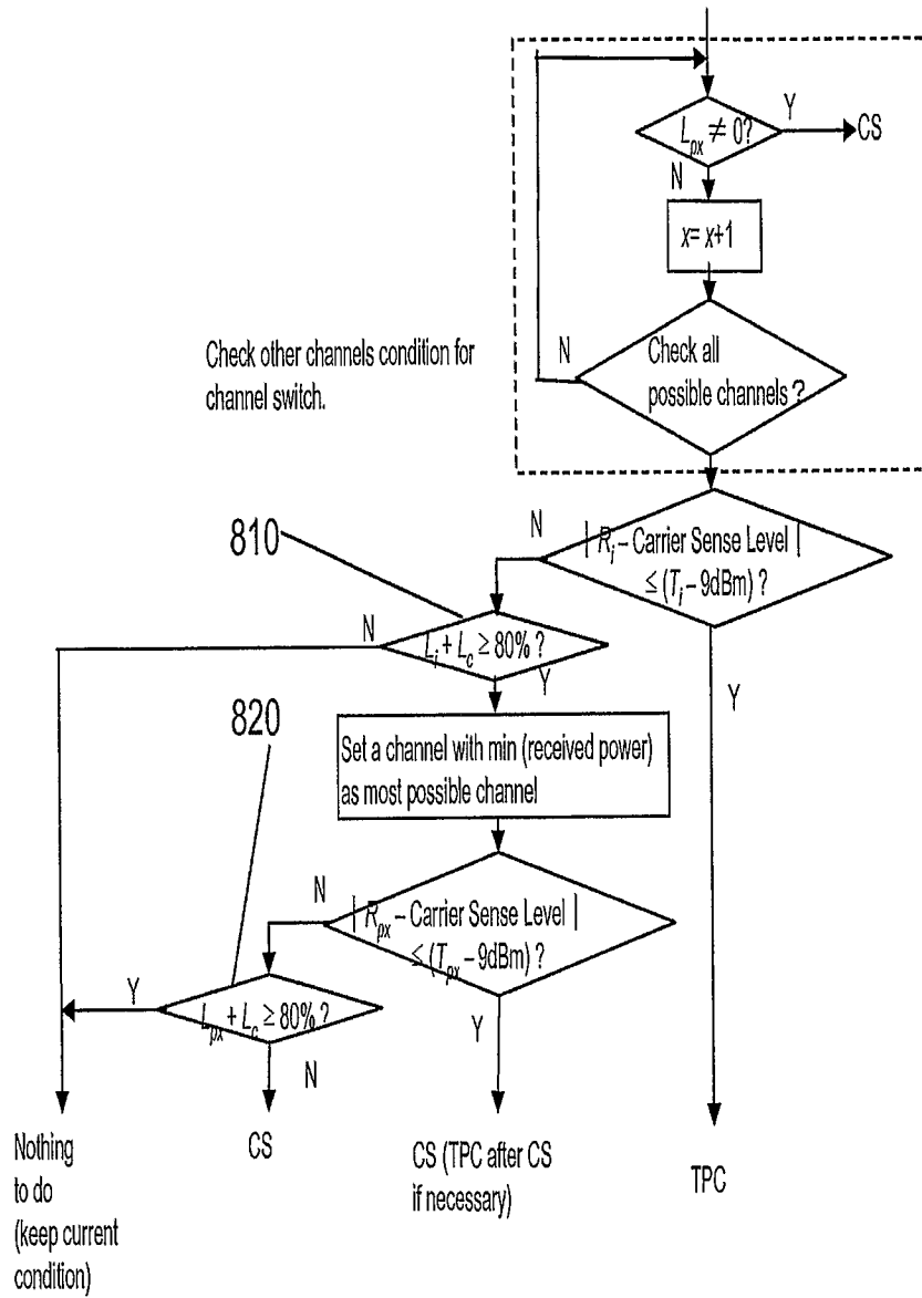
Figure 8: Advanced Selection Flow with Policy 2 ((i)-policy2-b)
