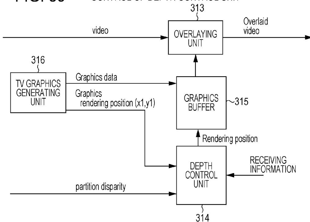
CONTROL OF DEPTH CONTROL UNIT
