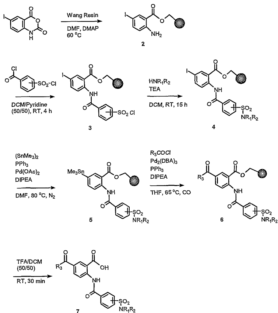
Scheme 3.1
