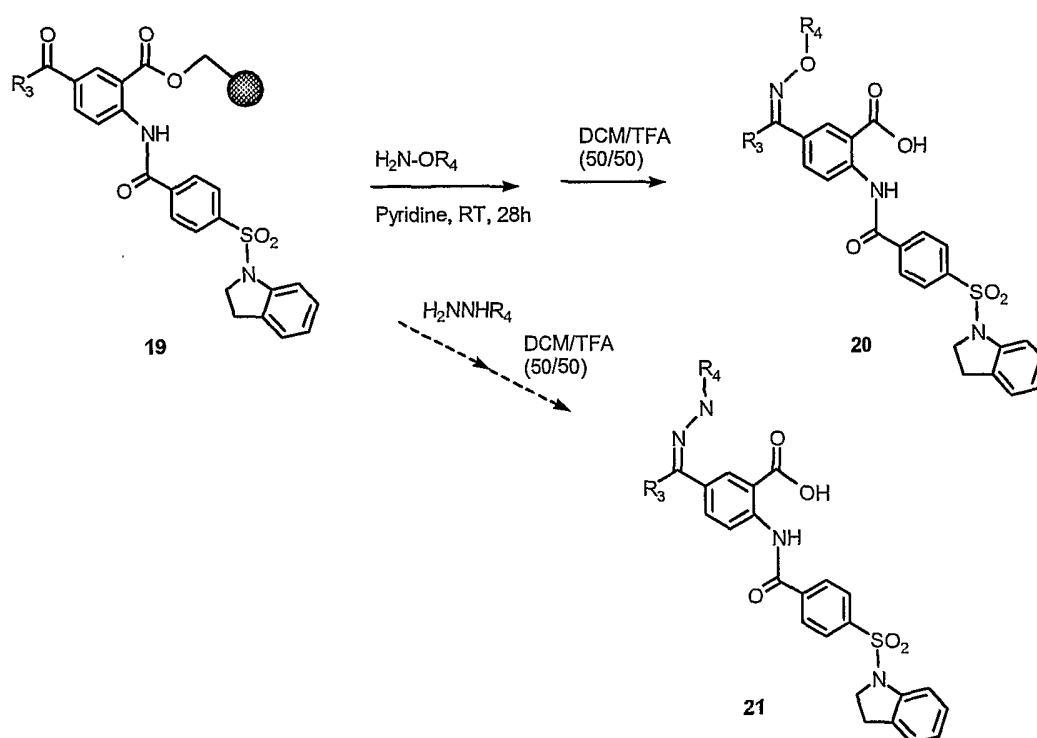
Scheme 1.26
