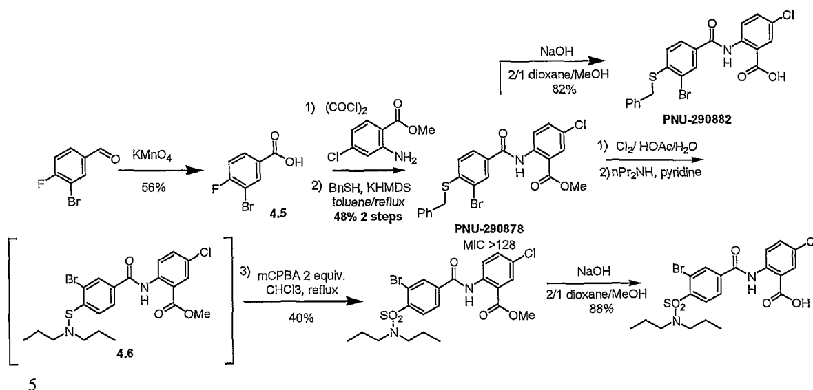
Scheme 1.13
