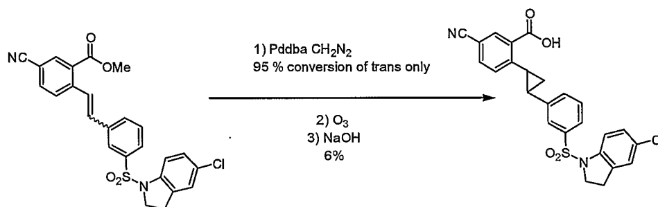
Scheme 7.3
