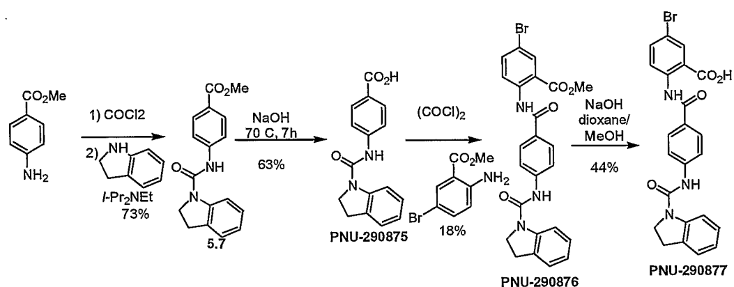
Scheme 4.1
