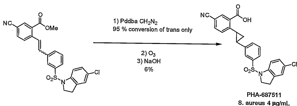
Scheme 7.1
