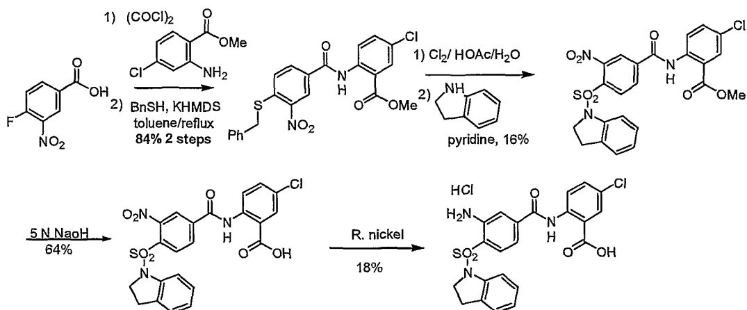
Scheme 1.11
