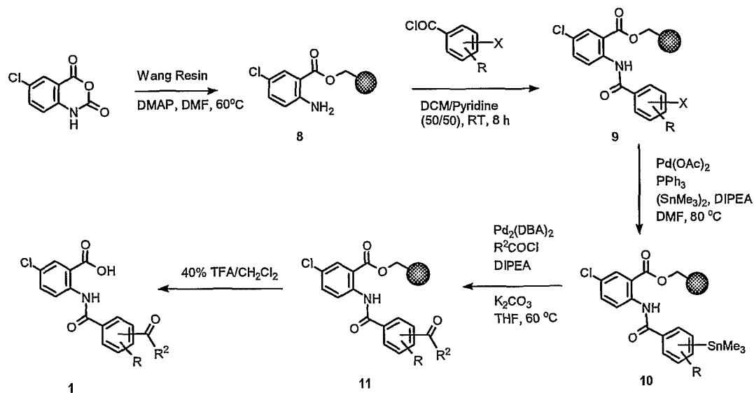
Scheme 3.2
