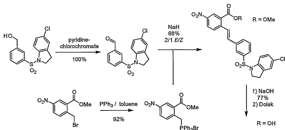
Scheme 7.3
