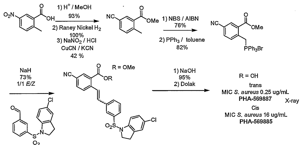
Scheme 7.4
