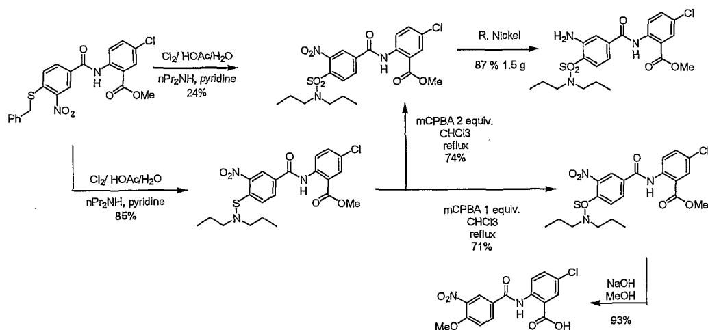
Scheme 1.11
