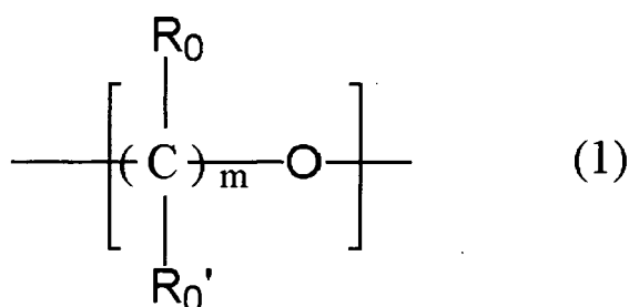
[Chemical formula 1]
