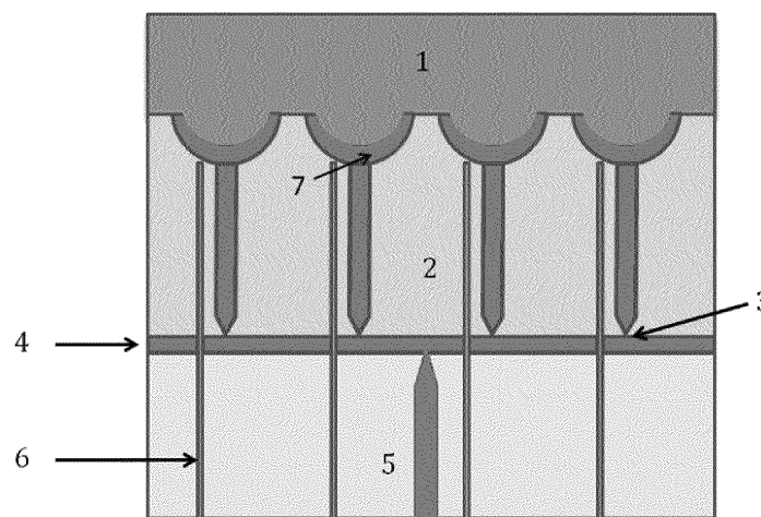
FIGURE 1 SECTION OF PLATES OF THE MOLD
