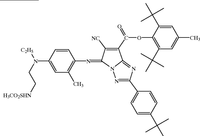
Dye compound (a)
