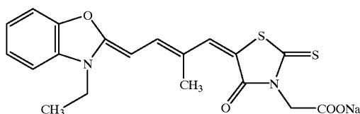
Spectrally-sensitized dye (1)
