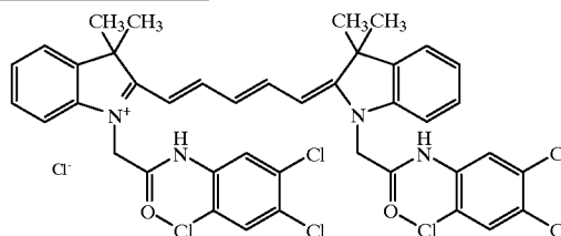
Cyanine dye compound (5)
