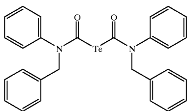
Tellurium sensitizer (2)
