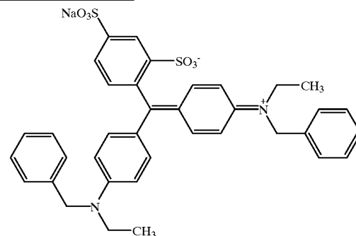
Colored dye compound (6)
