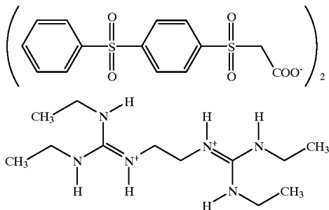
Basic precursor compound (3)
