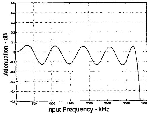
Figure 5. Decimation Filter Passband Ripple
