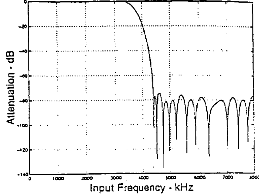
Figure 6. Interpolation Filter Response
