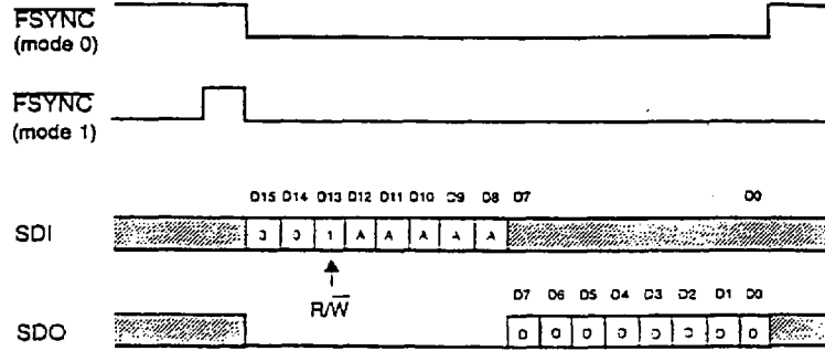
Figure 14. Secondary Communication Data Format—Read Cycle
