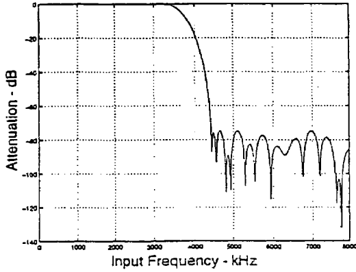
Figure 4. Decimation Filter Response
