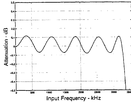
Figure 7. Interpolation Filter Passband Ripple
