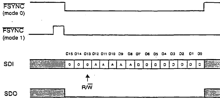
Figure 15. Secondary Communication Data Format—Write Cycle
