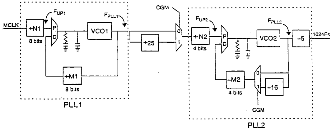
Figure 11. Clock Generation Subsystem
