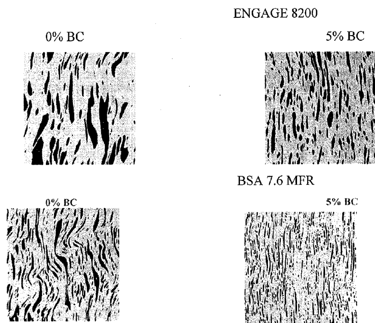
Figure 3: 20 \mu\text{m} AFM images of ENGAGE™ 8200 (Comparative Samples 5-6) and BSA7.6 (Comparative Sample 7, Example 5) dispersed in PP blends at 0 wt % active-BC and 5 wt % active-BC content.
