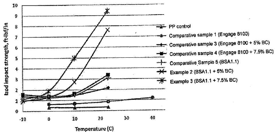
Figure 2: Effect of BC content on impact strength at different temperatures (BC is active-BC)
