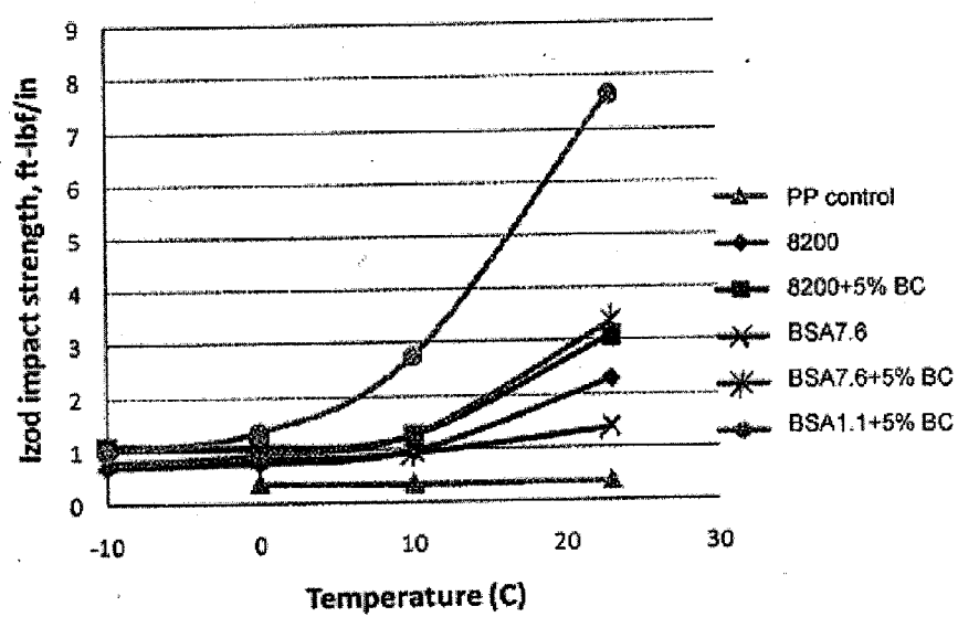
Figure 4: Effect of BC content on impact strength at different temperatures (BC is active-BC)
