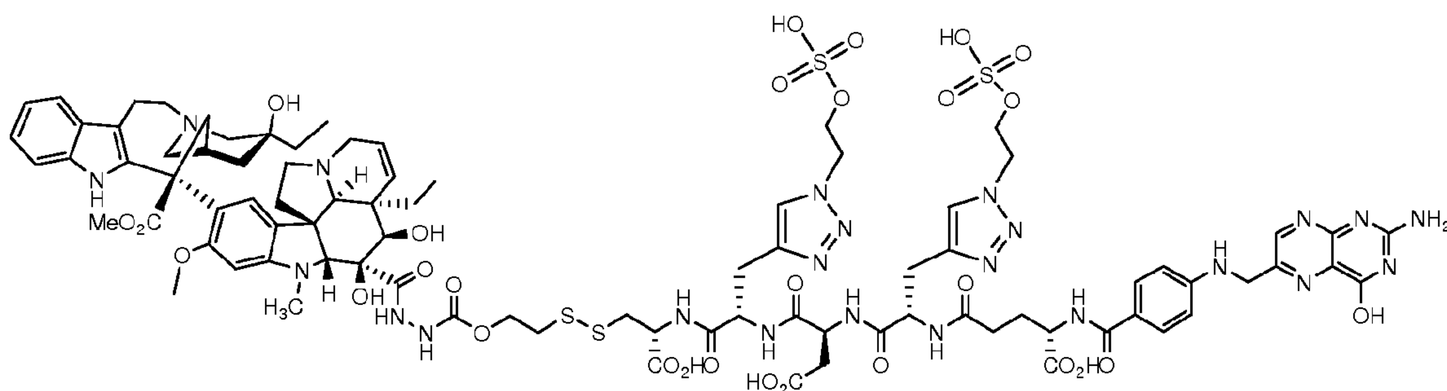
EC0428 Conjugate of DAVLBH
