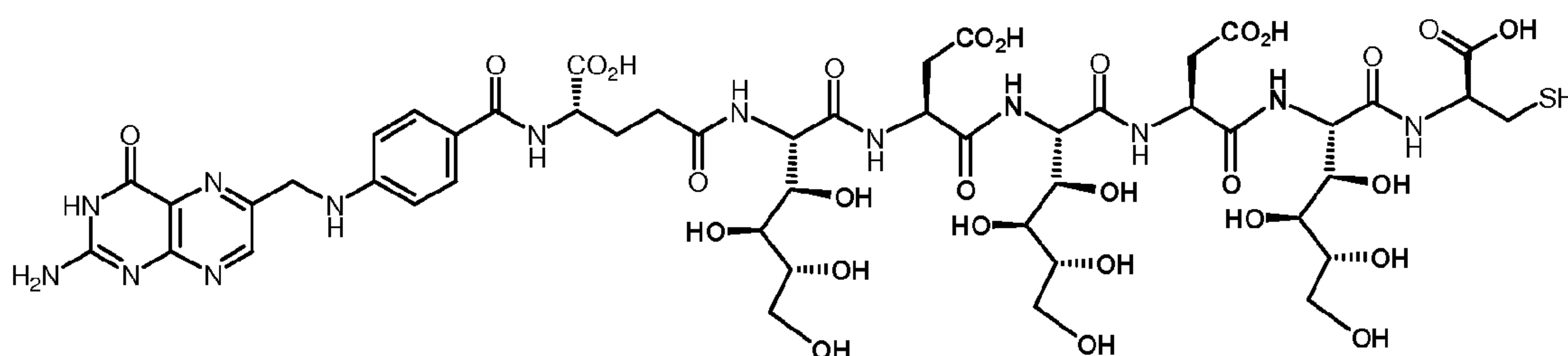
EC0261: \text{C}_{48}\text{H}_{67}\text{N}_{13}\text{O}_{28}\text{S} ; MW 1306.18; Exact Mass: 1305.39
