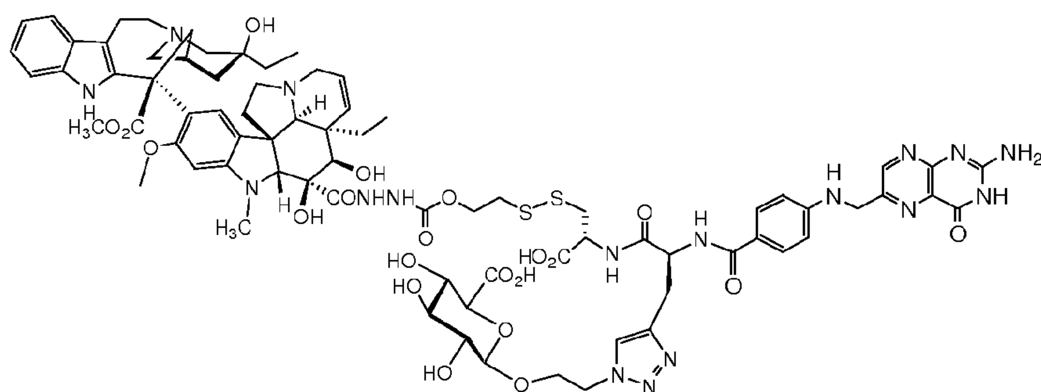
Conjugate of DAVLBH.
