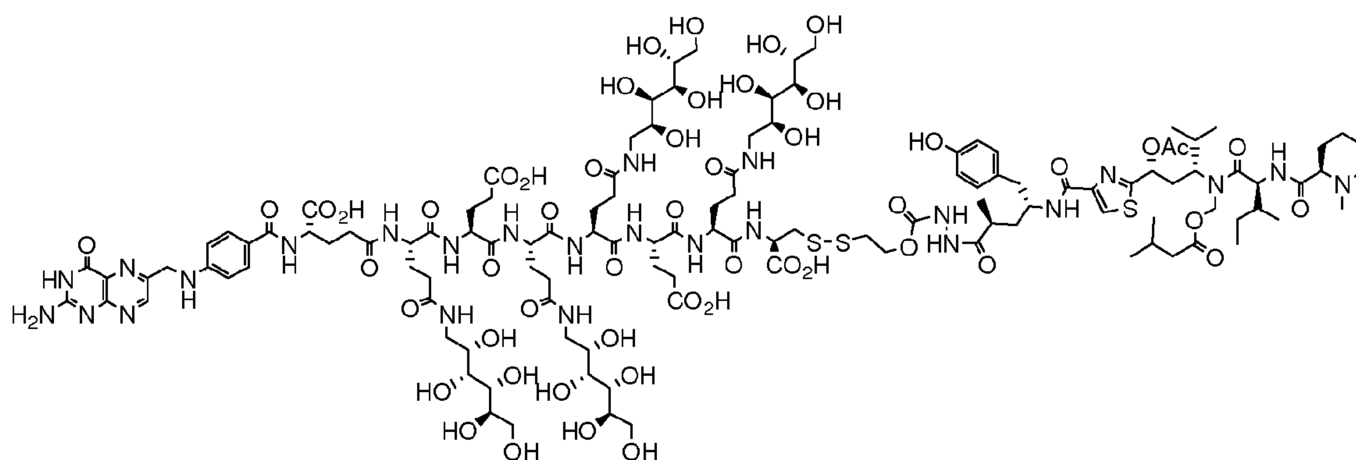
EC0533 Conjugate of Tubulysin
