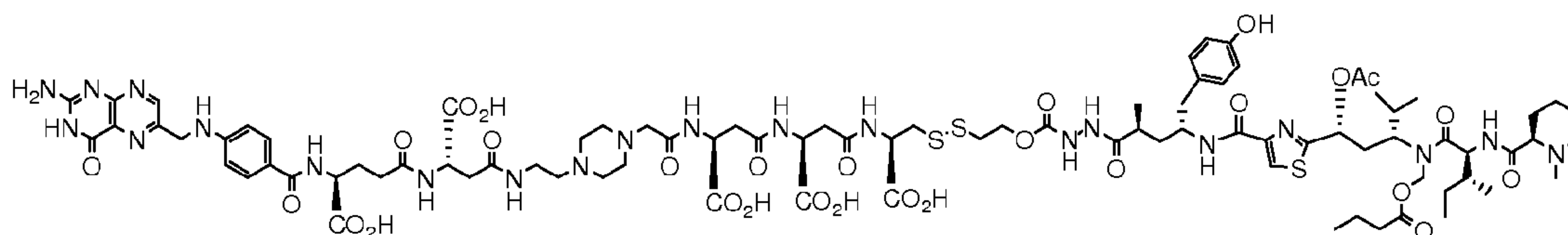
EC0444 Conjugate of Tubulysin
