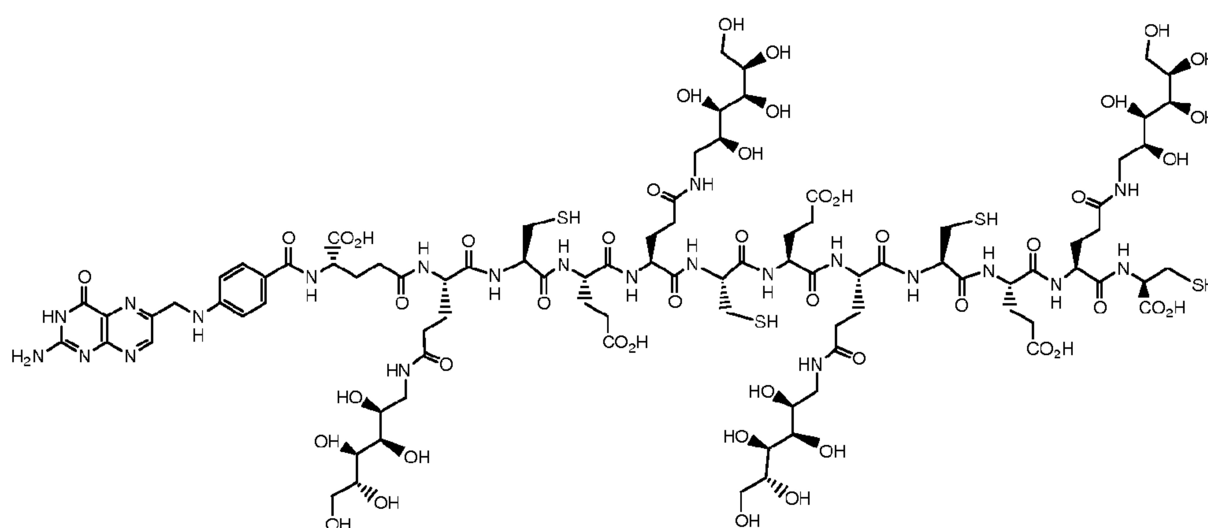
5 EC0613 Multidrug intermediate for three drugs. C_{90}H_{140}N_{22}O_{47}S_4 , MW 2410.45, Exact Mass: 2408.81
