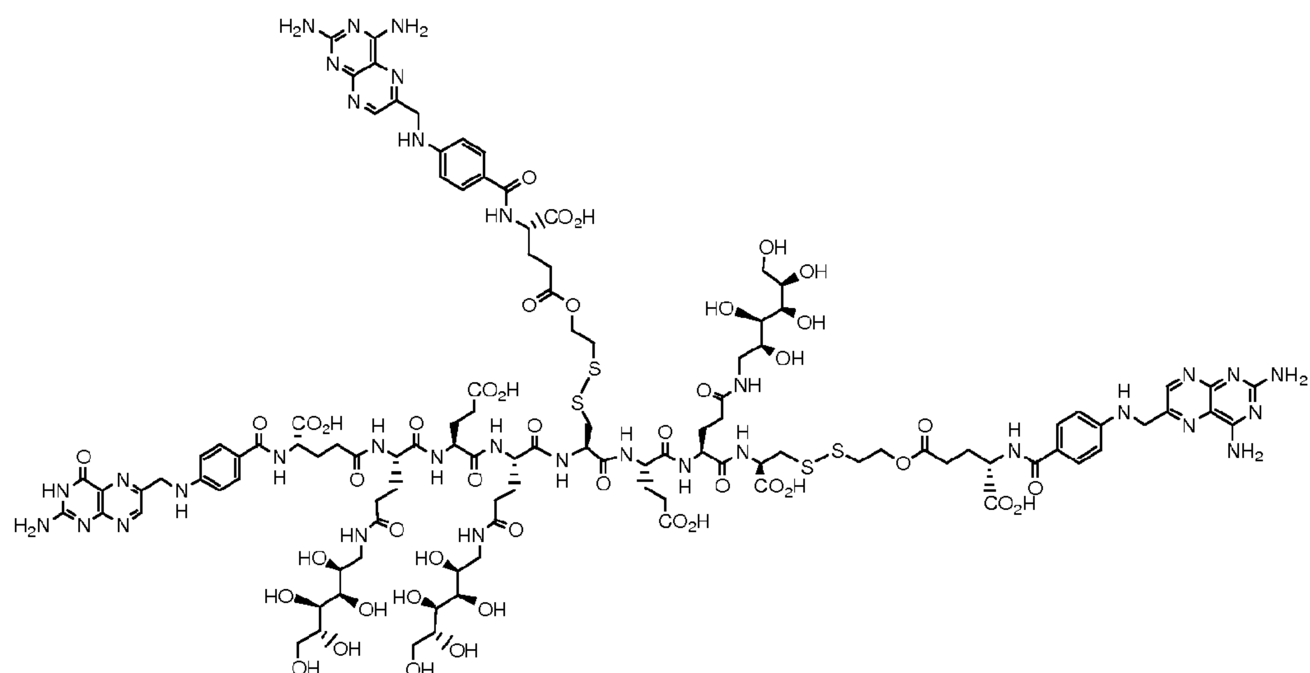
EC0647 Bis aminopterine conjugate. C 110 H 147 N 33 O 45 S 4 , MW, 2779.80, Exact Mass: 2777.9112, m/z: 2778.91 (100.0%), 2777.91 (74.4%), 2779.92 (62.2%)
