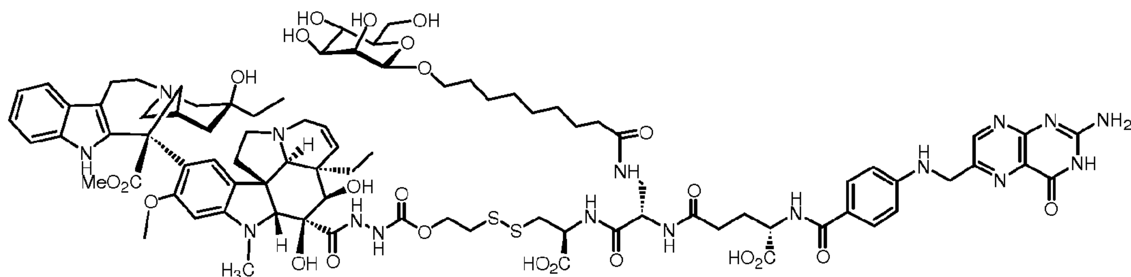
Conjugate of DAVLBH including a \beta -alkyl mannopyranoside.
