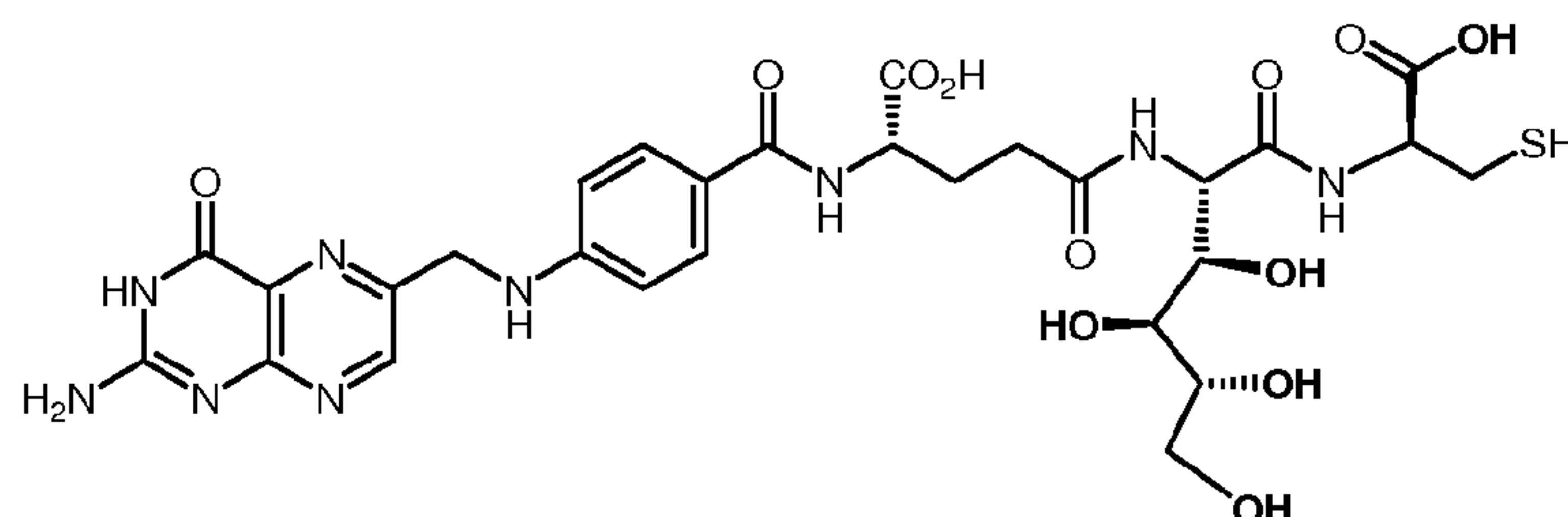
EC0233: \text{C}_{28}\text{H}_{35}\text{N}_9\text{O}_{12}\text{S} ; MW 721.70; Exact Mass: 721.21
