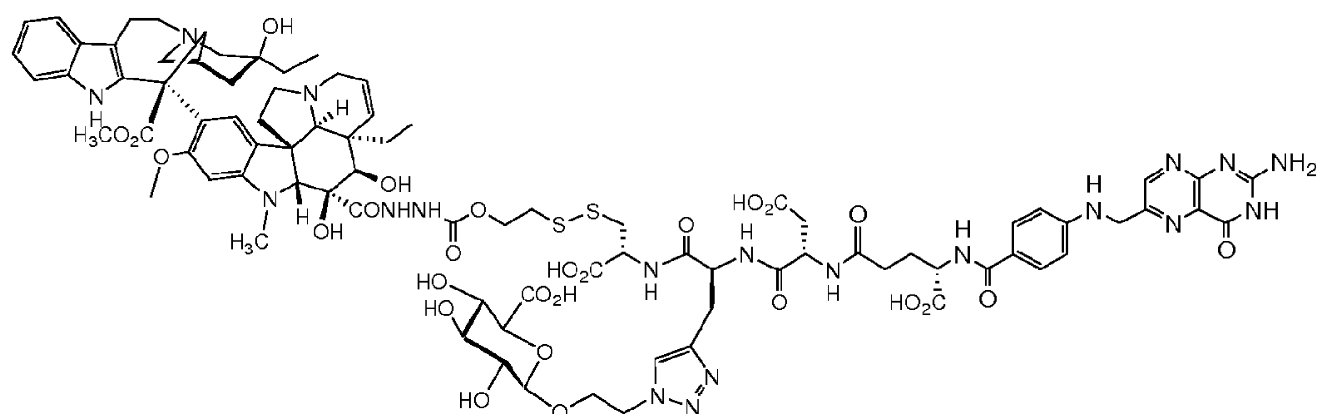
Conjugate of DAVLBH.
