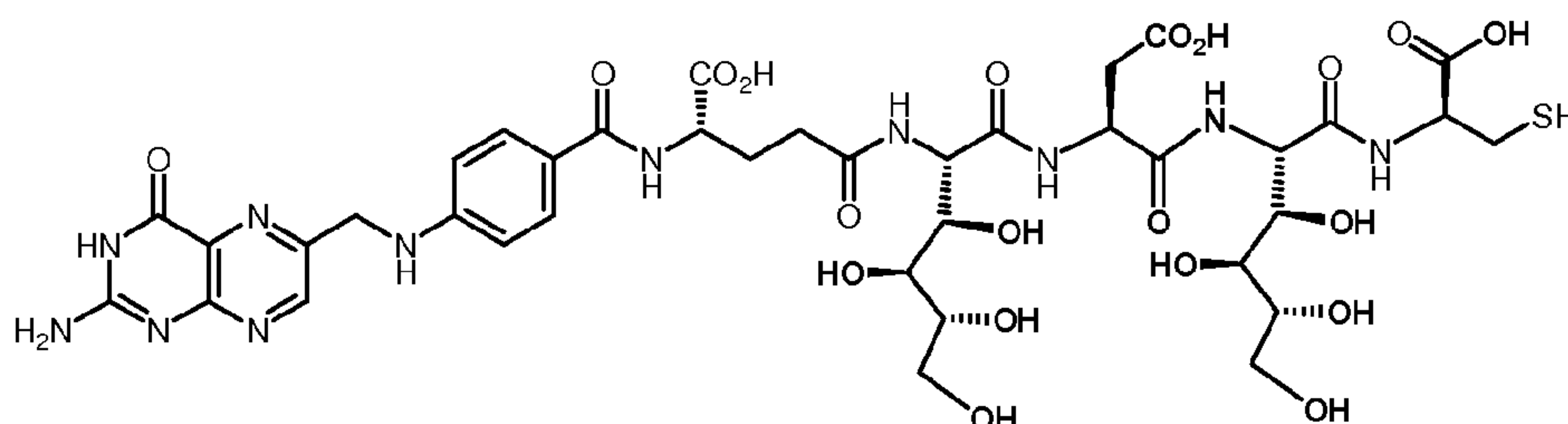
EC0244: \text{C}_{38}\text{H}_{51}\text{N}_{11}\text{O}_{20}\text{S} ; MW 1013.94; Exact Mass: 1013.30
