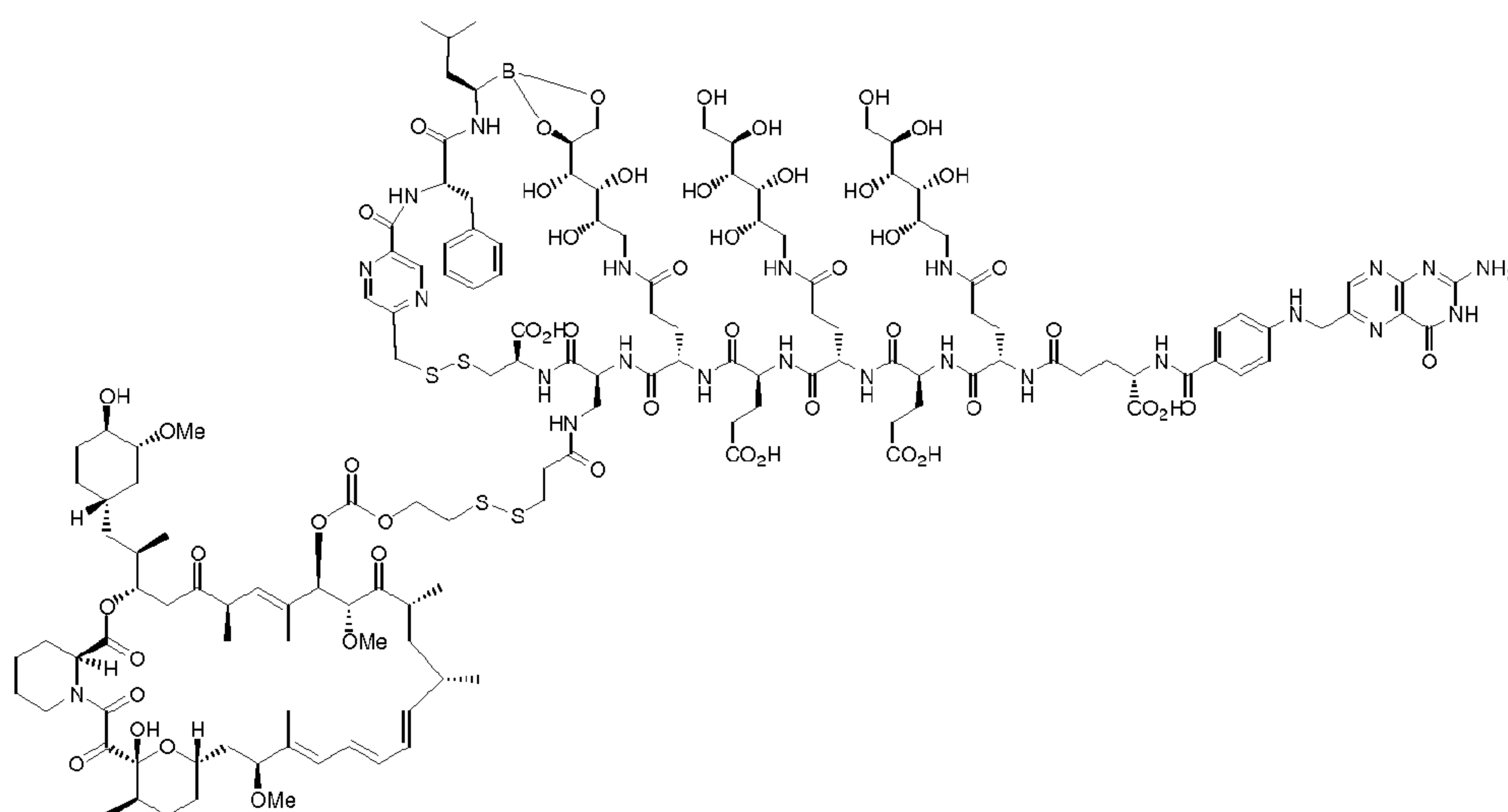
EC0563 Conjugate of Bortezomib and Rapamycin.
