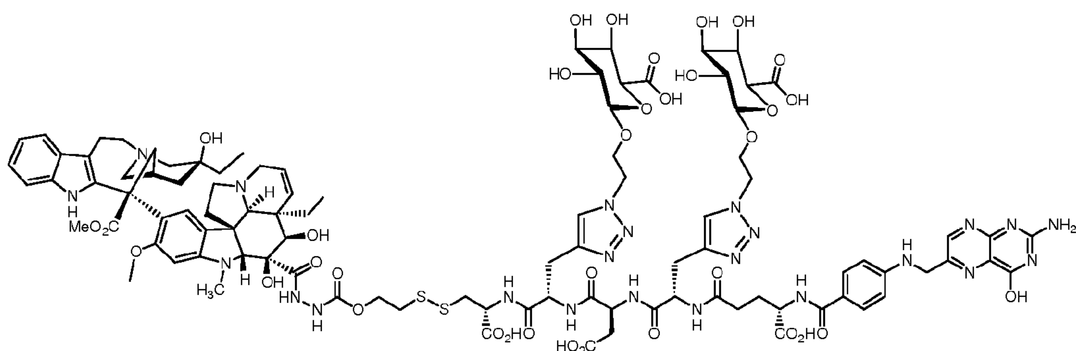
EC0423 Conjugate of DAVLBH. Prepared by Huisgen cyclization; C 98 H 123 N 23 O 35 S 2 , C, 52.38; H, 5.52; N, 14.34; O, 24.92; S, 2.85, MW 2247.29, Exact Mass: 2245.80
