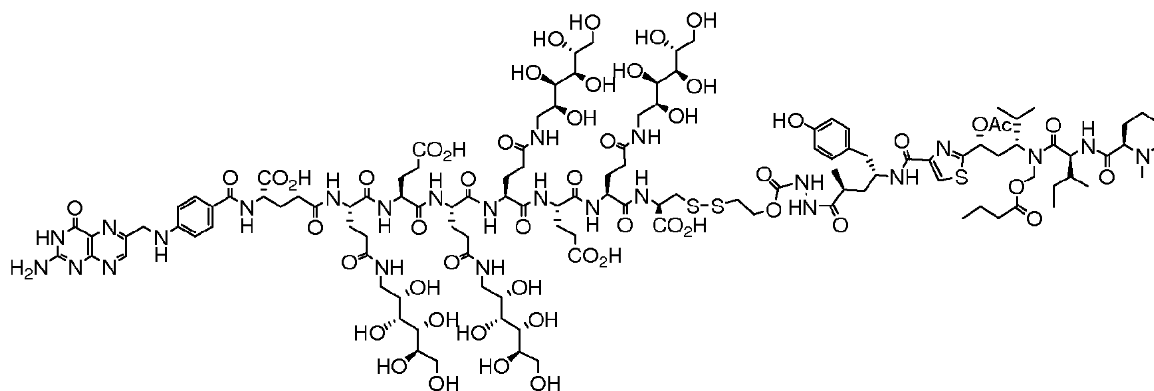
EC0530 Conjugate of Tubulysin
