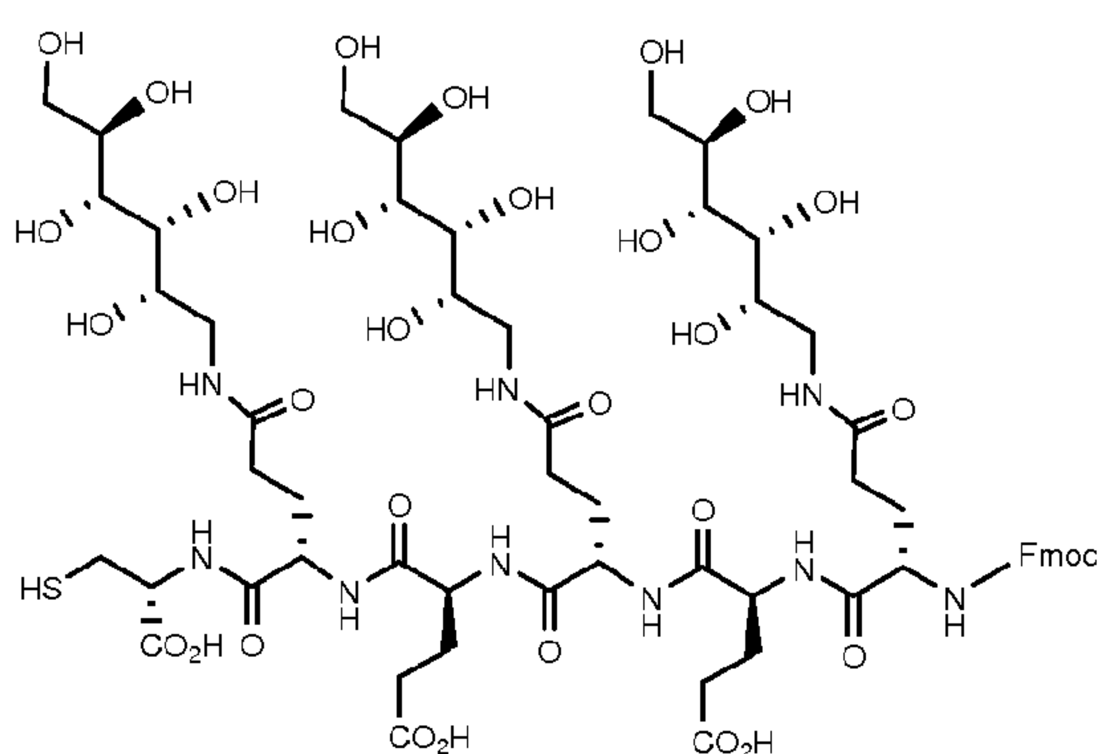
EC0680 Conjugate of Everolimus and 4-[(3-Bromophenyl)amino]-6-hydrazino-pyrido[3,4-d]pyrimidine. C 143 H 206 BrN 25 O 54 S 4 , MW 3347.47, Exact Mass: 3344.22
