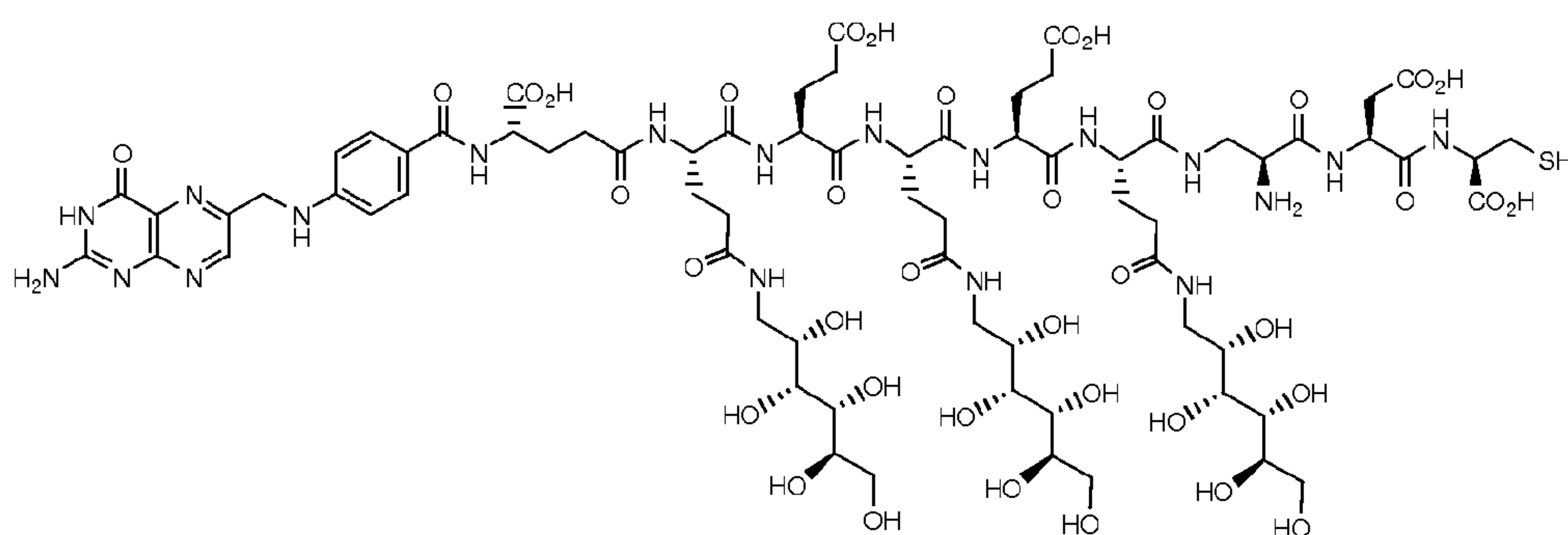
EC0536 Conjugate intermediate
