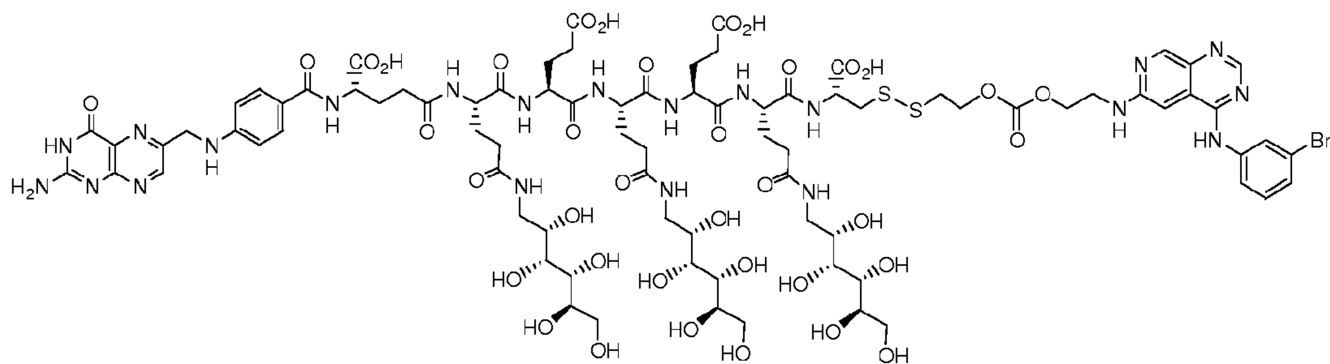
EC0631 Conjugate of the tyrosine kinase inhibitor 4-[(3-bromophenyl)amino]-6-[(2-hydroxyethyl-amino)-pyrido[3,4-d]pyrimidine, C 83 H 114 BrN 21 O 37 S 2 , MW 2141.95, Exact Mass: 2139.63
