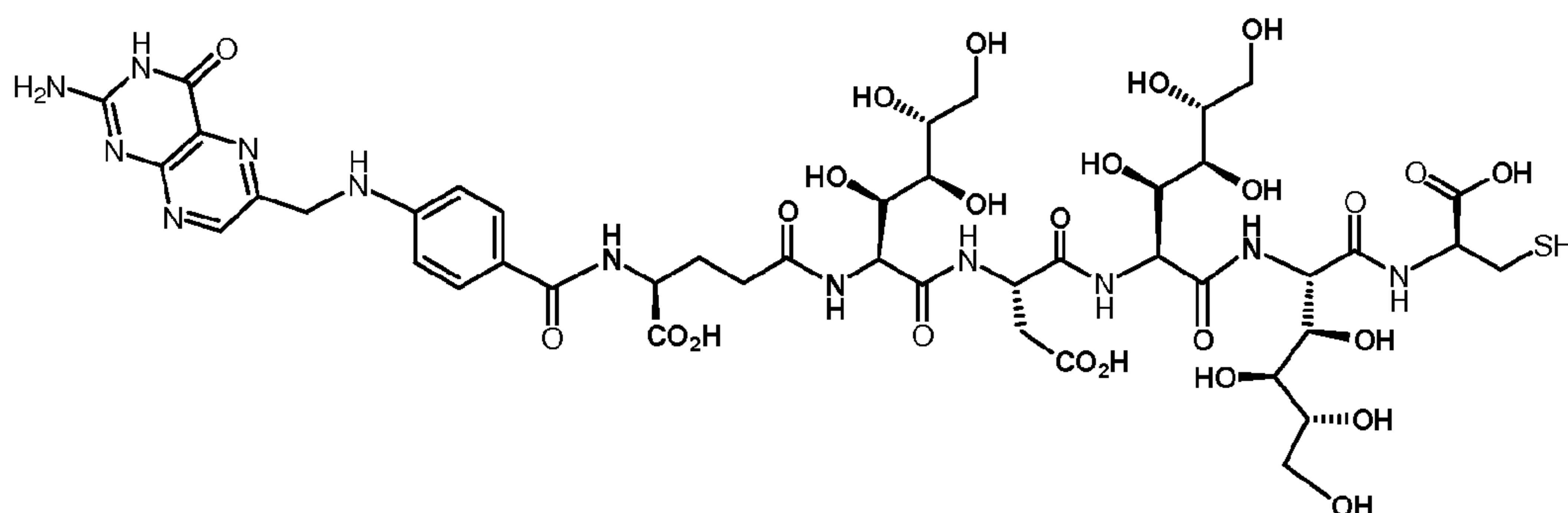
EC0257: \text{C}_{44}\text{H}_{62}\text{N}_{12}\text{O}_{25}\text{S} ; MW 1191.09; Exact Mass: 1190.37
