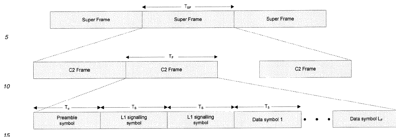
Figure 29: C2 Frame Structure
