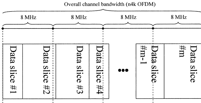
Figure 22: Data slicing in the overall channel bandwidth (32 MHz channel example)
