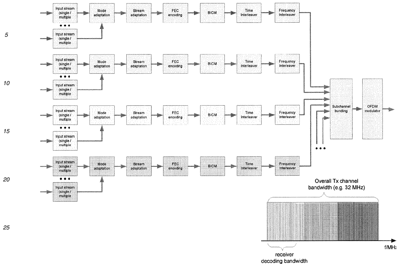
Figure 35: Building the overall OFDM signal
