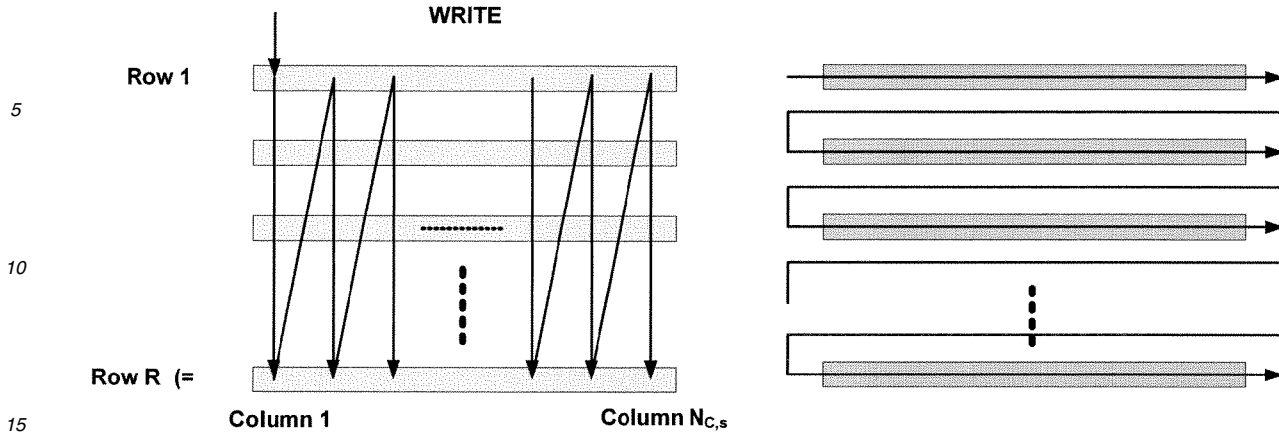
Figure 27: Time Interleaver
