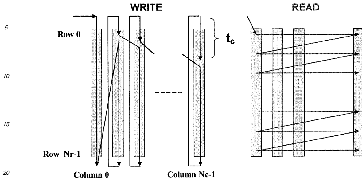
Figure 26: Bit Interleaving scheme
