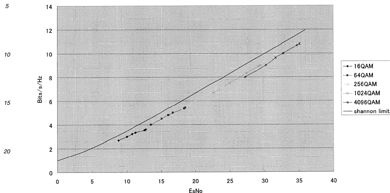
EsNo vs Bits/s/Hz (from RHS, R9/10, R8/9, R5/6, R4/5, R3/4, R2/3)
