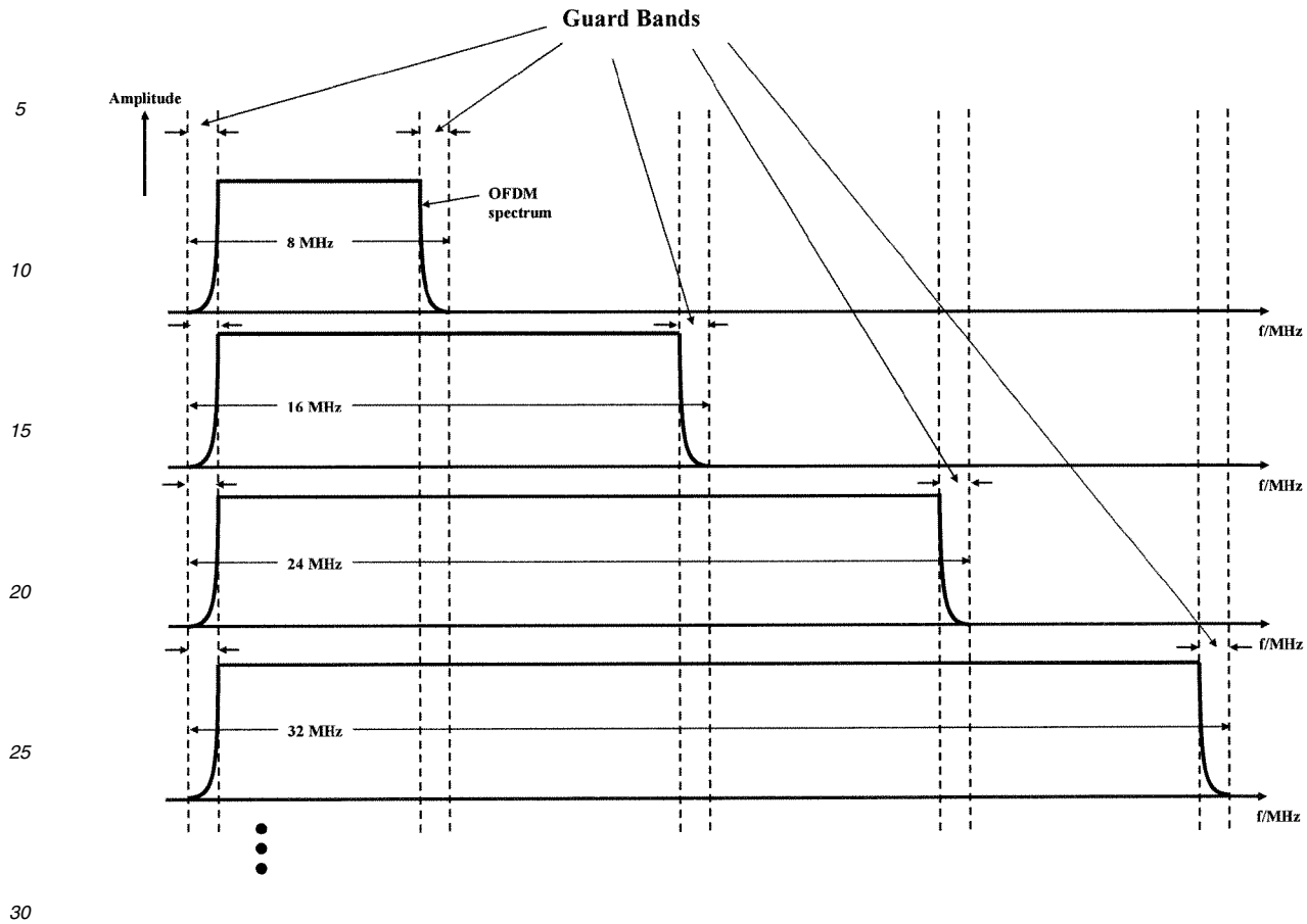
Figure 19: Example bandwidths of the proposed DVB-C2 OFDM channels
