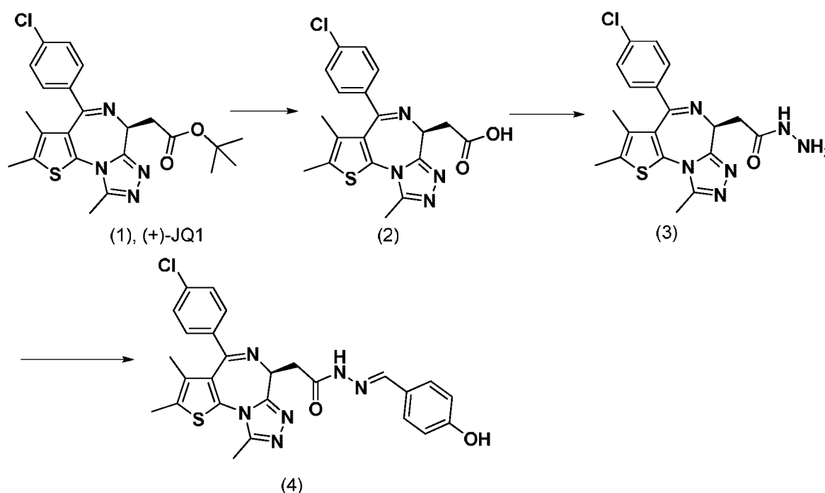
Scheme S3. Synthesis of hydrazine derivatives.
