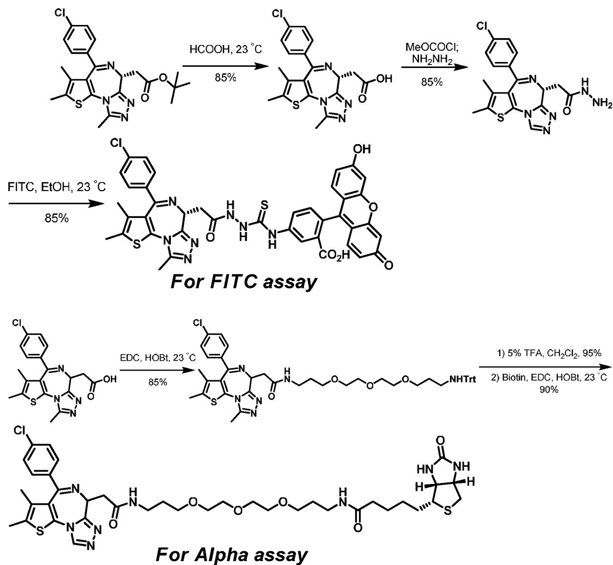
Scheme S4. Synthesis of derivatives useful as probes.
