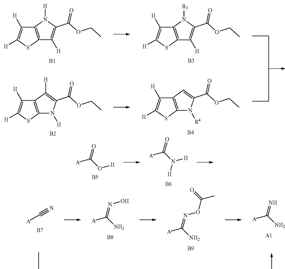
Scheme B
