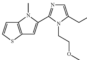
101 5-[5-ethyl-1-(2-methoxyethyl)imidazol-2-yl]-4-methyl-thieno[3,2-b]pyrrole
