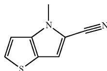
Intermediate 5: 4-Methylthieno[3,2-b]pyrrole-5-carbonitrile
