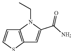
Intermediate 4: 4-Ethylthieno[3,2-b]pyrrole-5-carboxamide
