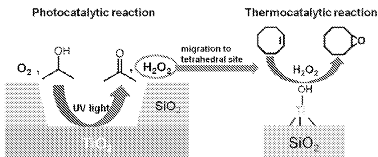
Scheme 1: Combined photo- and thermo-catalytic system for hydrogen peroxide production on SiO_2@TiO_2 (left) and subsequent consumption via alkene epoxidation on Ti- SiO_2 (right). Note that the Ti- SiO_2 site may exist on the surface of the SiO_2@TiO_2 material, as in Ti- SiO_2@TiO_2 .
