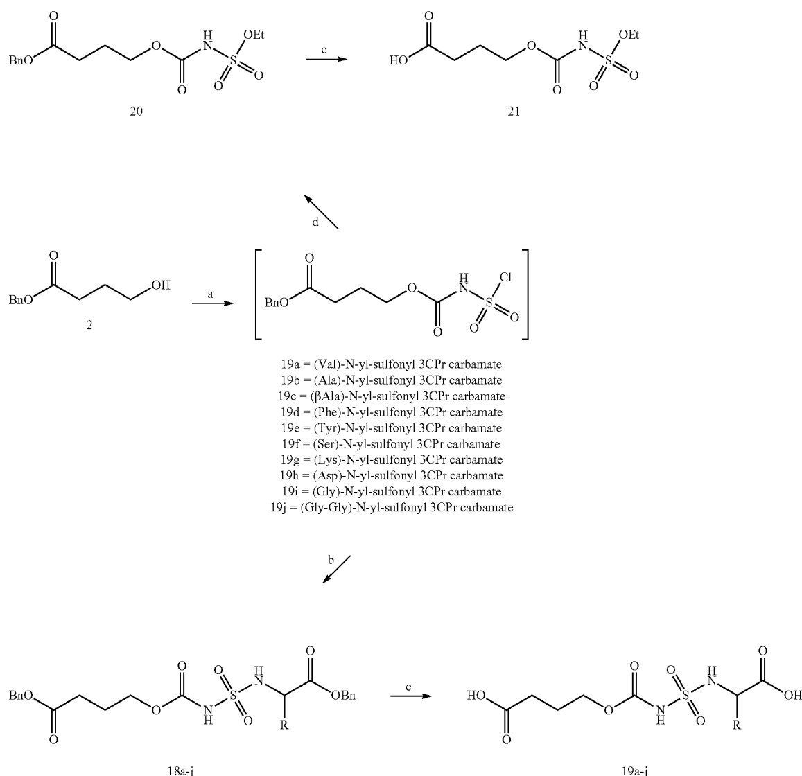
Scheme 6.
