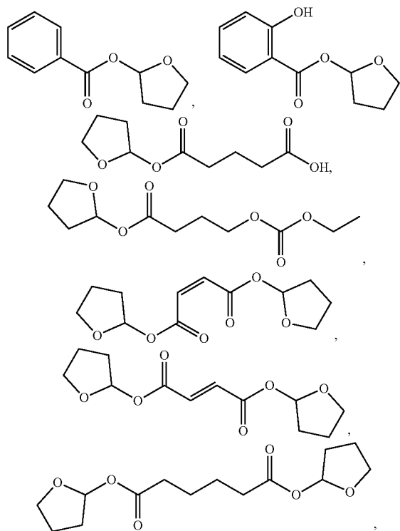
Formula III
