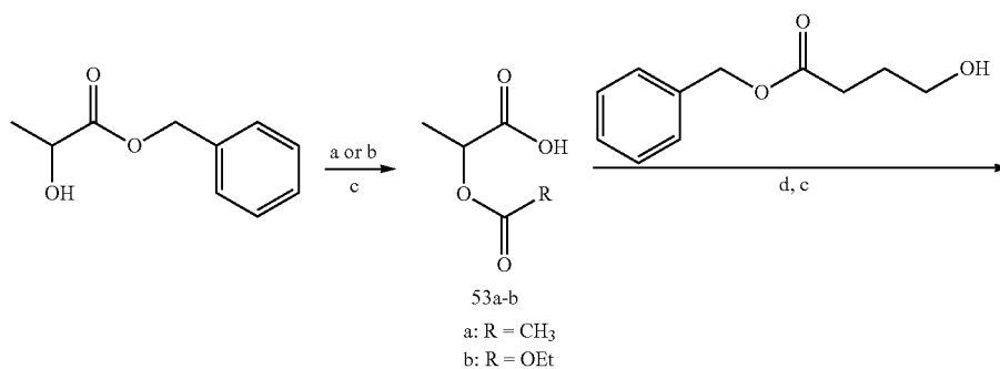
Scheme 21. (a) \text{Ac}_2\text{O} , DMAP, DCM; (b) Ethyl chloroformate, DMAP, DIPEA, DCM; (c) Pd/C, EtOH, (d) 2, DCC, DMAP, DCM
