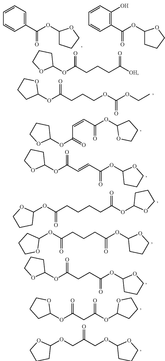
Formula III
