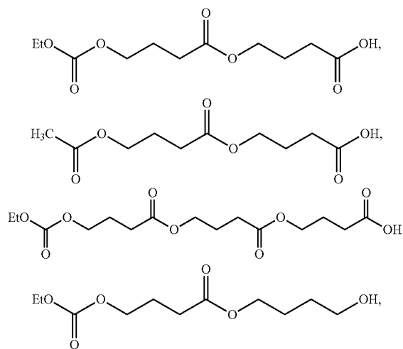
Formula I
