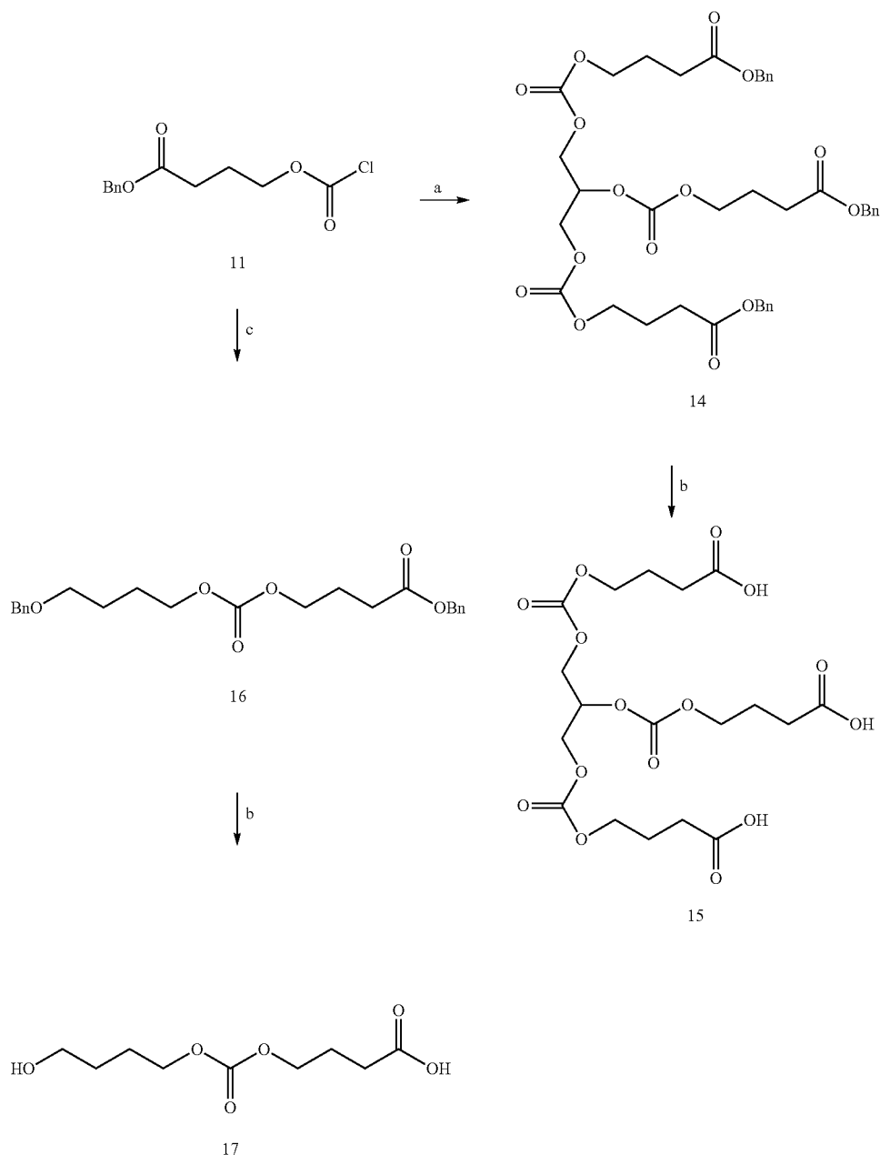
Scheme 5.
