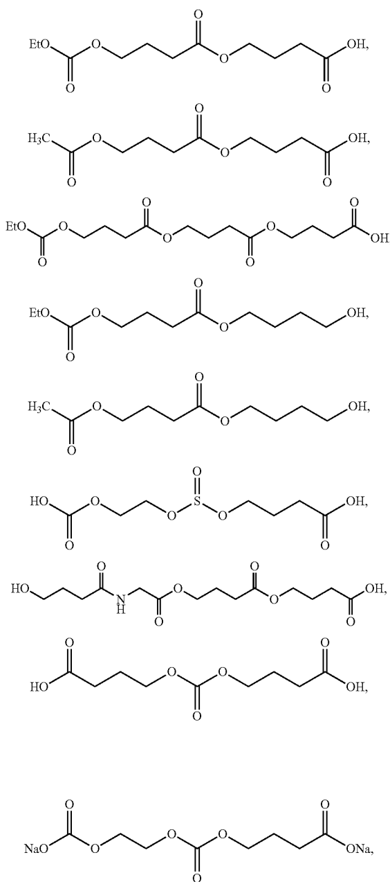
Formula I
