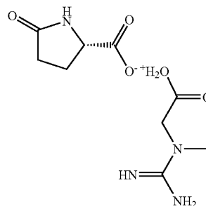
(2-(1-methylguanidino)acetyl)oxonium pyroglutamate
