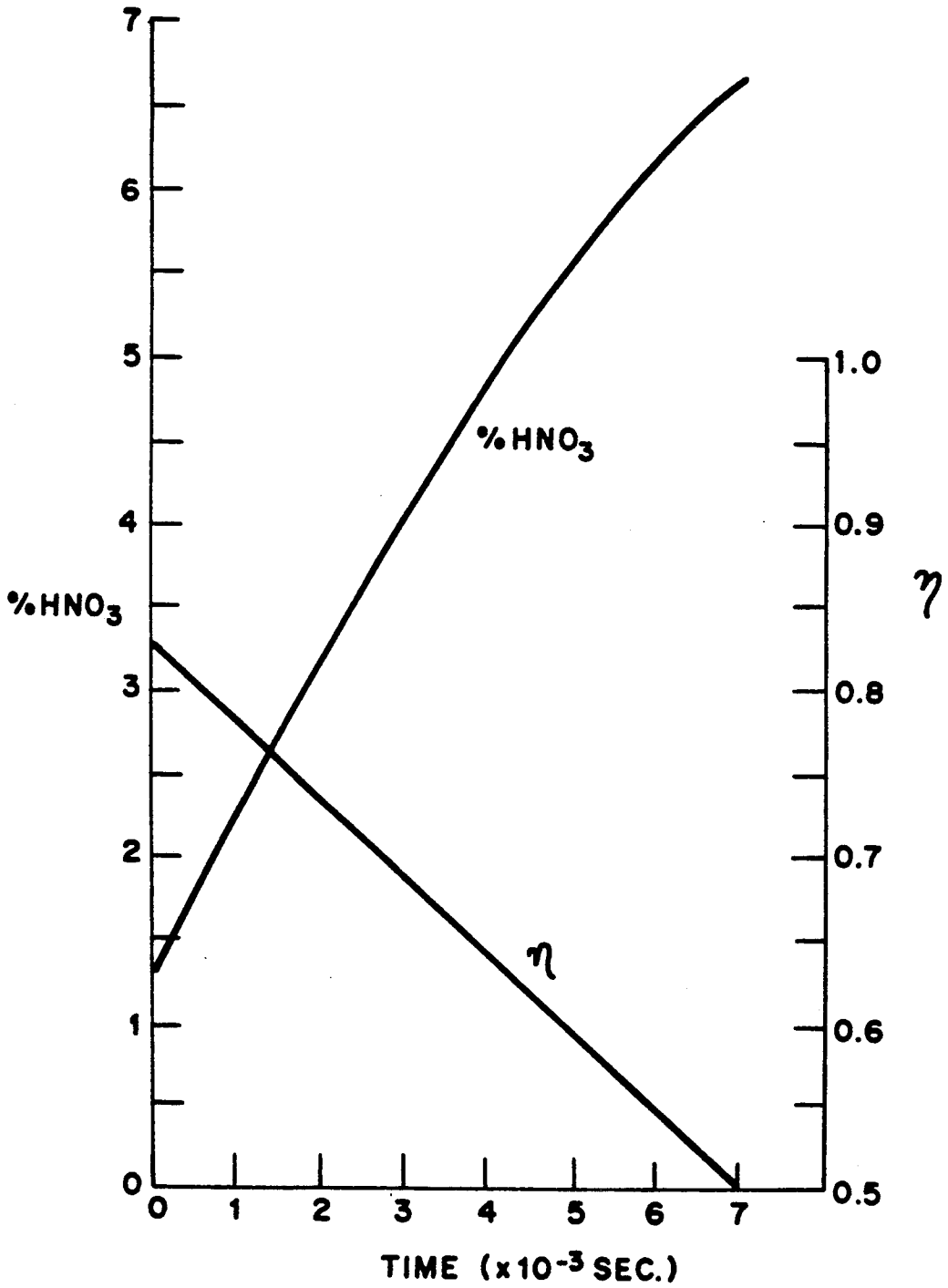
FIG. 3 GENERATION OF HNO 3 FROM KNO 3
