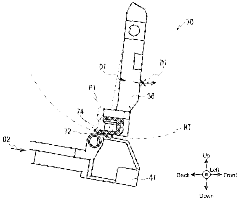
[Switching Lever Extracting State]
