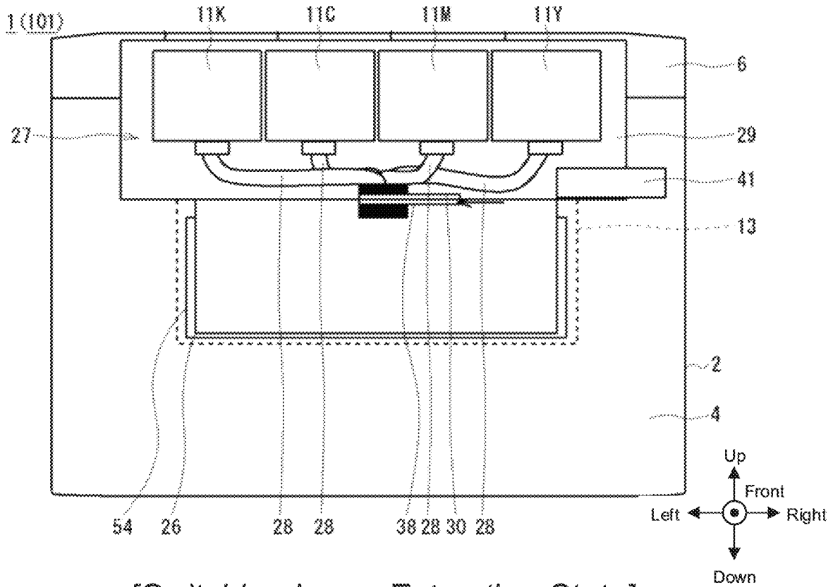
[Switching Lever Extracting State]
