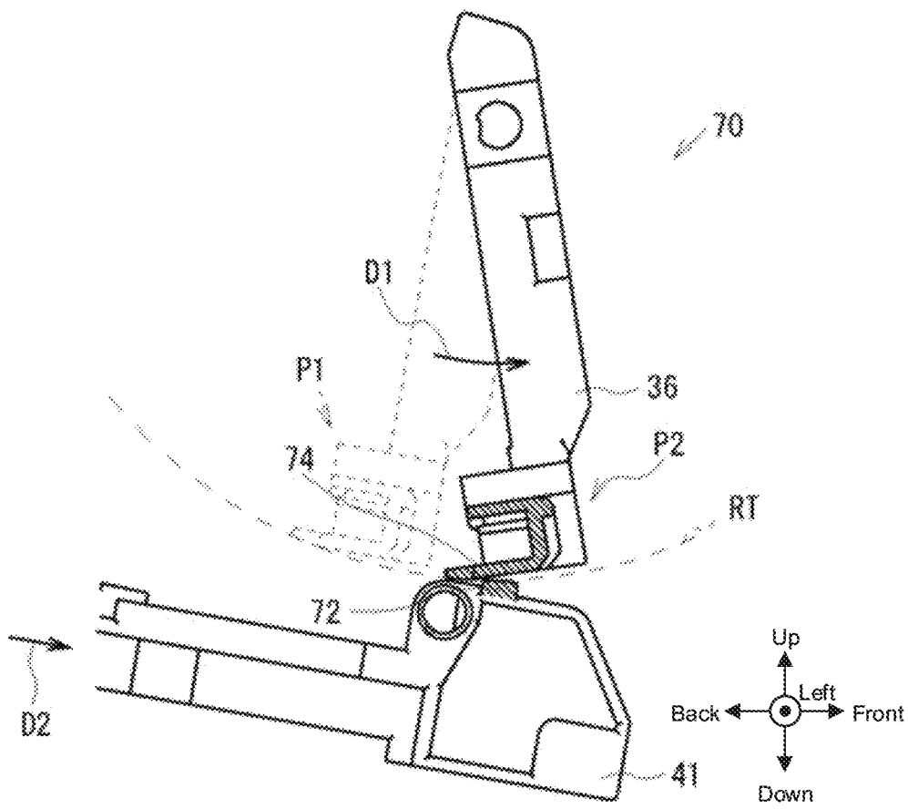
[Switching Lever Extracted State]
