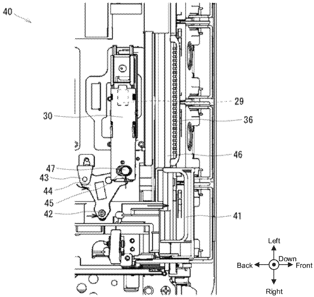
[Switching Lever Extracting State]
