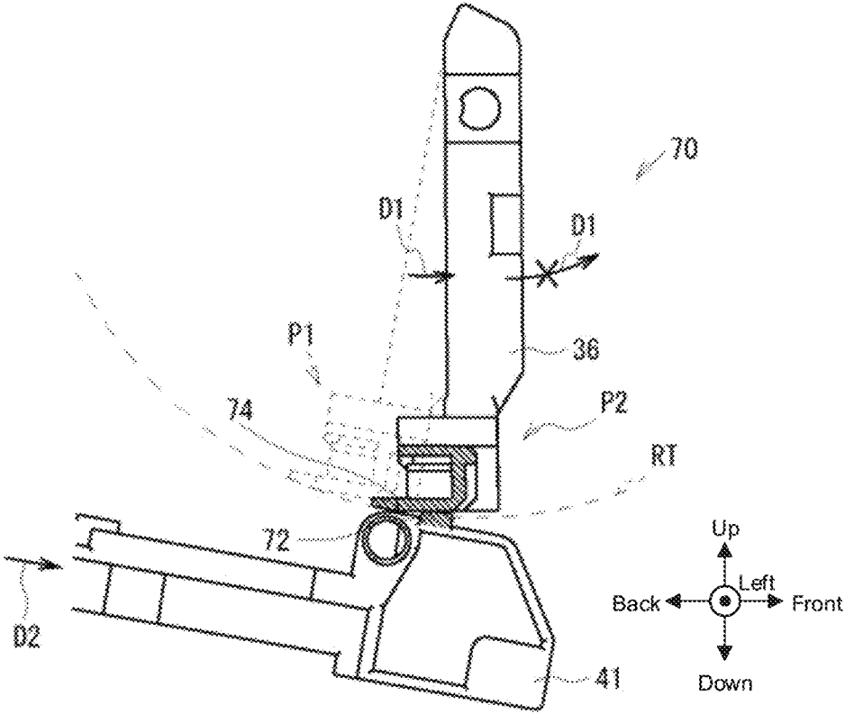
[Switching Lever Extracting State]
