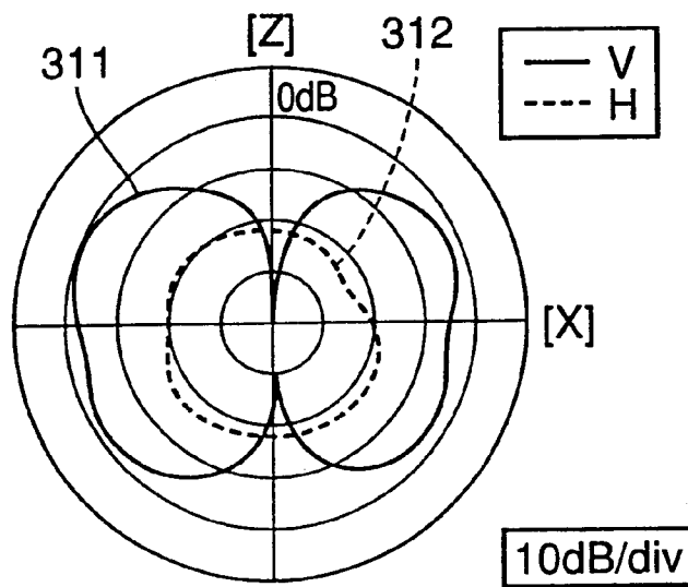
FIG. 14 PRIOR ART
