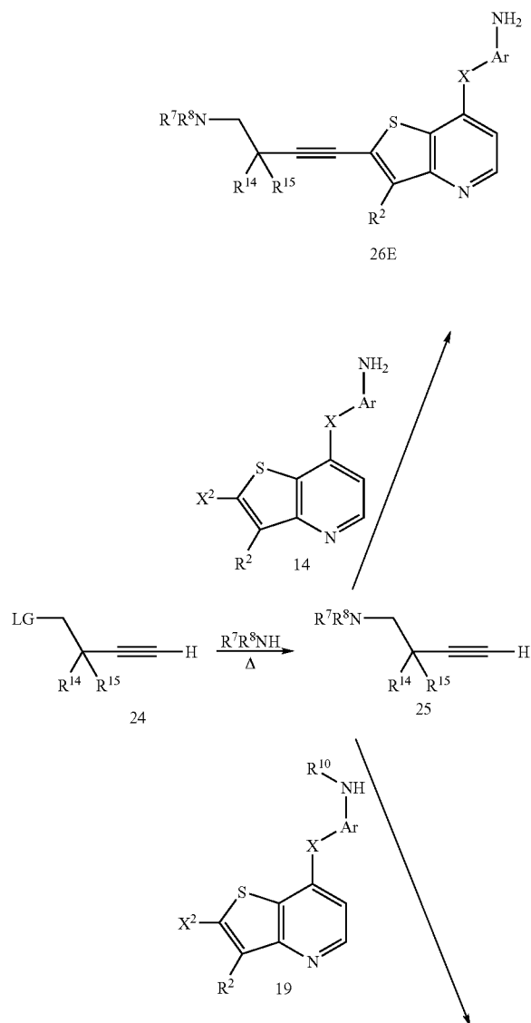
Scheme 11
