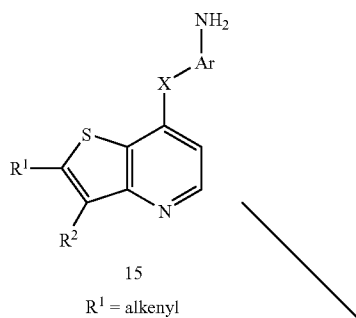
Scheme 14
