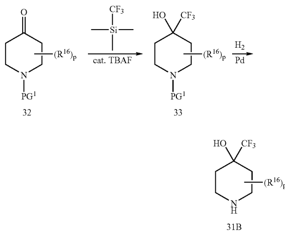
Scheme 13
