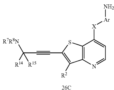
Scheme 10
