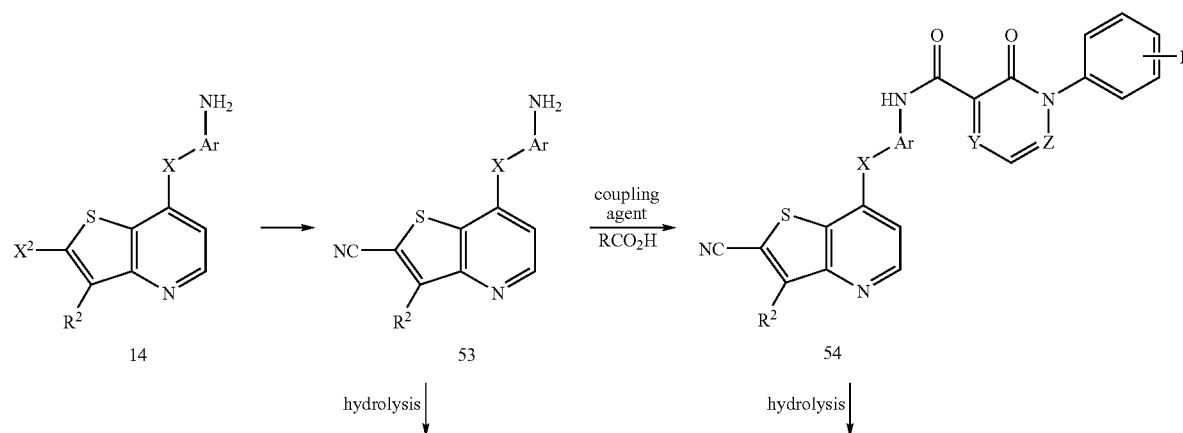
Scheme 19
