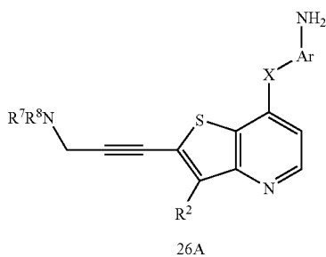
Scheme 9
