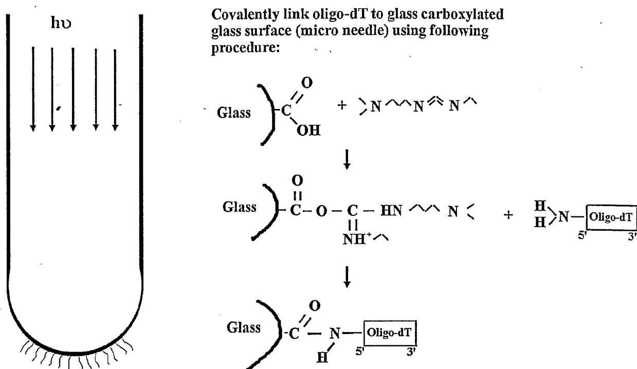
Fig. 4 Design of micro glass/quartz needle for immobilizing target sequences and probe in hybridization analysis.
