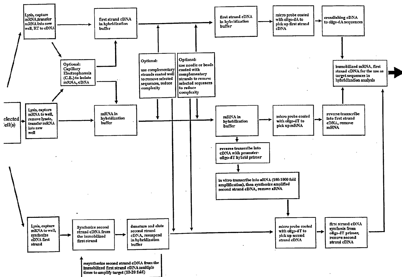
Fig. 3 Procedures in preparing and immobilizing target sequences of mRNA, cDNA.
