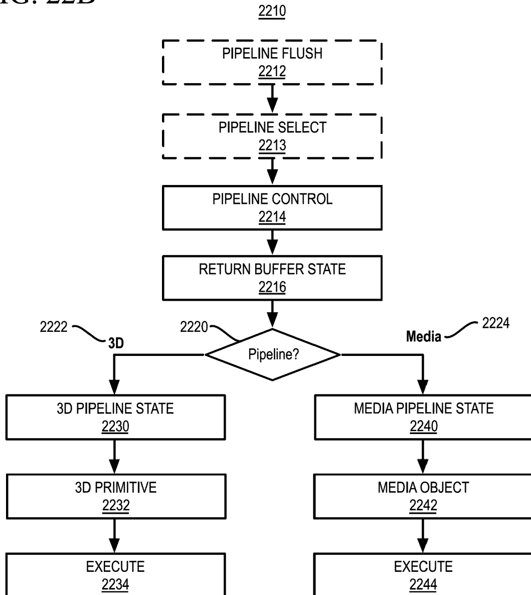
FIG. 22B GRAPHICS PROCESSOR COMMAND SEQUENCE
