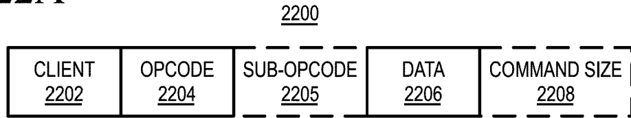
FIG. 22A GRAPHICS PROCESSOR COMMAND FORMAT
