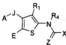
Formula (V);
