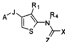
Formula (III);
