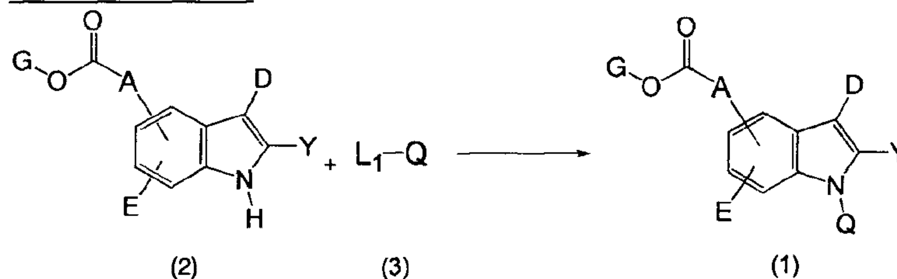
Reaction Scheme 1
