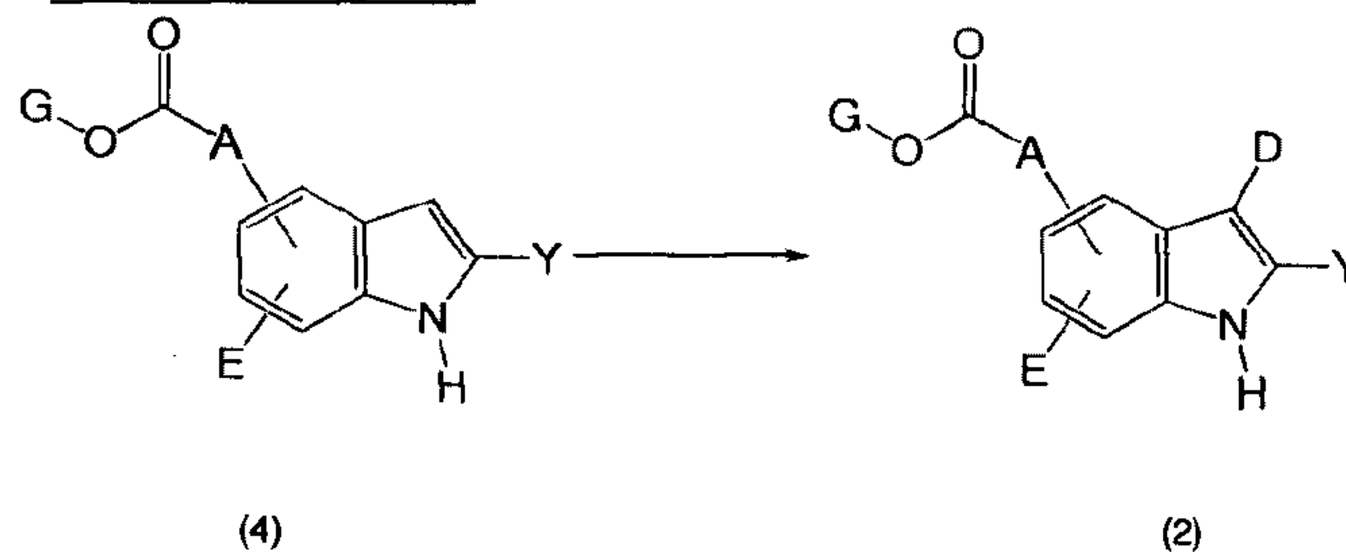
Reaction Scheme 2
