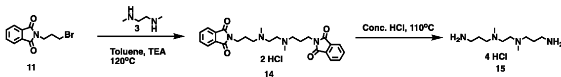
Scheme 14: Synthesis of Amine Compound 15
