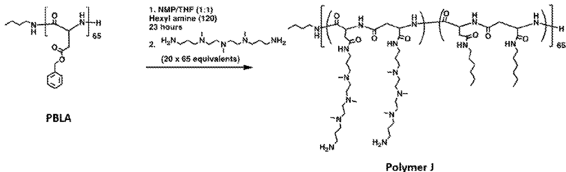
Scheme 17: Synthesis of Polymer J
