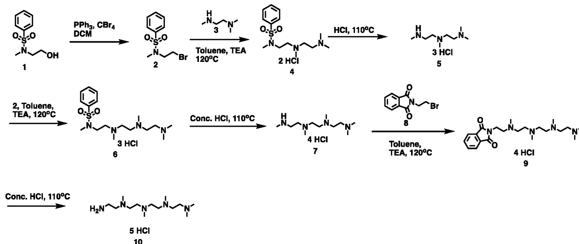
Scheme 5: Synthesis of Amine Compound 10
