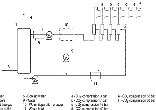
LOW TEMPERATURE CAPTURE PROCESS A
