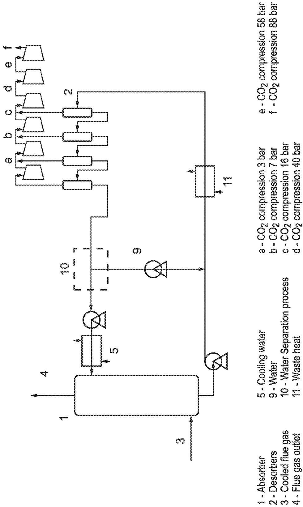
LOW TEMPERATURE CAPTURE PROCESS A
