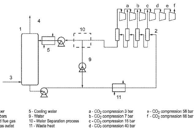
LOW TEMPERATURE CAPTURE PROCESS A
